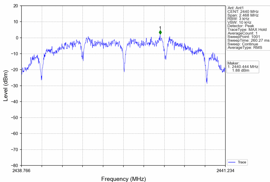
Zigbee_MCH_2440MHz_Ant1_NTNV
