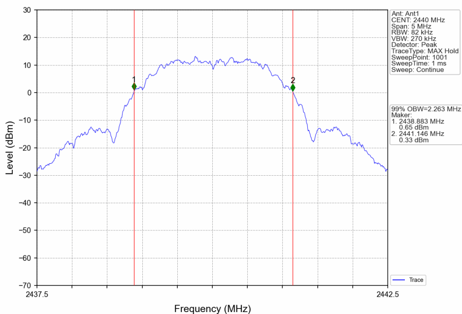
Zigbee_MCH_2440MHz_Ant1_NTNV
