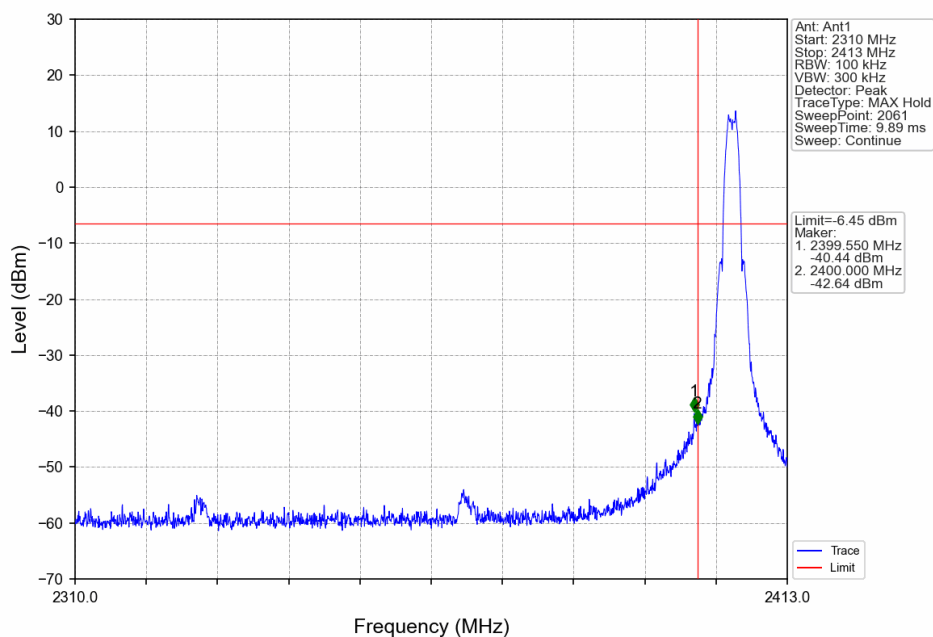
Zigbee_LCH_2405MHz_Ant1_NTNV
