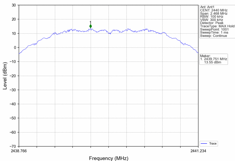
Zigbee_MCH_2440MHz_Ant1_NTNV
