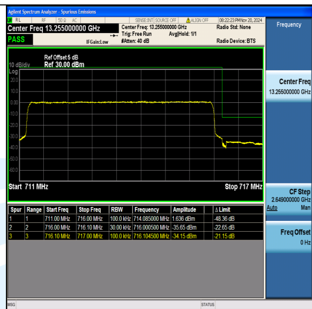
Band12 5MHz 16QAM 23155 25RB#0
