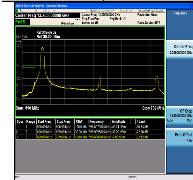
Band12 10MHz 16QAM 23060 1RB#0
