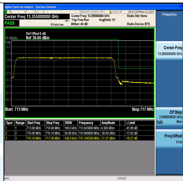
Band12 3MHz 64QAM 23165 15RB#0
