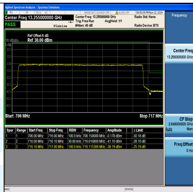
Band12 10MHz 64QAM 23130 50RB#0
