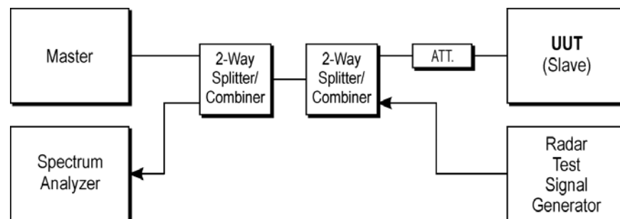
Figure 1: Setup
