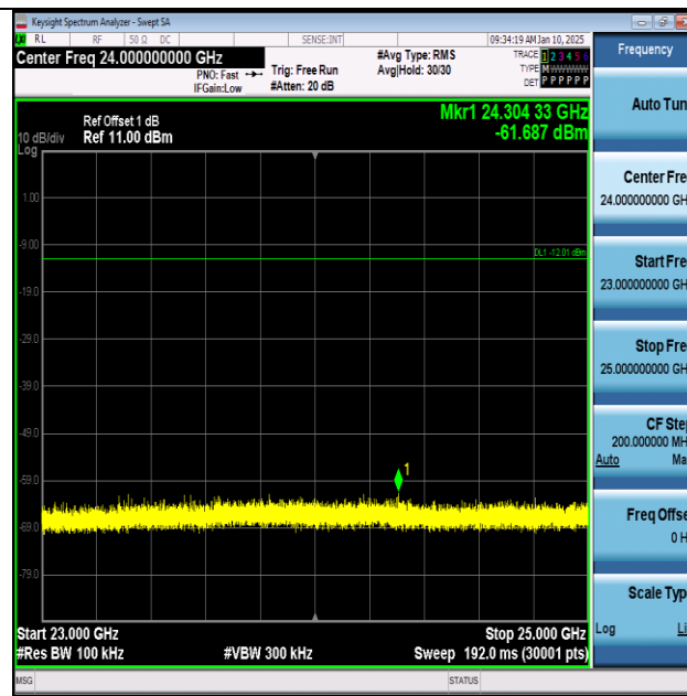
BLE_125K-Ant1-2402-23000~25000-PASS
