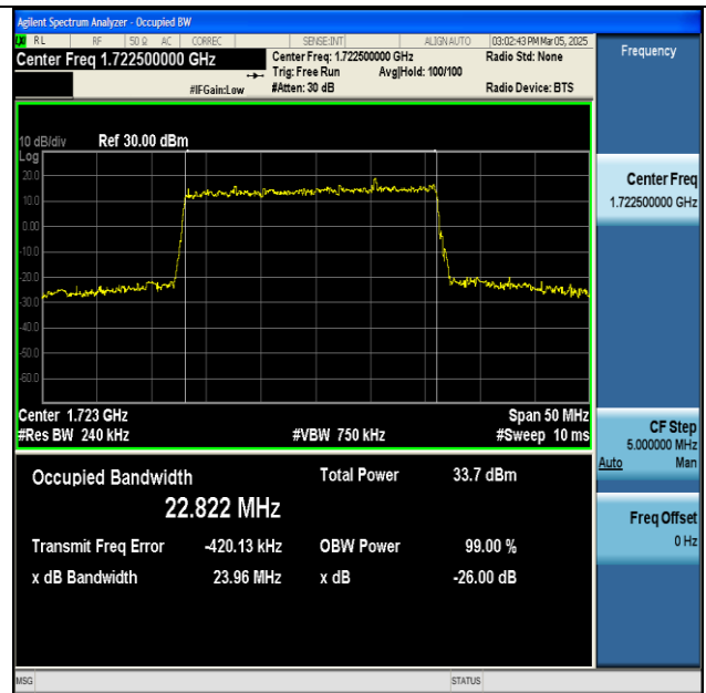
NTNV-n66-PC3-15-25-L-DFT-QPSK-Outer_Full-Ant1- PASS
