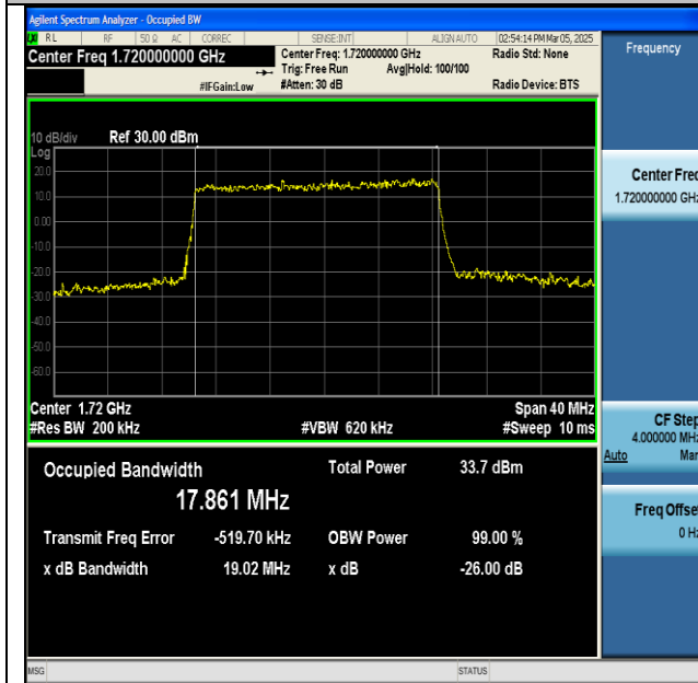
NTNV-n66-PC3-15-20-L-DFT-QPSK-Outer_Full-Ant1- PASS
