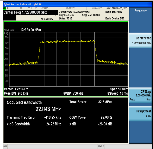
NTNV-n66-PC3-15-25-L-DFT-64QAM-Outer_Full-Ant1- PASS
