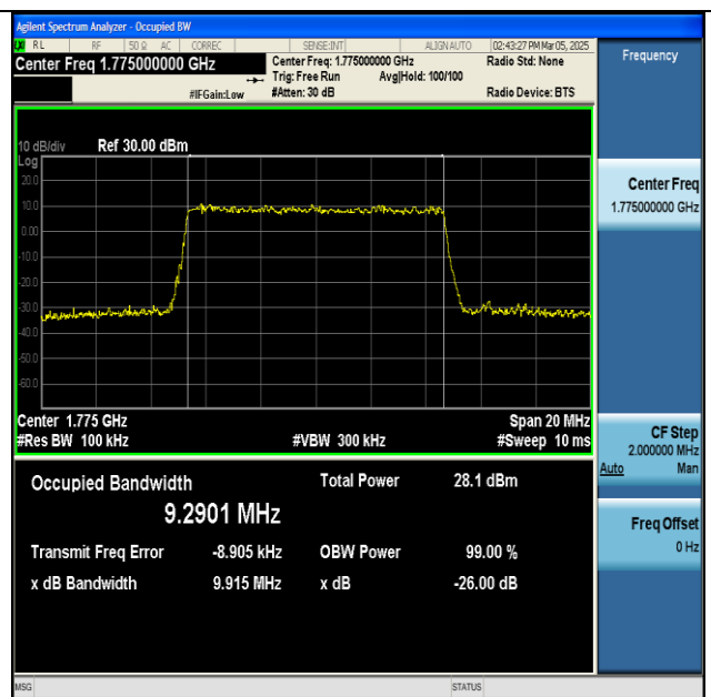
NTNV-n66-PC3-15-10-H-CP-256QAM-Outer_Full-Ant1- PASS
