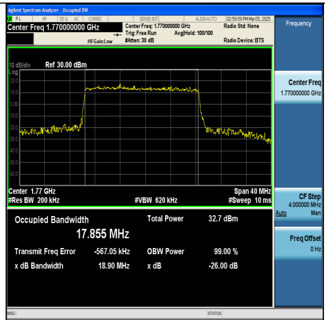
NTNV-n66-PC3-15-20-H-DFT-16QAM-Outer_Full-Ant1- PASS
