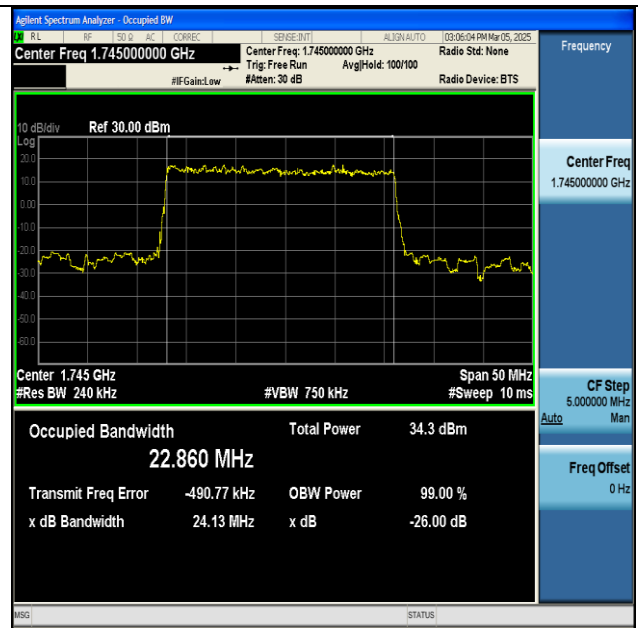
NTNV-n66-PC3-15-25-M-DFT-BPSK-Outer_Full-Ant1- PASS
