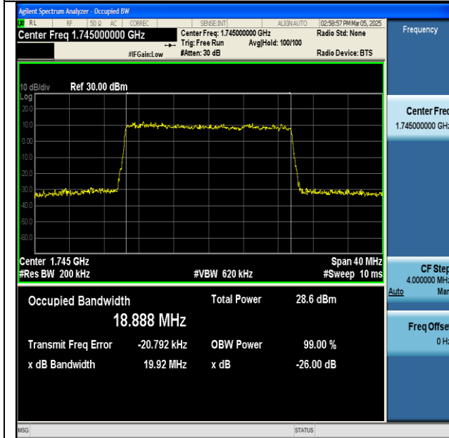
NTNV-n66-PC3-15-20-M-CP-256QAM-Outer_Full-Ant1- PASS
