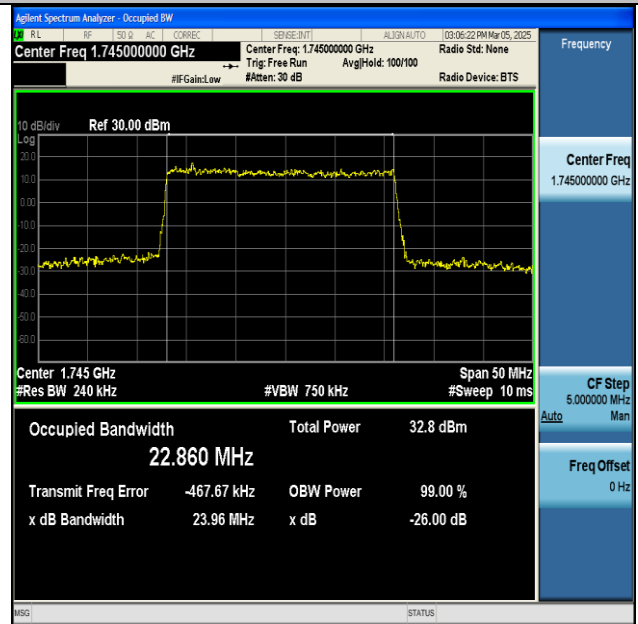
NTNV-n66-PC3-15-25-M-DFT-16QAM-Outer_Full-Ant1- PASS
