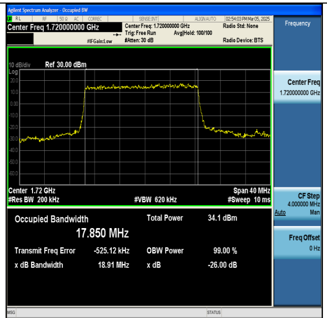
NTNV-n66-PC3-15-20-L-DFT-BPSK-Outer_Full-Ant1- PASS
