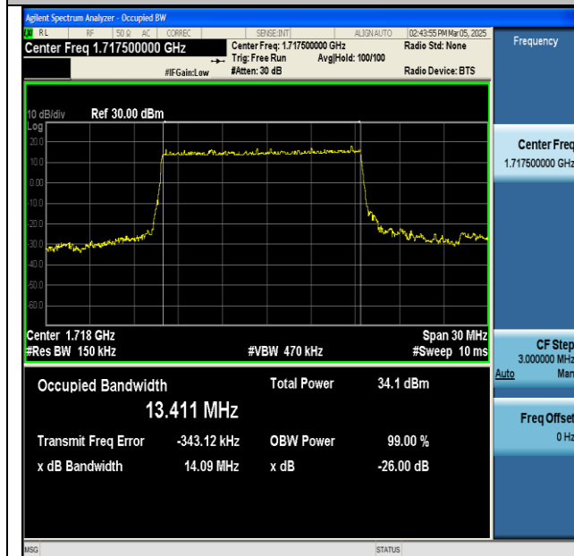
NTNV-n66-PC3-15-15-L-DFT-BPSK-Outer_Full-Ant1- PASS
