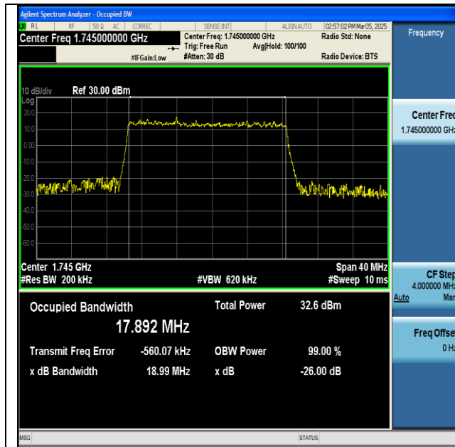
NTNV-n66-PC3-15-20-M-DFT-16QAM-Outer_Full-Ant1- PASS
