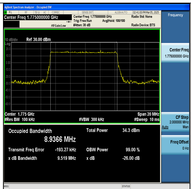
NTNV-n66-PC3-15-10-H-DFT-BPSK-Outer_Full-Ant1- PASS
