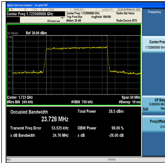
NTNV-n66-PC3-15-25-L-CP-256QAM-Outer_Full-Ant1- PASS
