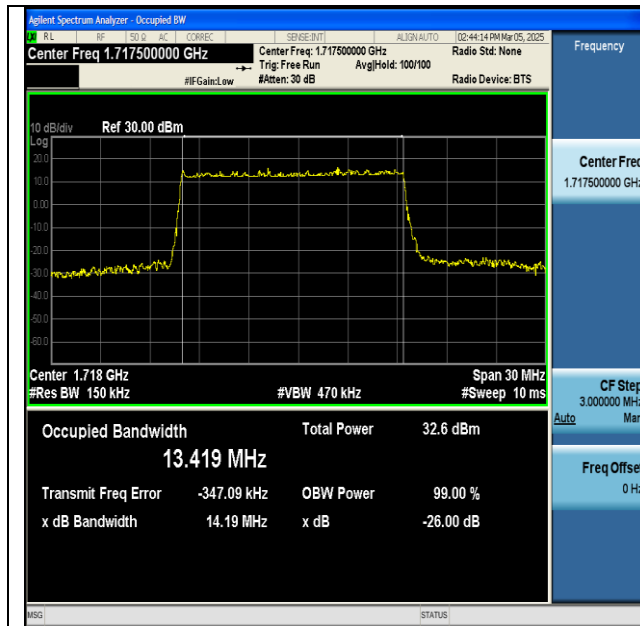
NTNV-n66-PC3-15-15-L-DFT-16QAM-Outer_Full-Ant1- PASS
