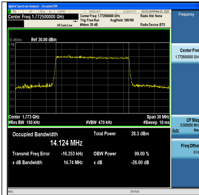
NTNV-n66-PC3-15-15-H-CP-256QAM-Outer_Full-Ant1- PASS
