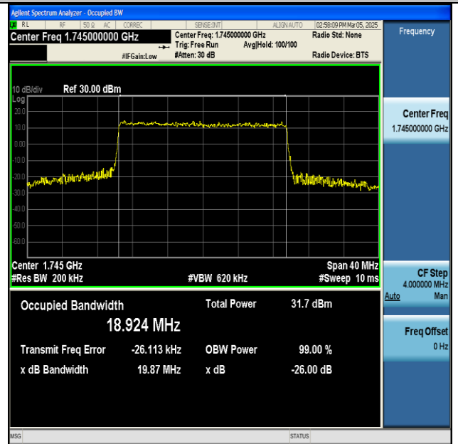
NTNV-n66-PC3-15-20-M-CP-QPSK-Outer_Full-Ant1-PASS
