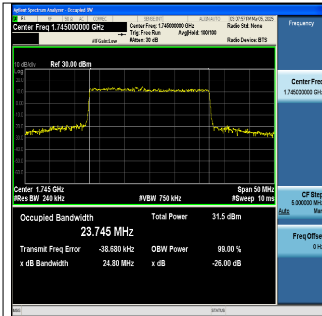
NTNV-n66-PC3-15-25-M-CP-64QAM-Outer_Full-Ant1- PASS
