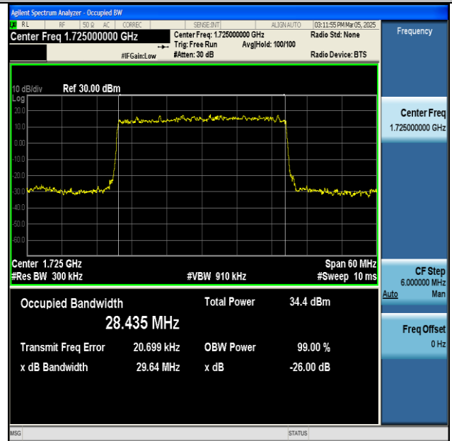
NTNV-n66-PC3-15-30-L-DFT-BPSK-Outer_Full-Ant1- PASS
