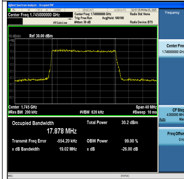
NTNV-n66-PC3-15-20-M-DFT-256QAM-Outer_Full-Ant1- PASS
