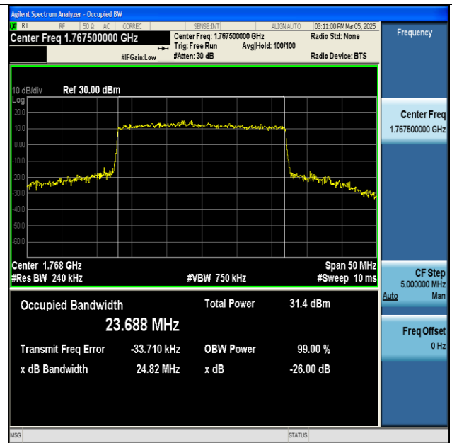
NTNV-n66-PC3-15-25-H-CP-64QAM-Outer_Full-Ant1- PASS
