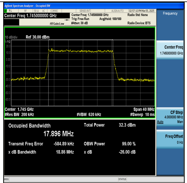
NTNV-n66-PC3-15-20-M-DFT-64QAM-Outer_Full-Ant1- PASS
