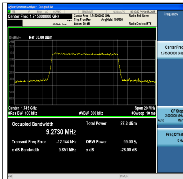
NTNV-n66-PC3-15-10-M-CP-256QAM-Outer_Full-Ant1- PASS
