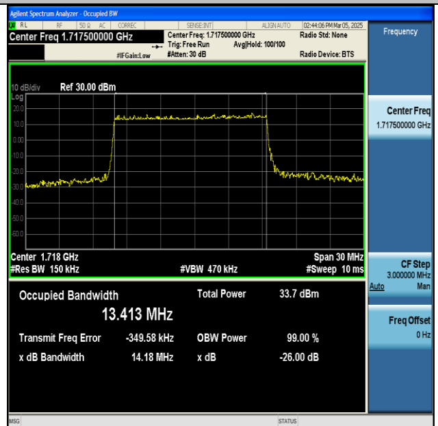
NTNV-n66-PC3-15-15-L-DFT-QPSK-Outer_Full-Ant1- PASS
