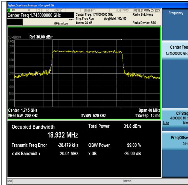
NTNV-n66-PC3-15-20-M-CP-16QAM-Outer_Full-Ant1- PASS
