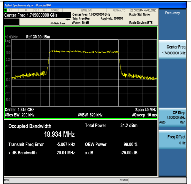
NTNV-n66-PC3-15-20-M-CP-64QAM-Outer_Full-Ant1- PASS
