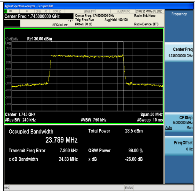
NTNV-n66-PC3-15-25-M-CP-256QAM-Outer_Full-Ant1- PASS
