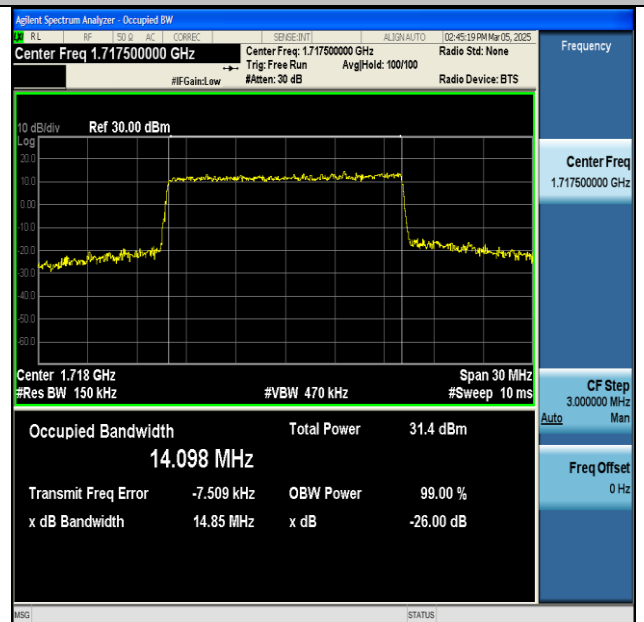
NTNV-n66-PC3-15-15-L-CP-QPSK-Outer_Full-Ant1-PASS
