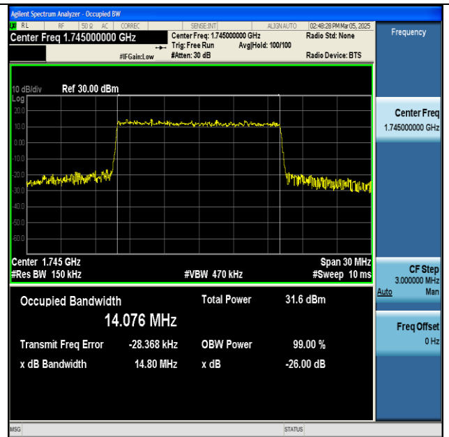
NTNV-n66-PC3-15-15-M-CP-16QAM-Outet_Full-Ant1-PASS
