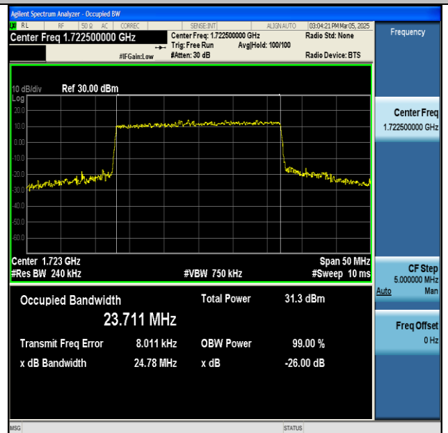
NTNV-n66-PC3-15-25-L-CP-64QAM-Outer_Full-Ant1-PASS
