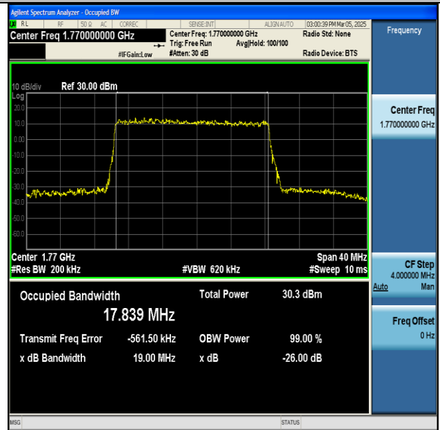
NTNV-n66-PC3-15-20-H-DFT-256QAM-Outer_Full-Ant1- PASS
