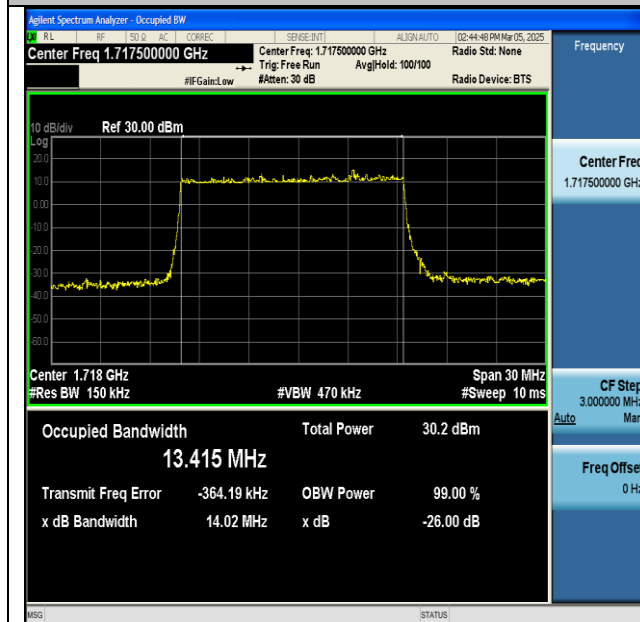
NTNV-n66-PC3-15-15-L-DFT-256QAM-Outer_Full-Ant1- PASS
