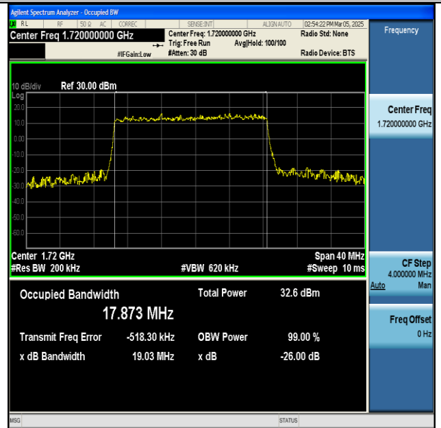
NTNV-n66-PC3-15-20-L-DFT-16QAM-Outer_Full-Ant1- PASS
