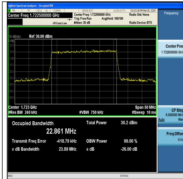
NTNV-n66-PC3-15-25-L-DFT-256QAM-Outer_Full-Ant1-PASS
