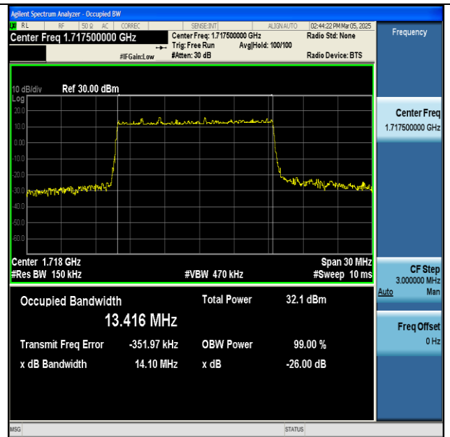
NTNV-n66-PC3-15-15-L-DFT-64QAM-Outer_Full-Ant1- PASS
