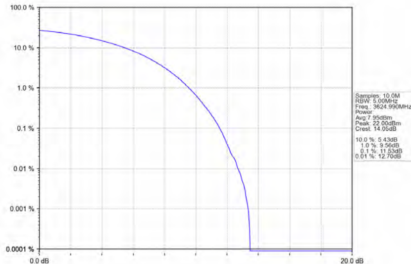
n48_30kHz_MIMO_NTNV_40MHz_CP-OFDM_QPSK_3624.99MHz_Outer_Full
