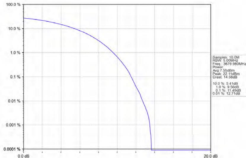
n48_30kHz_MIMO_NTNV_40MHz_CP-OFDM_QPSK_3679.98MHz_Outer_Full
