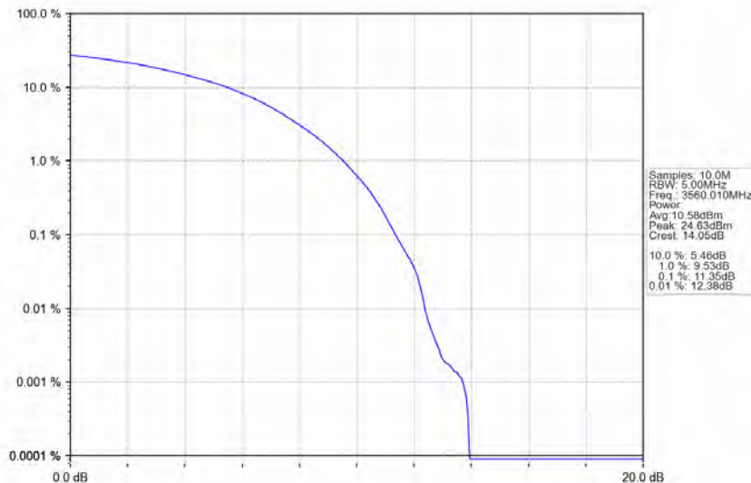
n48_30kHz_MIMO_NTNV_20MHz_CP-OFDM 64 QAM 3560.01MHz_Outer_Full
