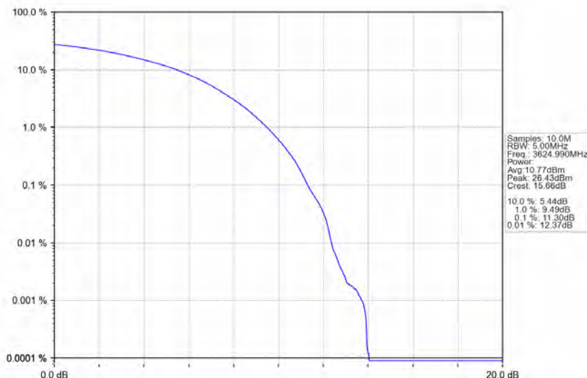
n48_30kHz_MIMO_NTNV_20MHz_CP-OFDM 64 QAM 3624.99MHz_Outer_Full
