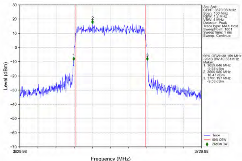
n48_30kHz_MIMO_NTNV_40MHz_CP-OFDM_64_QAM_3679.98MHz_Outer_Full
