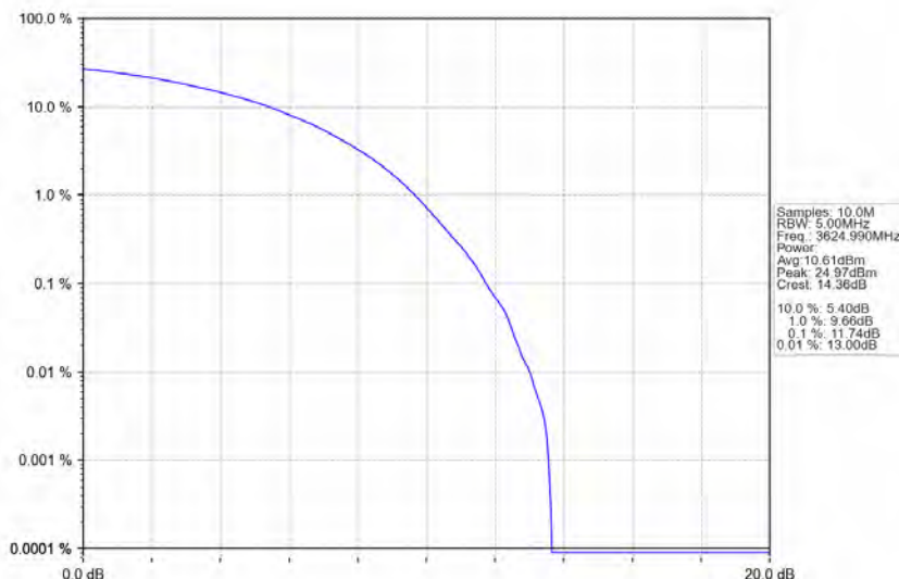
n48_30kHz_MIMO_NTNV_10MHz_CP-OFDM_256_QAM_3624.99MHz_Outer_Full
