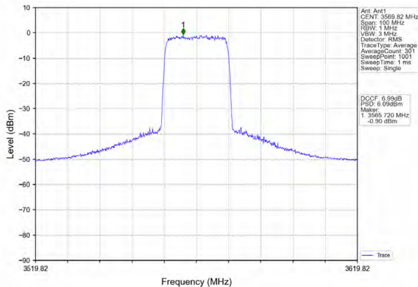
n48_30kHz_MIMO_NTNV_40MHz_CP-OFDM_256_QAM_3570MHz_Inner_Full
