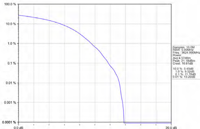
n48_30kHz_MIMO_NTNV_40MHz_CP-OFDM_256_QAM_3624.99MHz_Outer_Full
