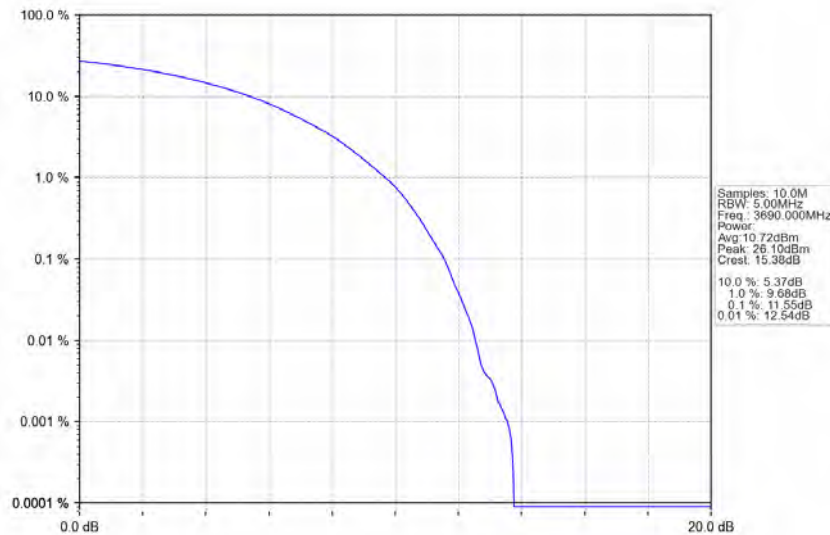
n48_30kHz_MIMO_NTNV_20MHz_CP-OFDM_QPSK_3690MHz_Outer_Full
