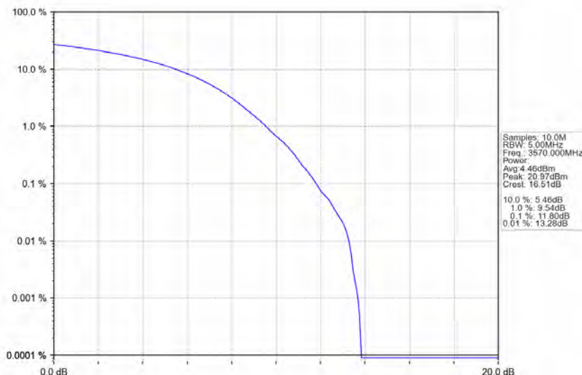
n48_30kHz_MIMO_NTNV_40MHz_CP-OFDM_256_QAM_3570MHz_Outer_Full
