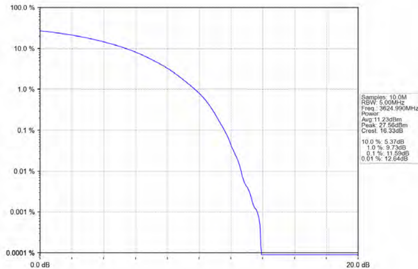
n48_30kHz_MIMO_NTNV_20MHz_CP-OFDM_QPSK_3624.99MHz_Outer_Full
