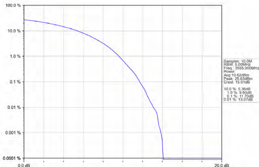
n48_30kHz_MIMO_NTNV_10MHz_CP-OFDM_256_QAM_3555MHz_Outer_Full
