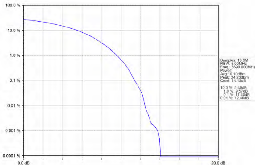
n48_30kHz_MIMO_NTNV_20MHz_CP-OFDM 64 QAM 3690MHz_Outer_Full
