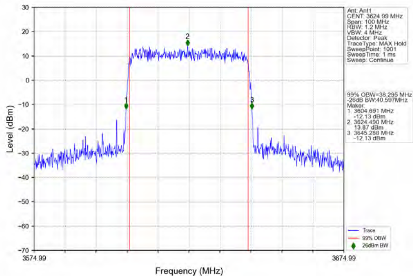
n48_30kHz_MIMO_NTNV_40MHz_CP-OFDM_256_QAM_3624.99MHz_Outer_Full
