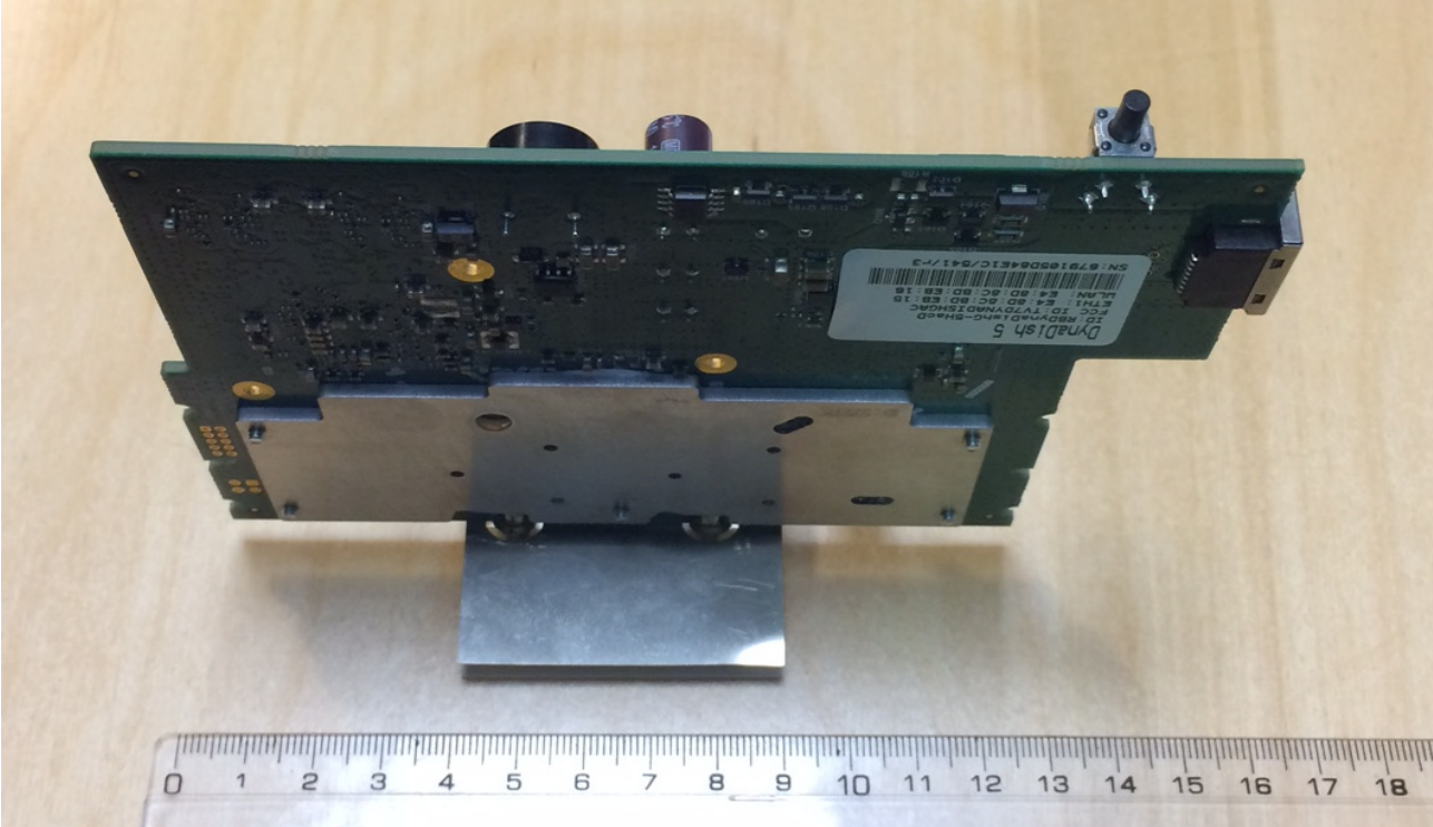
Internal Photos of EUT
