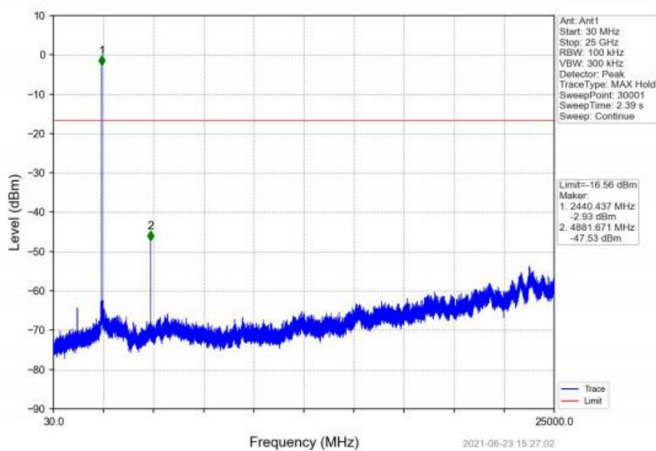
\pi /4-DQPSK_2DH5_MCH_2441MHz_Ant1_NTNV
