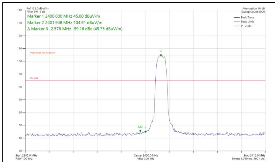
Figure 159 - Bluetooth 3-DH5, SISO, Core 1 - 2402 MHz Band Edge Frequency 2400 MHz
