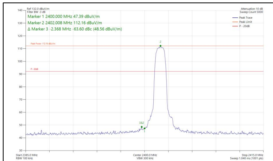
Figure 164 - Bluetooth 2-DH5, MIMO, Core 0 - Core 1 - 2402 MHz Band Edge Frequency 2400 MHz
