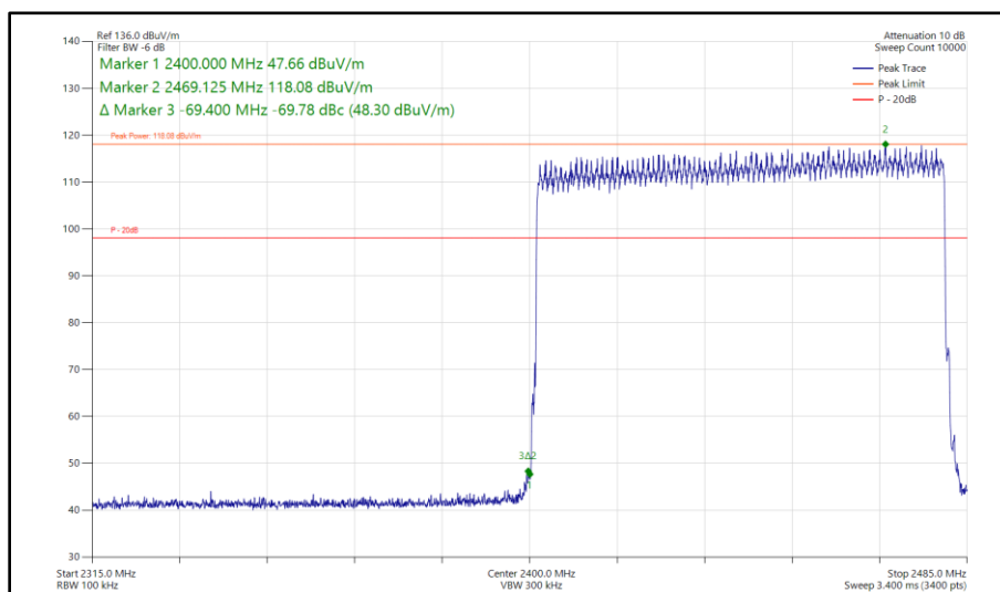
Figure 175 - Bluetooth 2-DH5, SISO, Core 1 - Hopping Band Edge Frequency 2400 MHz
