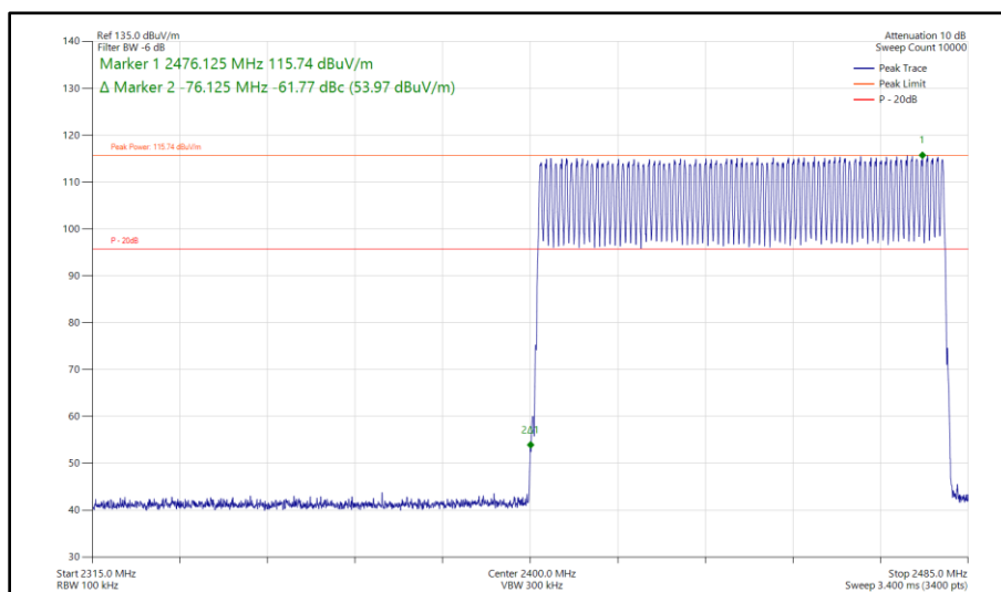
Figure 166 - Bluetooth DH5, MIMO, Core 0 - Core 1 - Hopping Band Edge Frequency 2400 MHz
