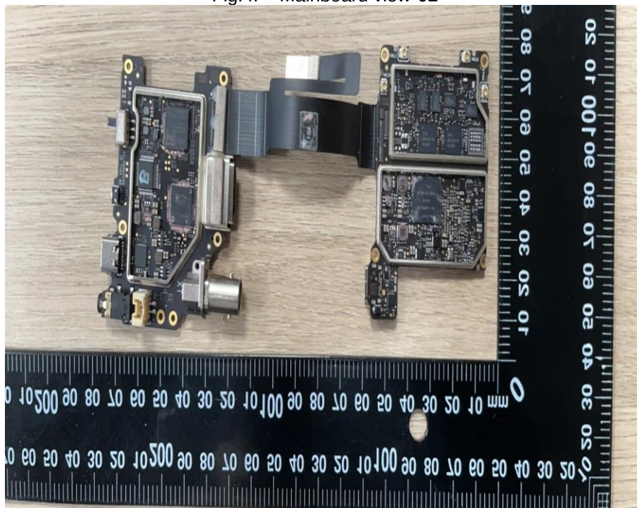
Fig.5. Mainboard view-02
