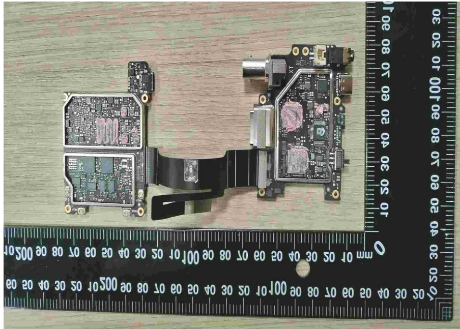
Fig.4. Mainboard view-02
