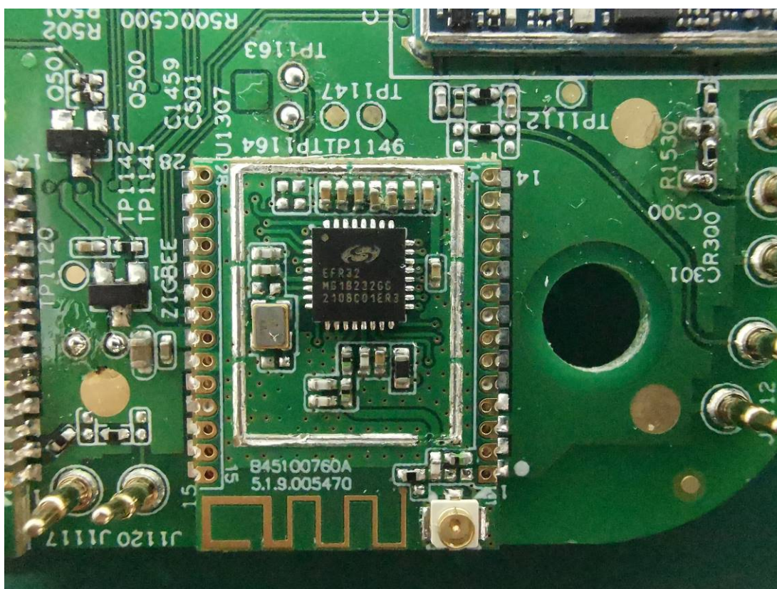
ZigBee Antenna
