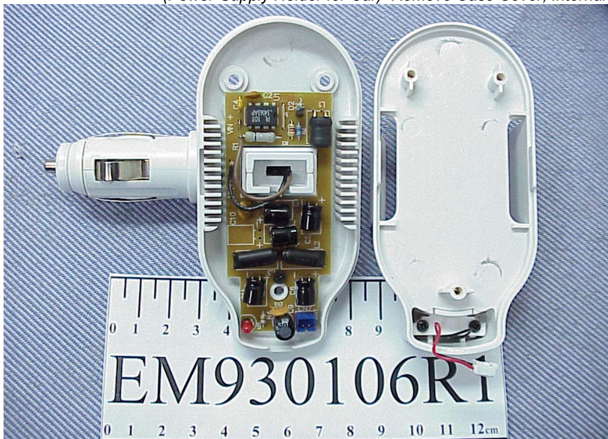
Photos 15 (Power-Supply Holder for Car) Remove Case Cover, Internal View
