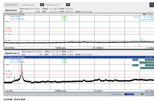
Figure 8.8-35: Conducted spurious emissions 30 MHz – 40 GHz, mid channel, 802.11n
