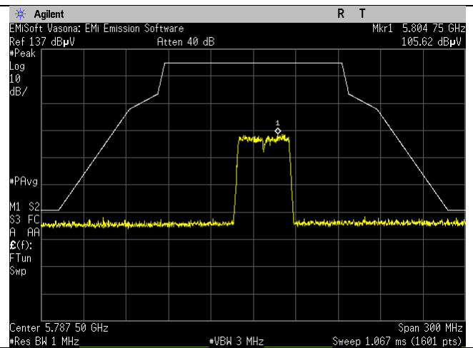
5795 MHz_n40
