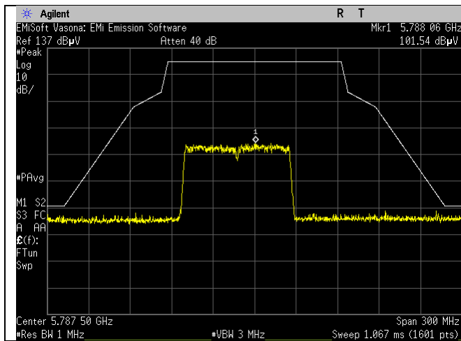
5775MHz_ac80mode
