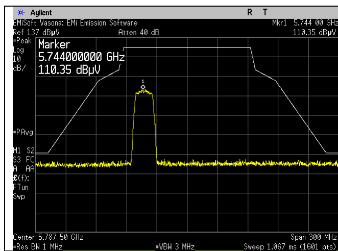
5745MHz_n20mode
