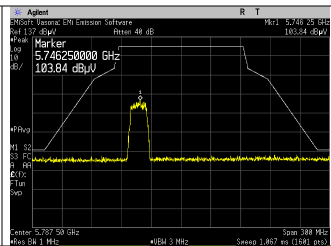
5745MHz_amode
