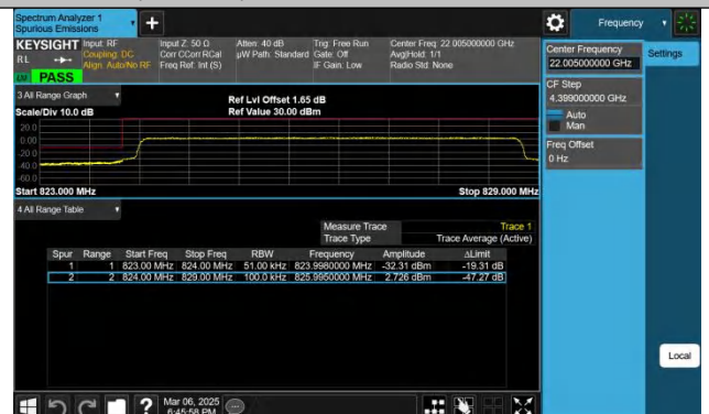
Band26(824-849)-5MHz-QPSK-26815-25RB#0-PASS
