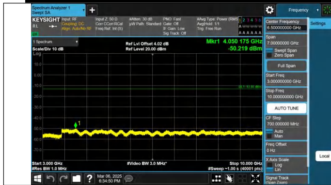
Band26(824-849)-1.4MHz-QPSK-26915-1RB#0-3000~10000-PASS S
