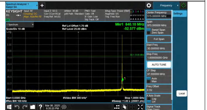
Band26(824-849)-1.4MHz-QPSK-26915-1RB#5-30~1000-PASS
