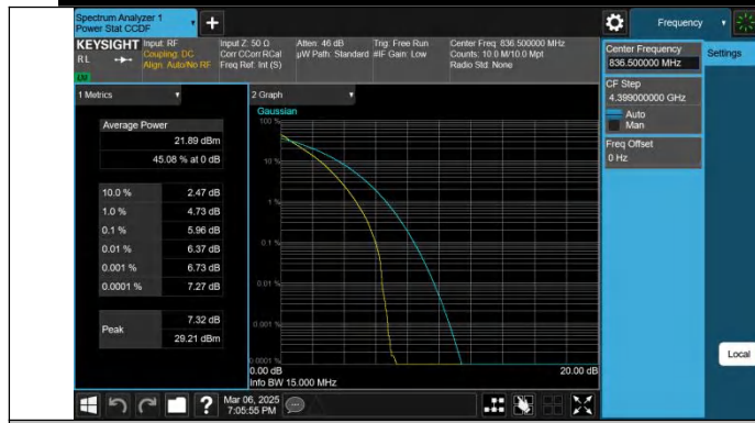
Band26(824-849)-15MHz-QPSK-26915-75RB#0-PASS
