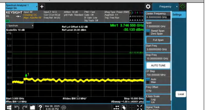
Band26(824-849)-1.4MHz-QPSK-26915-1RB#5-3000~10000-PASS S
