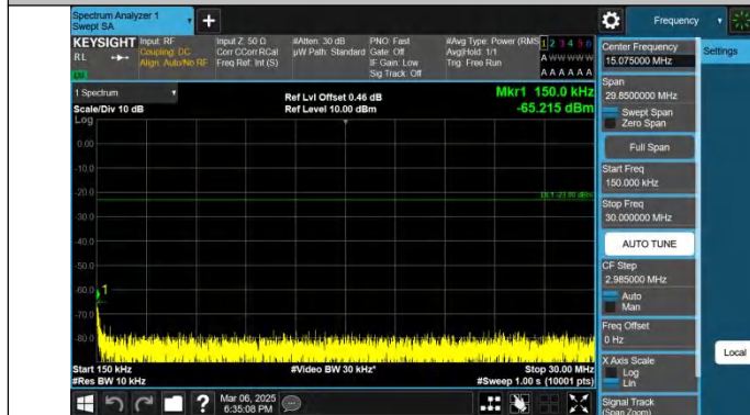
Band26(824-849)-1.4MHz-QPSK-26915-1RB#5-0.15~30-PASS
