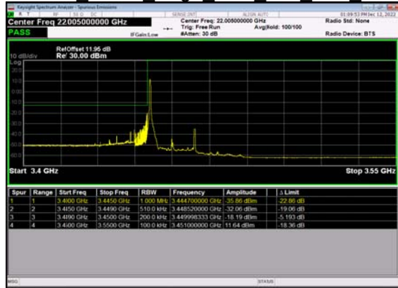
N77(20M)_DFT-s- OFDM BPSK Edge 1RB Left Low CH
