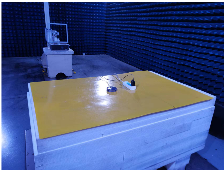
Photo of Radiated Emission Measurement (9kHz-30MHz)
