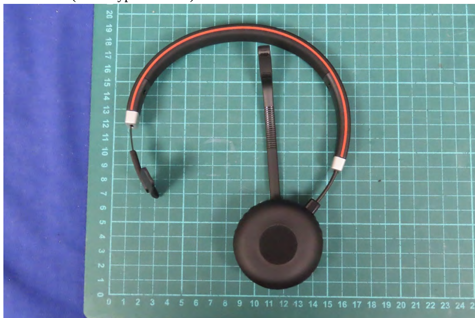
(10) EUT Photo (Mono type headsets)
