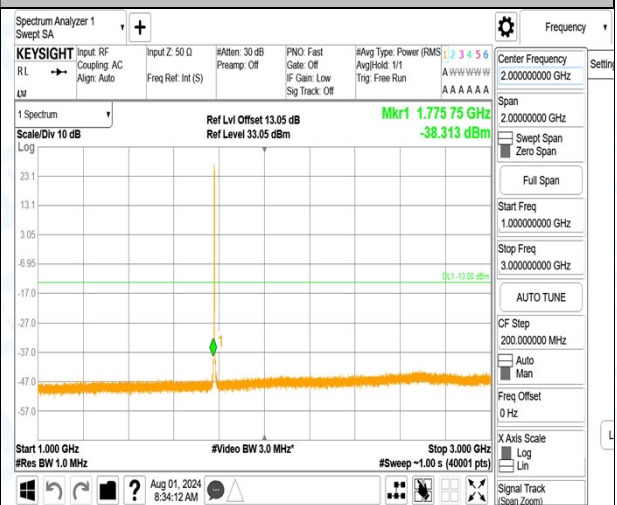
Band66_1.4MHz_QPSK_132665_1RB#0_1000~3000_1000~3000
