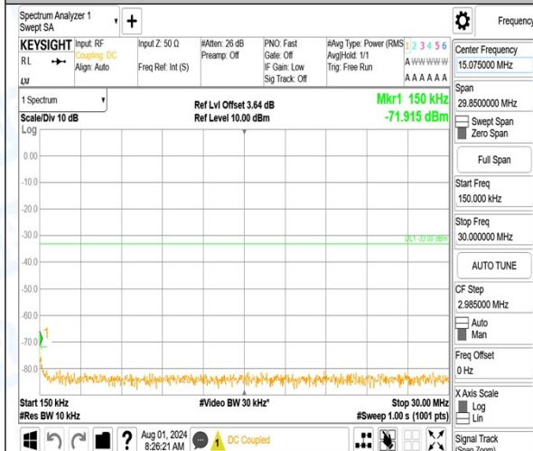
Band66_1.4MHz_QPSK_132322_1RB#0_0.15~30_0.15~30
