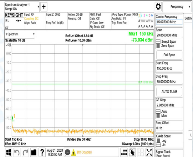
Band66_1.4MHz_QPSK_131979_6RB#0_1000~3000_1000~3000
