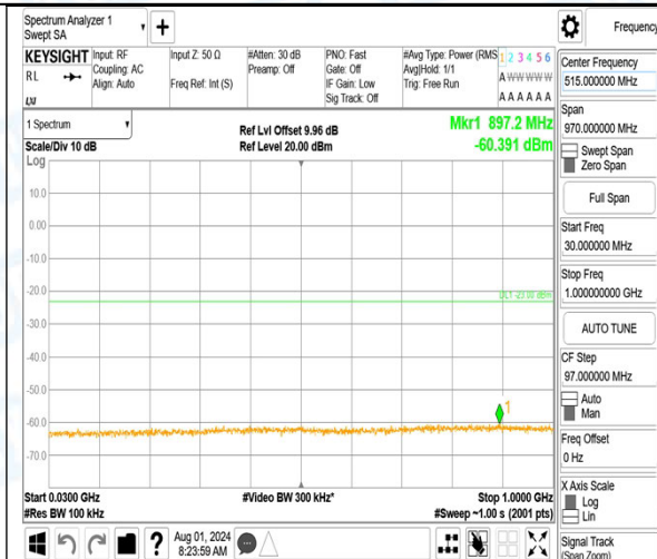
Band66_1.4MHz_QPSK_131979_6RB#0_3000~20000_3000~2000
