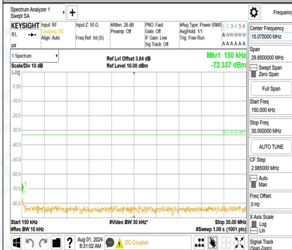
Band66_1.4MHz_QPSK_132322_6RB#0_0.15~30_0.15~30
