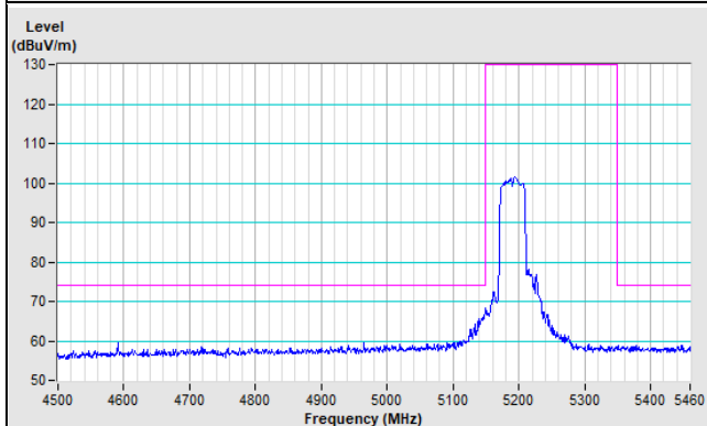
Horizontal (Peak)
