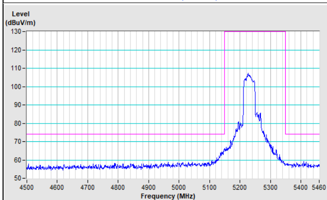
Vertical (Peak)
