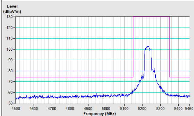
Horizontal (Peak)
