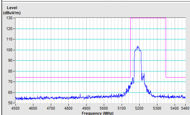
Vertical (Peak)
