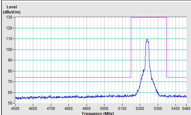
Vertical (Peak)
