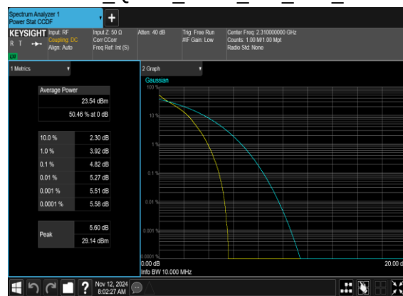
N30(10M)_DFT-s- OFDM_QPSK_Outer_Full_Low_CH
