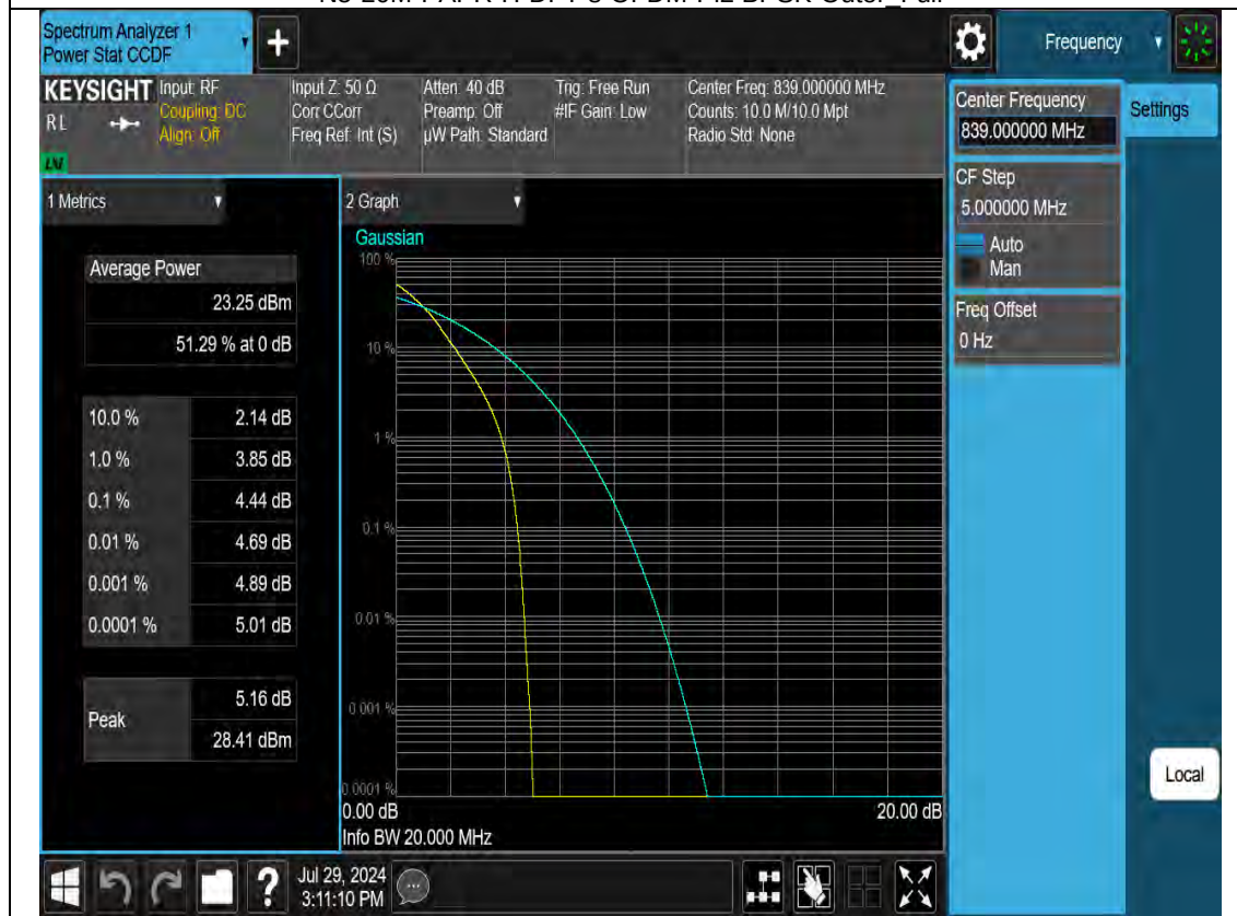
N5-20M-PAPR-H-CP-OFDM-QPSK-Outer Full
