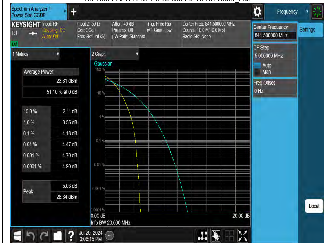
N5-15M-PAPR-H-CP-OFDM-QPSK-Outer Full
