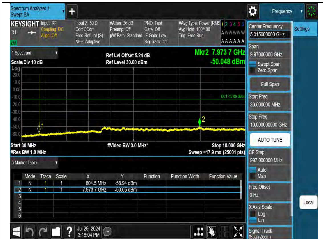
N5-10M-CSE-L-DFT-s-OFDM-Pi2 BPSK-1RB0-30MHz-10GHz
