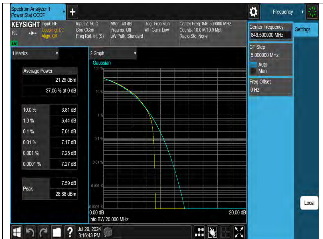
N5-10M-PAPR-L-DFT-s-OFDM-Pi2 BPSK-Outter Full
