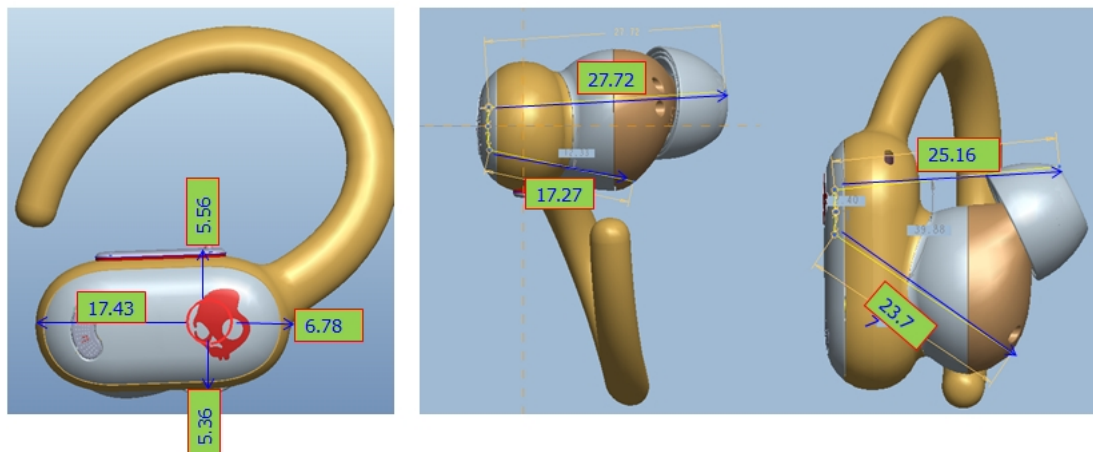
Antenna location
