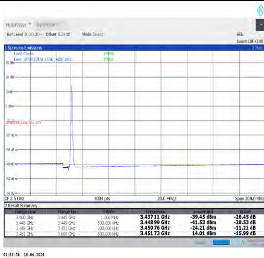
1-N78-3450-3550-30-25-L-1-DFT-PI2BPSK-Edge_1RB _Left-1@0-Ant1-1--PASS-see graph
