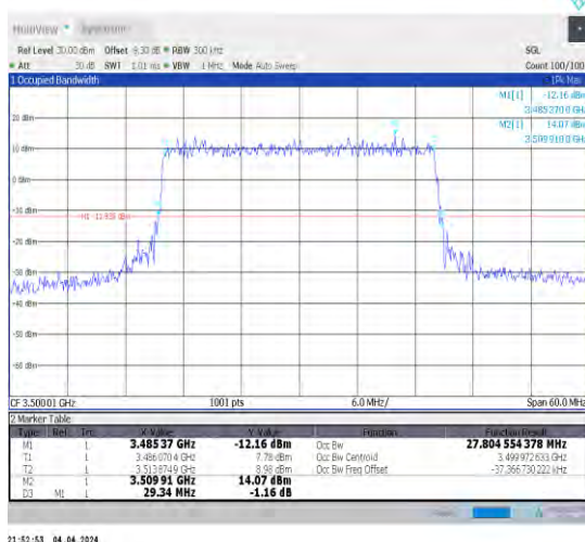
1-N78-3450-3550-30-30-M-7-CP-16QAM-Outer_Full-78@0-Ant1-27.806-29.340-≤30-PASS
