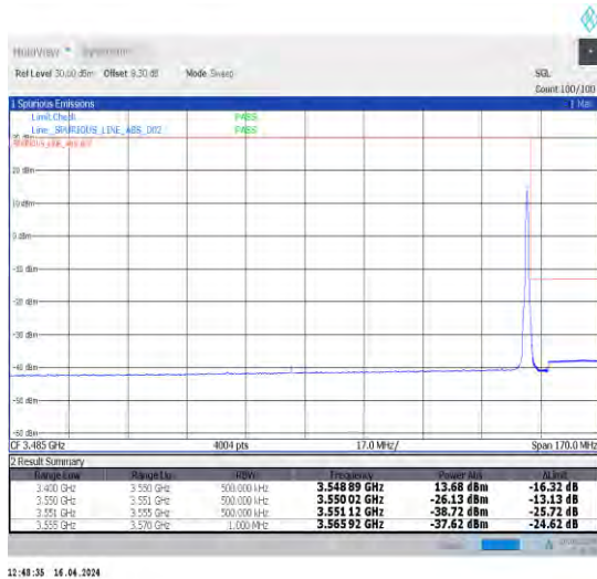
1-N78-3450-3550-30-70-H-5-CP-QPSK-Edge_1RB_Ri ght-1@188-Ant1-1--PASS-see graph
