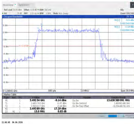
1-N78-3450-3550-30-15-M-8-CP-64QAM-Outer_Full-38@0-Ant1-13.638-15.000-≤15-PASS
