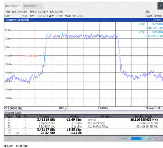
1-N78-3450-3550-30-30-M-2-DFT-PI2BPSK-Outet_Full-75@0-Ant1-26.822-28.320-≤30-PASS
