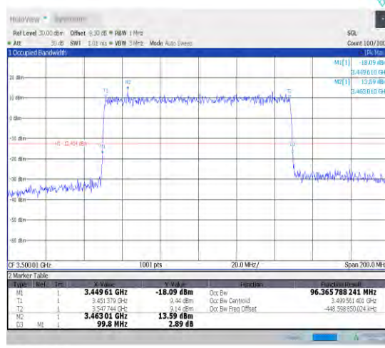
1-N78-3450-3550-30-100-M-5-DFT-256QAM-Outter_Full-270@0-Ant1-96.366-99.800-≤100-PASS
