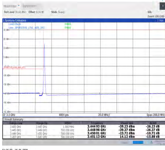
1-N78-3450-3550-30-70-L-1-DFT-PI2BPSK-Edge_1RB _Left-1@0-Ant1-1--PASS-see graph
