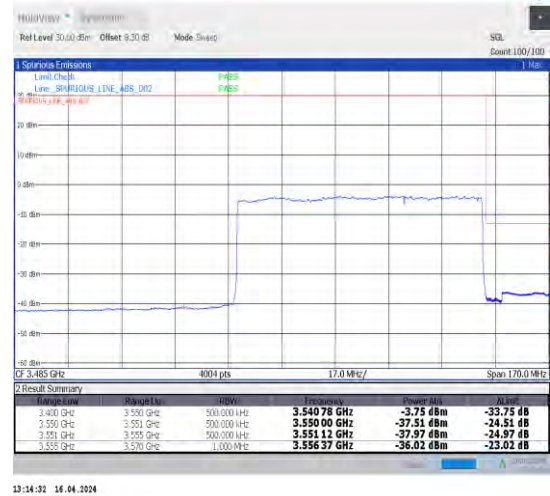
1-N78-3450-3550-30-80-H-3-DFT-PI2BPSK-Outer _Full-216@0-Ant1-1--PASS-see graph
