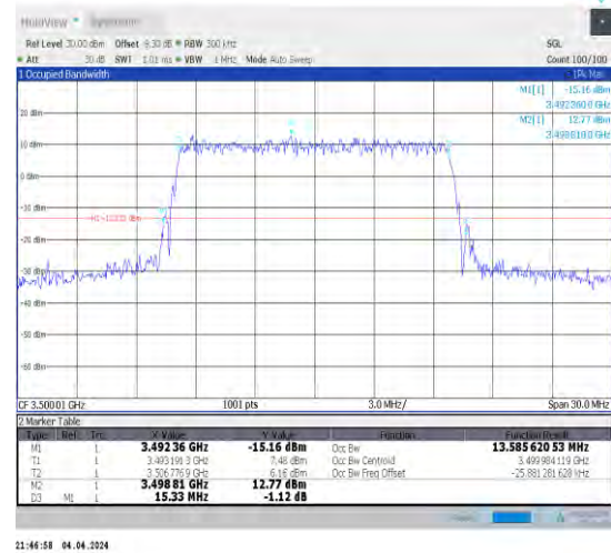
1-N78-3450-3550-30-15-M-9-CP-256QAM-Outer_Fu II-38@0-Ant1-13.586-15.330-≤15-PASS
