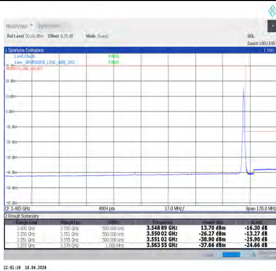
1-N78-3450-3550-30-70-H-2-DFT-PI2BPSK-Edge_1R B_Right-1@188-Ant1-1--PASS-see graph
