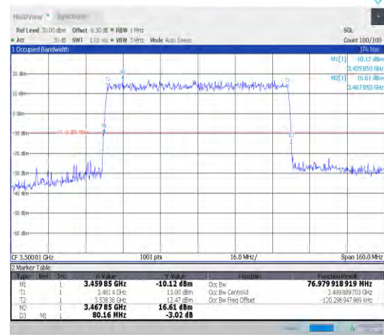
1-N78-3450-3550-30-80-M-1-DFT-QPSK-Outer_Full-216@0-Ant1-76.98-80.160-≤80-PASS
