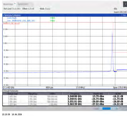
1-N78-3450-3550-30-80-H-2-DFT-PI2BPSK-Edge_1R B_Right-1@216-Ant1-1--PASS-see graph
