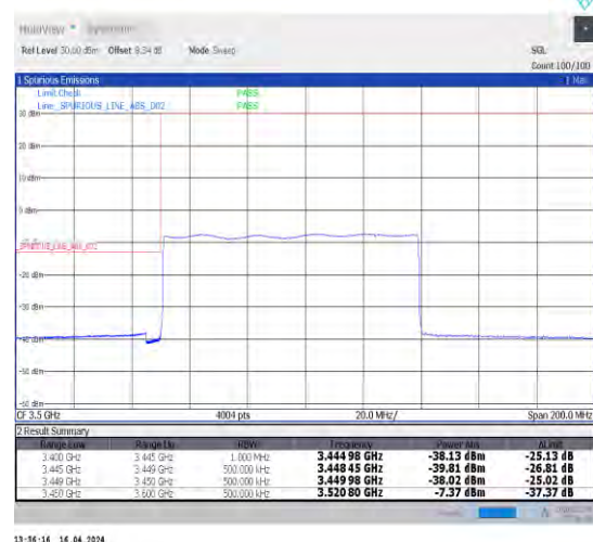
1-N78-3450-3550-30-90-L-6-CP-QPSK-Outer_Full -245@0-Ant1-1--PASS-see graph
