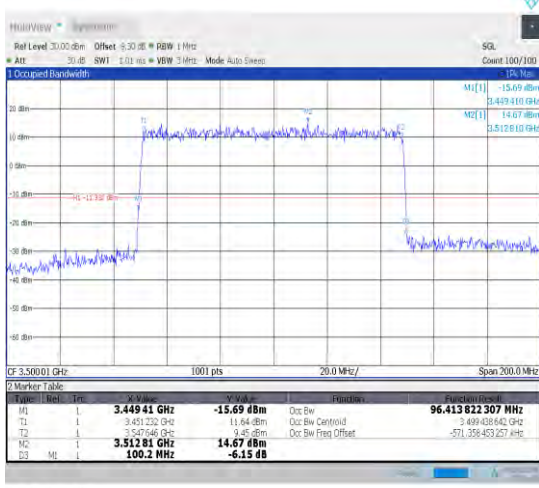
1-N78-3450-3550-30-100-M-4-DFT-64QAM-Outter_Full-270@0-Ant1-96.414-100.200-≤100-PASS
