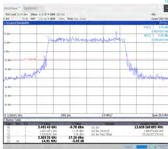
1-N78-3450-3550-30-15-M-7-CP-16QAM-Out_Full-38@0-Ant1-13.659-14.910-≤15-PASS
