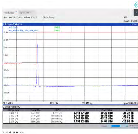
1-N78-3450-3550-30-30-L-4-CP-QPSK-Edge_1RB_Lef t-1@0-Ant1-1--PASS-see graph
