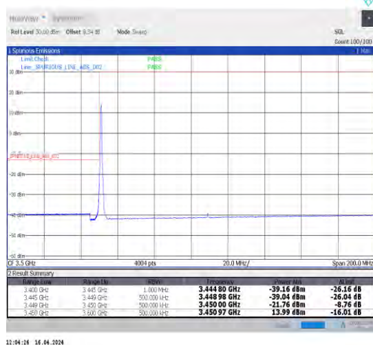
1-N78-3450-3550-30-60-L-4-CP-QPSK-Edge_1RB_Lef t-1@0-Ant1-1--PASS-see graph
