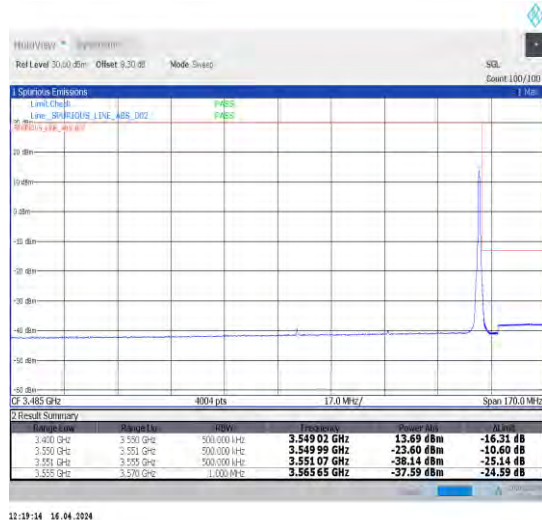
1-N78-3450-3550-30-60-H-5-CP-QPSK-Edge_1RB_Ri ght-1@161-Ant1-1--PASS-see graph
