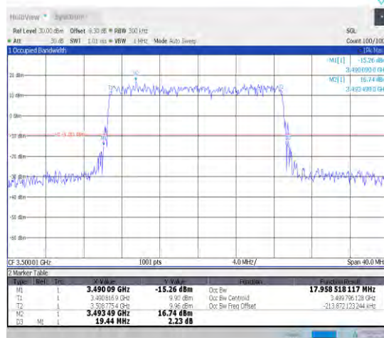
1-N78-3450-3550-30-20-M-4-DFT-64QAM-Outer_Ful I-50@0-Ant1-17.959-19.440-≤20-PASS
