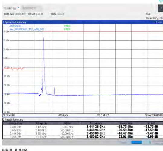
1-N78-3450-3550-30-15-L-4-CP-QPSK-Edge_1RB_Lef t-1@0-Ant1-1--PASS-see graph
