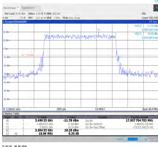
1-N78-3450-3550-30-20-M-1-DFT-QPSK-Outer_Full-50@0-Ant1-17.958-18.960-≤20-PASS
