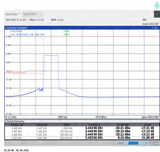
1-N78-3450-3550-30-20-L-6-CP-QPSK-Outer_Full -51@0-Ant1-1--PASS-see graph
