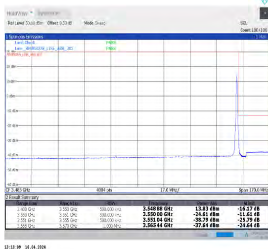
1-N78-3450-3550-30-80-H-5-CP-QPSK-Edge_1RB_Ri ght-1@216-Ant1-1--PASS-see graph
