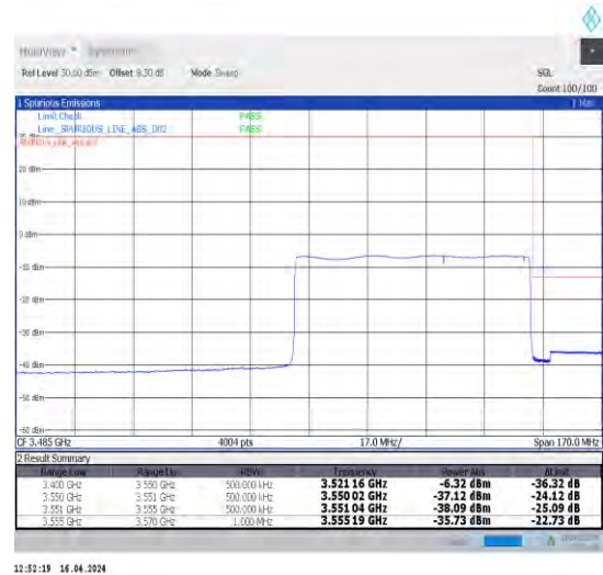
1-N78-3450-3550-30-70-H-6-CP-QPSK-Outer_Full -189@0-Ant1-1--PASS-see graph
