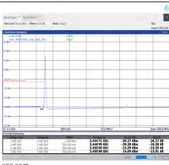
1-N78-3450-3550-30-100-L-1-DFT-PI2BPSK-Edge_1R_B_Left-1@0-Ant1-1--PASS-see graph
