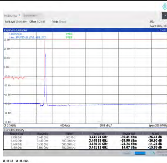
1-N78-3450-3550-30-30-L-1-DFT-PI2BPSK-Edge_1RB _Left-1@0-Ant1-1--PASS-see graph
