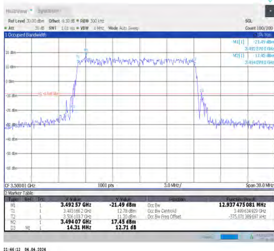
1-N78-3450-3550-30-15-M-4-DFT-64QAM-Out_Ful I-36@0-Ant1-12.937-14.310-≤15-PASS
