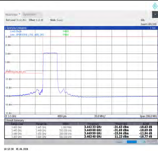
1-N78-3450-3550-30-20-L-3-DFT-PI2BPSK-Outer _Full-50@0-Ant1-1--PASS-see graph
