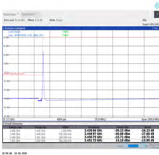
1-N78-3450-3550-30-25-L-4-CP-QPSK-Edge_1RB_Lef t-1@0-Ant1-1--PASS-see graph
