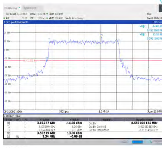
1-N78-3450-3550-30-10-M-8-CP-64QAM-Outer_F ull-24@0-Ant1-8.569-9.340-≤10-PASS
