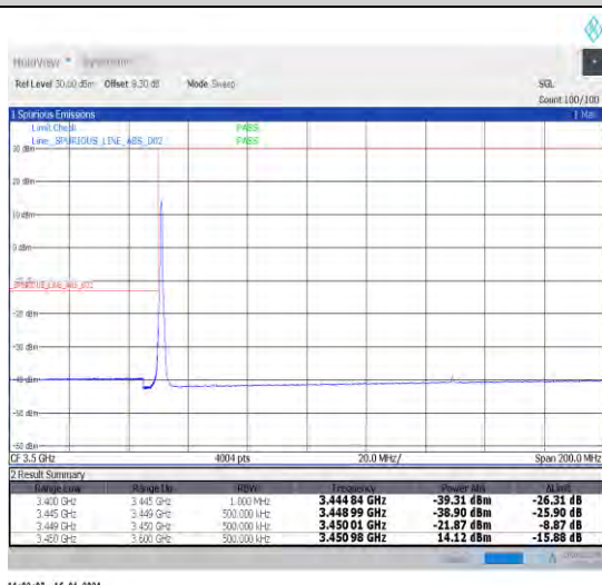
1-N78-3450-3550-30-100-L-4-CP-QPSK-Edge_1RB_Left-1@0-Ant1-1--PASS-see graph
