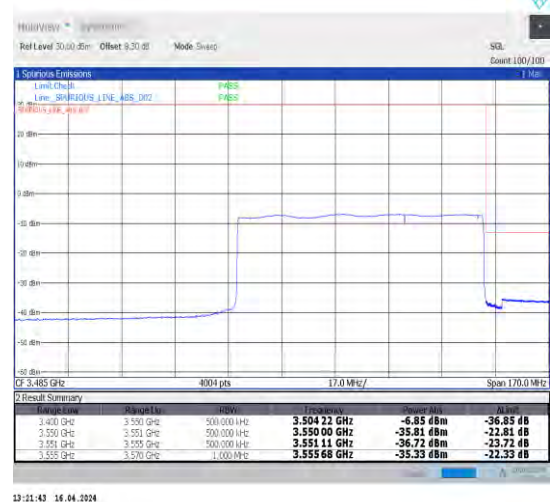
1-N78-3450-3550-30-80-H-6-CP-QPSK-Outer_Full -217@0-Ant1-1--PASS-see graph
