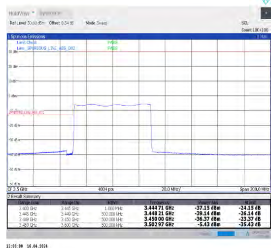
1-N78-3450-3550-30-60-L-6-CP-QPSK-Outer_Full -162@0-Ant1-1--PASS-see graph
