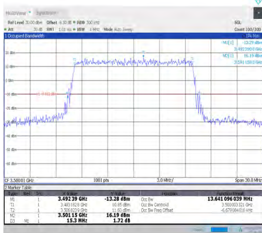
1-N78-3450-3550-30-15-M-6-CP-QPSK-Out_Full-38@0-Ant1-13.641-15.300-≤15-PASS
