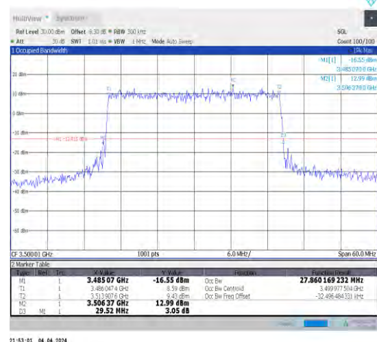
1-N78-3450-3550-30-30-M-8-CP-64QAM-Outer_Full-78@0-Ant1-27.86-29.520-≤30-PASS
