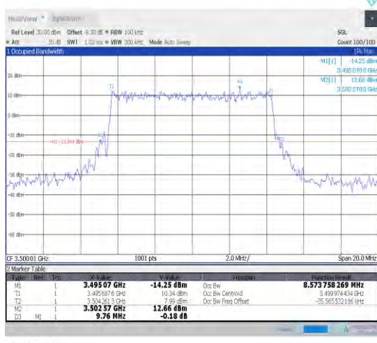
1-N78-3450-3550-30-10-M-7-CP-16QAM-Outer_F ull-24@0-Ant1-8.574-9.760-≤10-PASS
