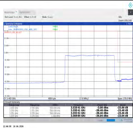
1-N78-3450-3550-30-70-H-3-DFT-PI2BPSK-Outer _Full-180@0-Ant1-1--PASS-see graph
