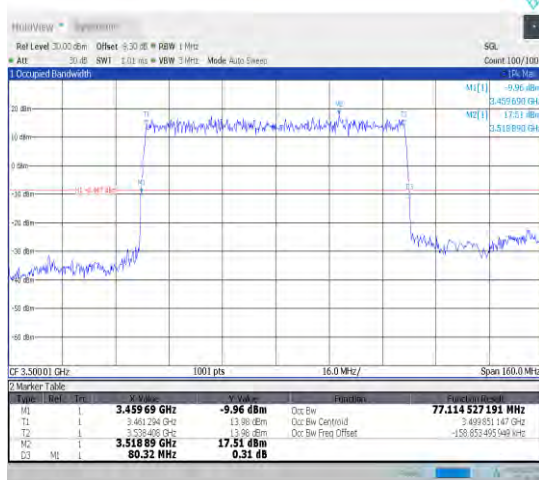
1-N78-3450-3550-30-80-M-2-DFT-PI2BPSK-Outer_Full-216@0-Ant1-77.115-80.320-≤80-PASS
