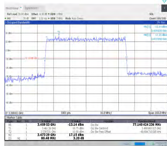
1-N78-3450-3550-30-80-M-3-DFT-16QAM-Outer_Full-216@0-Ant1-77.14-80.480-≤80-PASS
