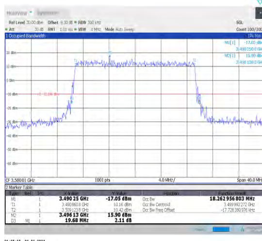
1-N78-3450-3550-30-20-M-6-CP-QPSK-Outer_Full-5 1@0-Ant1-18.263-19.680-≤20-PASS
