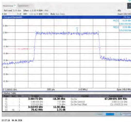
1-N78-3450-3550-30-70-M-9-CP-256QAM-Outer_Full-I-189@0-Ant1-67.39-70.420-≤70-PASS
