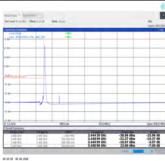
1-N78-3450-3550-30-20-L-1-DFT-PI2BPSK-Edge_1RB _Left-1@0-Ant1-1--PASS-see graph
