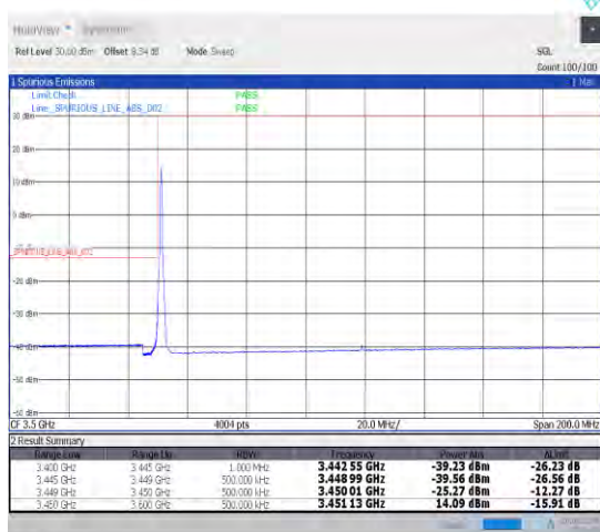
1-N78-3450-3550-30-70-L-4-CP-QPSK-Edge_1RB_Lef t-1@0-Ant1-1--PASS-see graph
