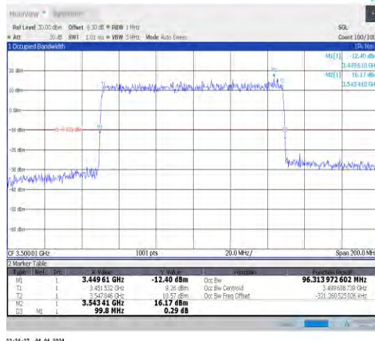
1-N78-3450-3550-30-100-M-3-DFT-16QAM-Outter_Full-270@0-Ant1-96.314-99.800-≤100-PASS
