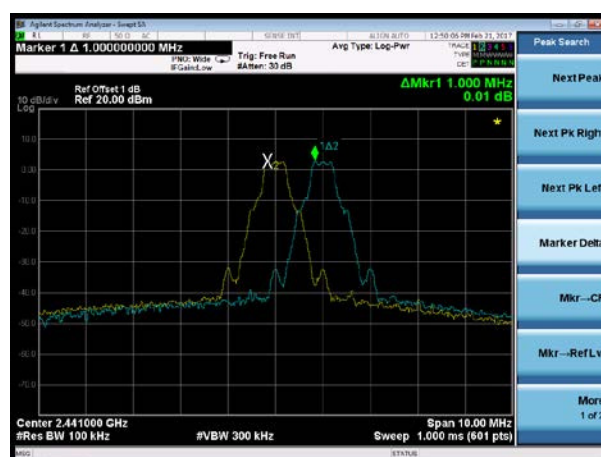
Channel 39 (2441MHz)
