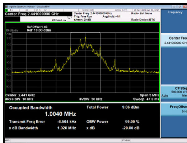
Channel 39 (2441MHz)
