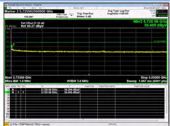
U-NII-2C 11n20 CH140 Peak
