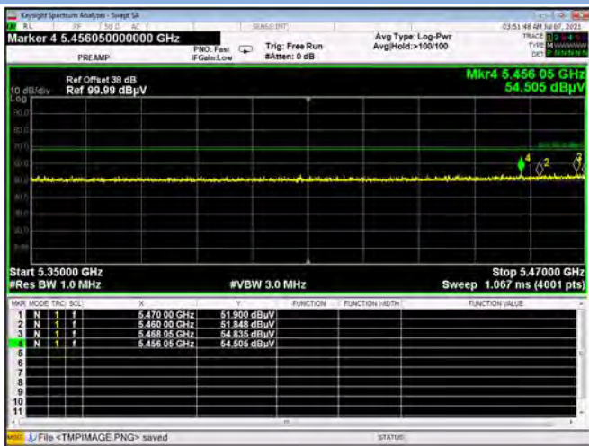
U-NII-2C 11n20 CH100 Peak
