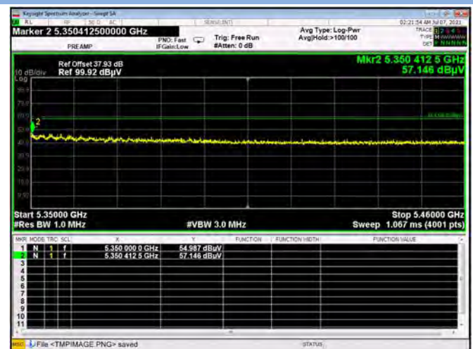
U-NII-2A 11ac80 CH58 Peak
