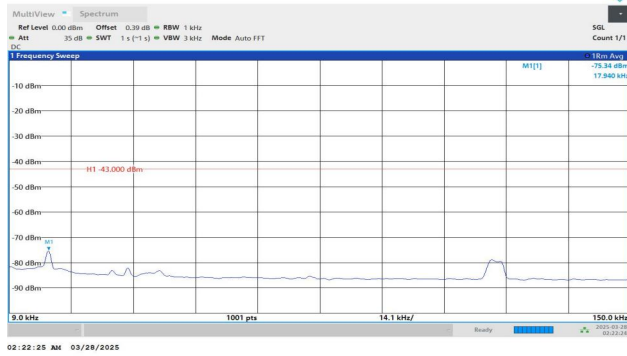
Band2-9400-4-0.009~0.15MHz-PASS
