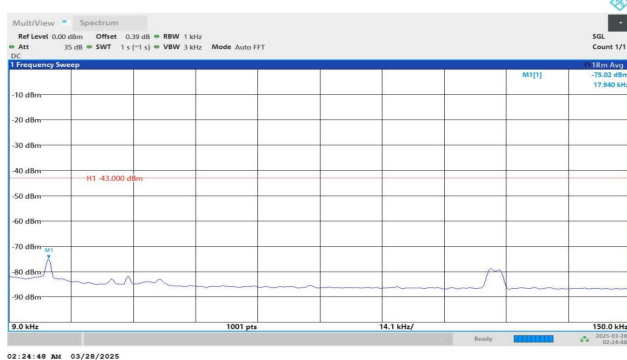
Band2-9400-5-0.009~0.15MHz-PASS
