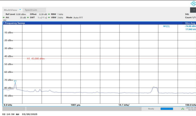
Band2-9538-2-0.009~0.15MHz-PASS
