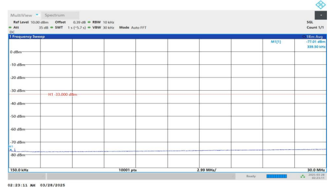
Band2-9538-4-0.15~30MHz-PASS
