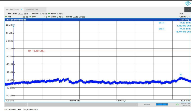
Band2-9262-4-1000~20000MHz-PASS
