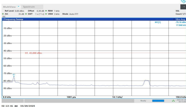
Band2-9400-1-0.009~0.15MHz-PASS
