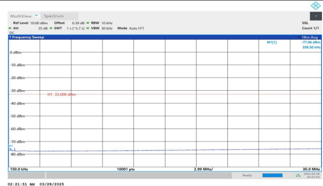
Band2-9262-4-0.15~30MHz-PASS
