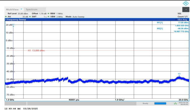
Band2-9262-2-1000~20000MHz-PASS
