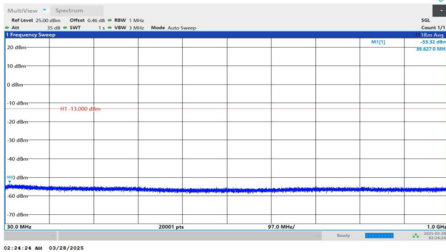
Band2-9262-5-30~1000MHz-PASS
