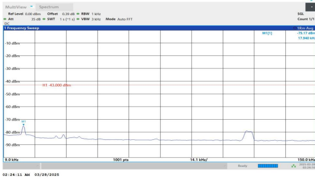
Band2-9262-5-0.009~0.15MHz-PASS
