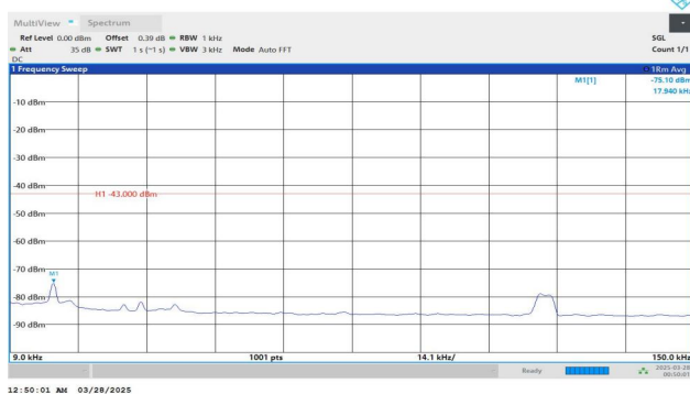
Band2-9400-2-0.009~0.15MHz-PASS
