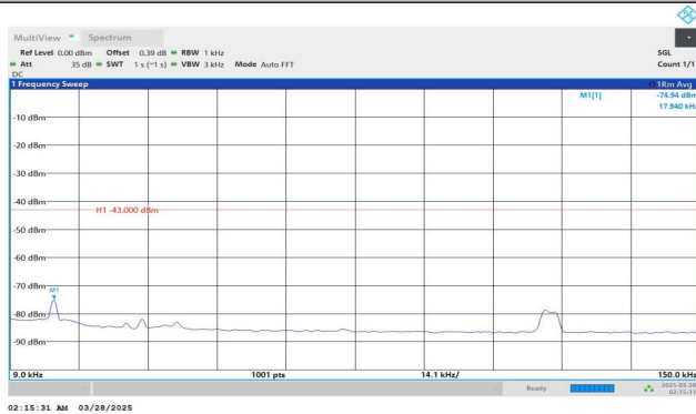
Band2-9262-2-0.009~0.15MHz-PASS
