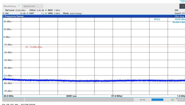
Band2-9400-5-30~1000MHz-PASS
