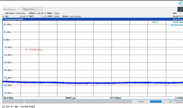
Band2-9262-4-30~1000MHz-PASS
