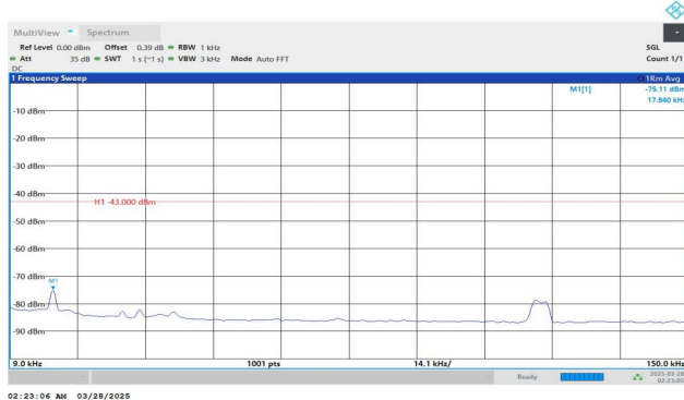
Band2-9538-4-0.009~0.15MHz-PASS
