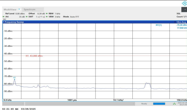
Band2-9262-4-0.009~0.15MHz-PASS
