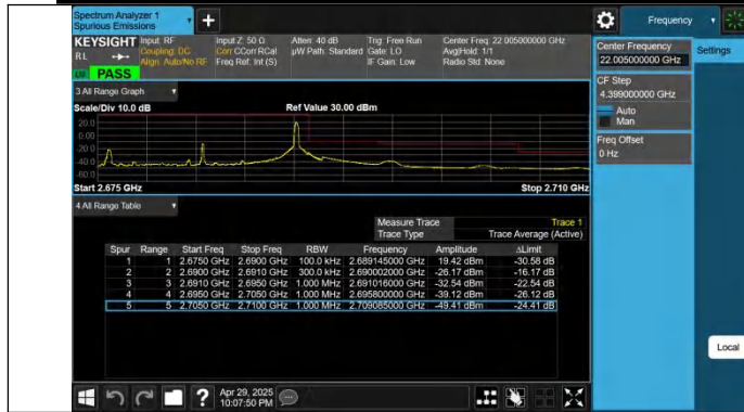
Band41-15MHz-QPSK-41515-1RB#74-PASS
