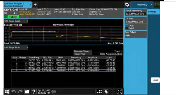
Band41-15MHz-QPSK-41515-75RB#0-PASS
