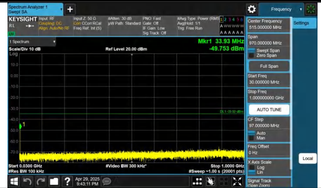
Band41-5MHz-QPSK-40620-1RB#24-30~1000-PASS
