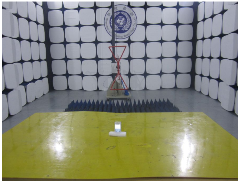
Test Setup Photos of the EUT_PCE
