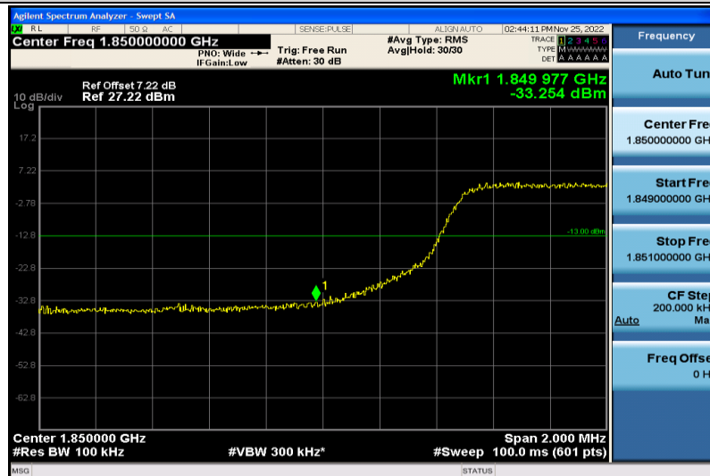
Band2-10MHz-64QAM-18650-50RB#0
