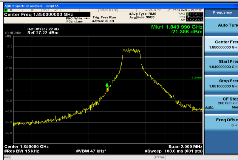
Band2-1.4MHz-64QAM-18607-1RB#0
