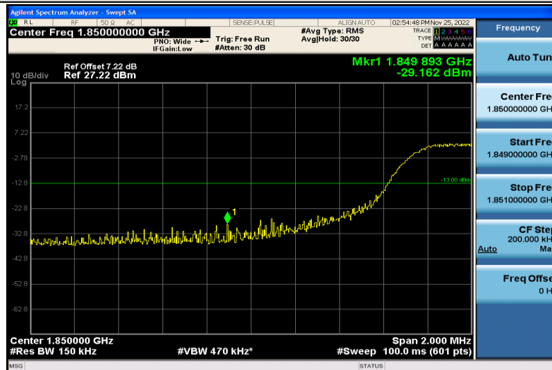
Band2-15MHz-64QAM-18675-75RB#0
