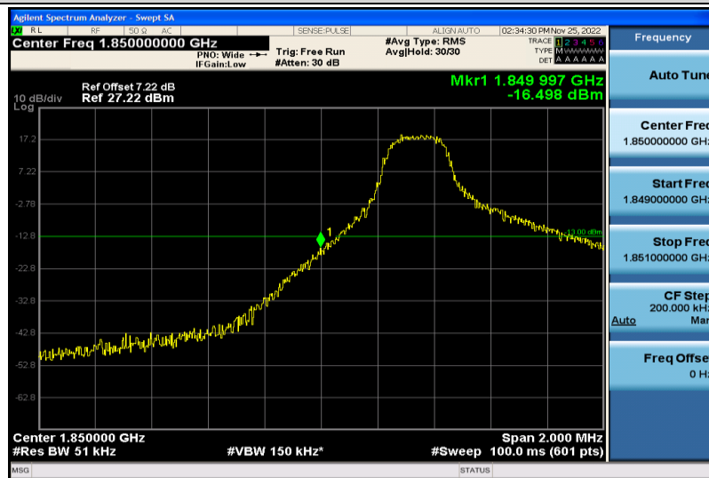
Band2-5MHz-64QAM-18625-1RB#0
