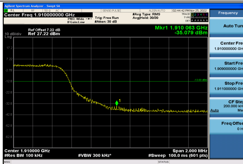
Band2-10MHz-64QAM-19150-50RB#0
