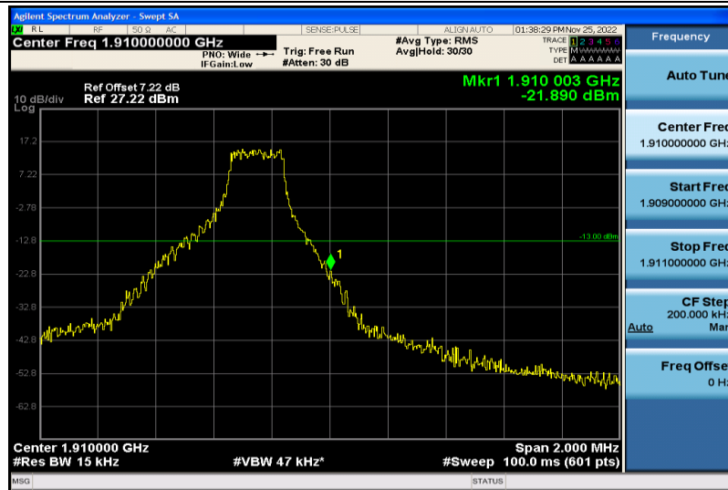
Band2-1.4MHz-64QAM-19193-1RB#5
