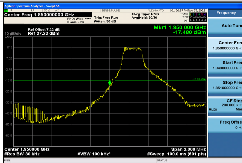
Band2-3MHz-64QAM-18615-1RB#0
