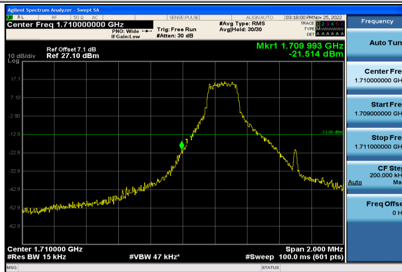
Band4-1.4MHz-64QAM-19957-1RB#0
