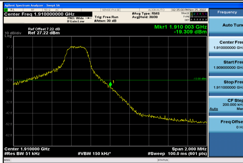
Band2-5MHz-64QAM-19175-1RB#24
