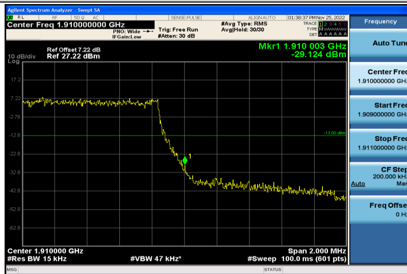
Band2-1.4MHz-64QAM-19193-6RB#0
