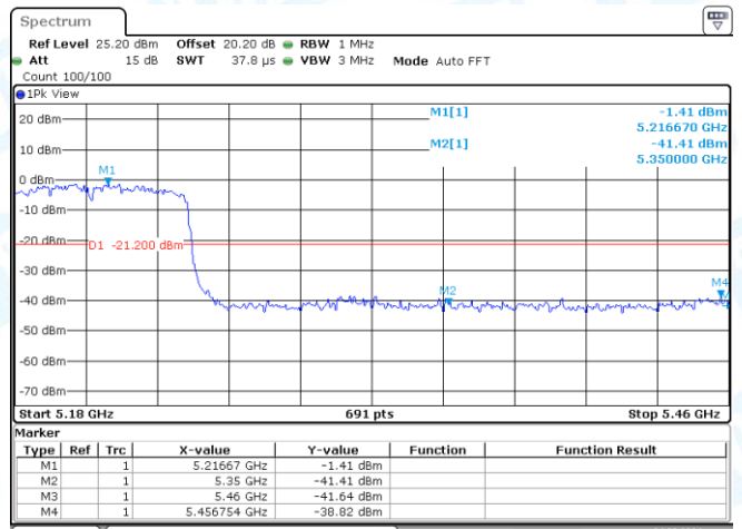
11AC80MIMO-Ant1-5210-PASS
