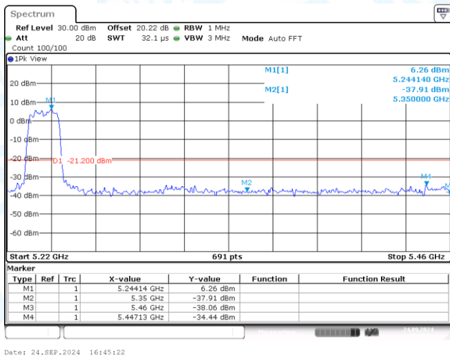
11A-CDD-Ant1-5240-PASS
