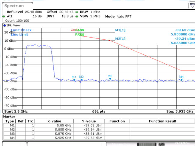
11N20MIMO-Ant1-5745-PASS
