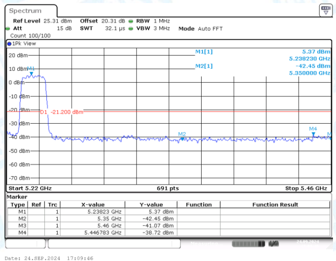
11N20MIMO-Ant2-5240-PASS
