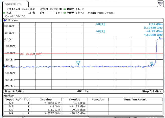
11N40MIMO-Ant2-5190-PASS
