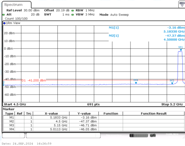
11A-CDD-Ant1-5180-PASS
