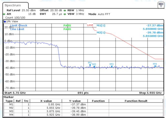
11AC80MIMO-Ant1-5775-PASS
