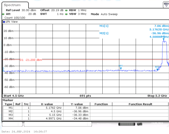
11A-CDD-Ant1-5180-PASS
