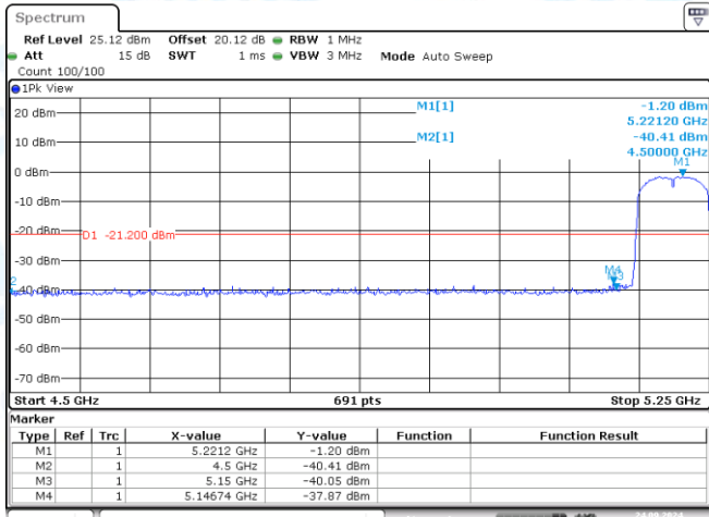
11AC80MIMO-Ant1-5210-PASS
