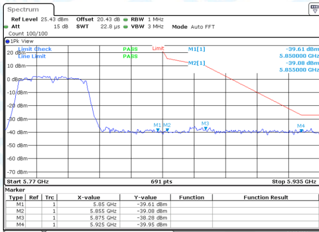
11AC40MIMO-Ant1-5755-PASS
