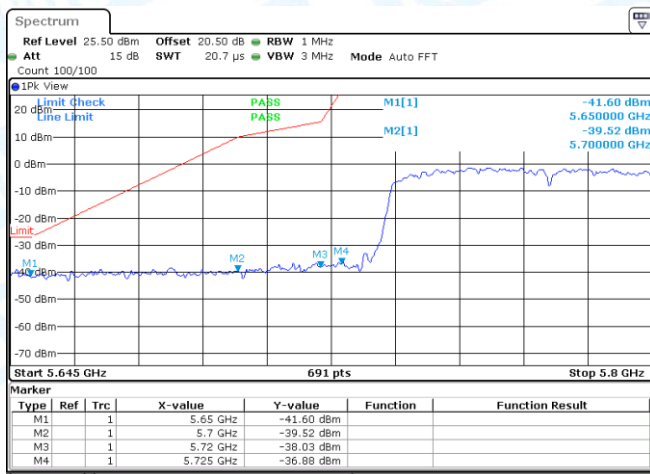
11AC80MIMO-Ant1-5775-PASS
