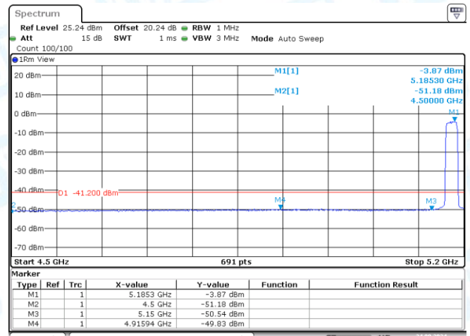
11AC20MIMO-Ant2-5180-PASS
