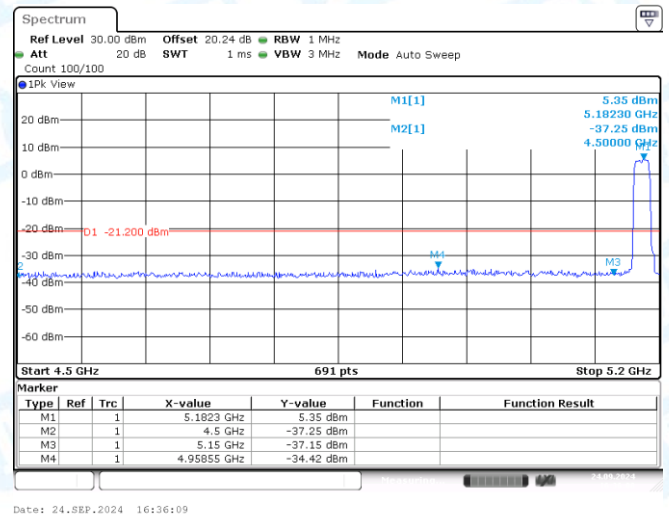
11A-CDD-Ant2-5180-PASS
