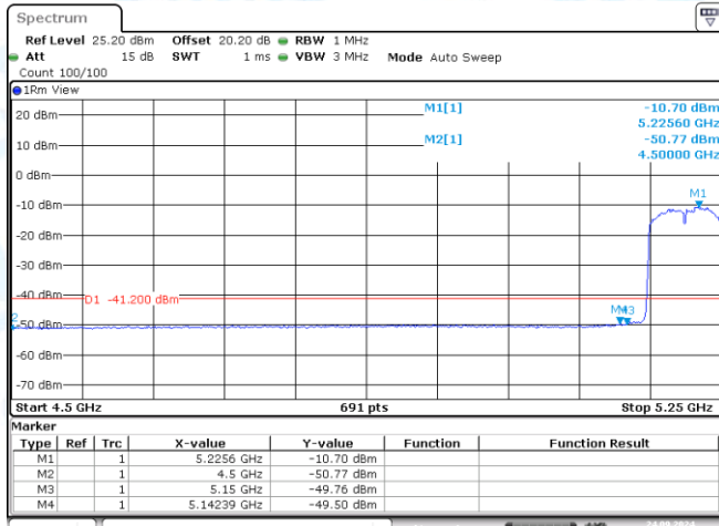
11AC80MIMO-Ant2-5210-PASS
