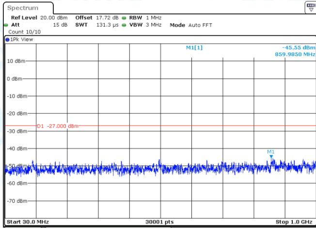
11AC80MIMO-Ant1-5775-30~1000-PASS
