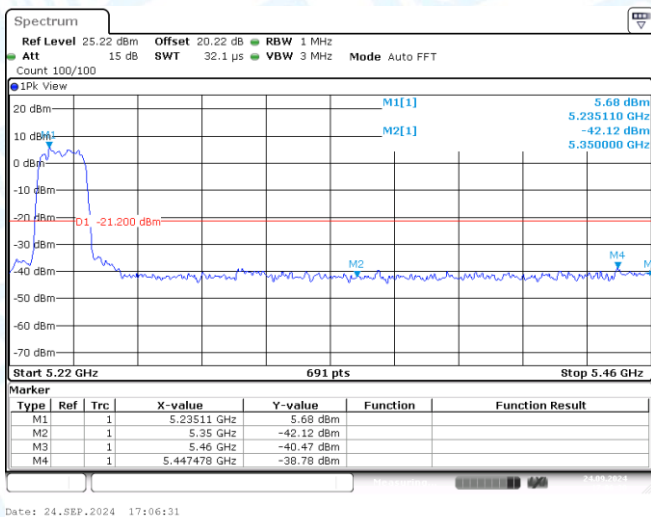
11N20MIMO-Ant1-5240-PASS
