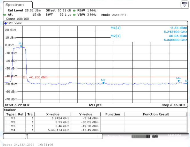
11A-CDD-Ant2-5240-PASS
