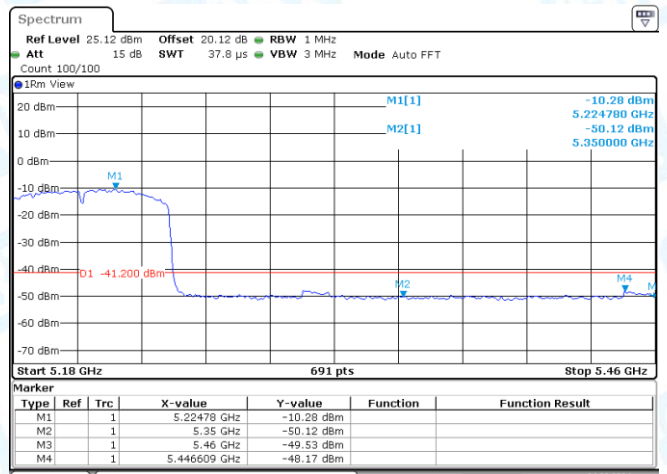
11AC80MIMO-Ant2-5210-PASS
