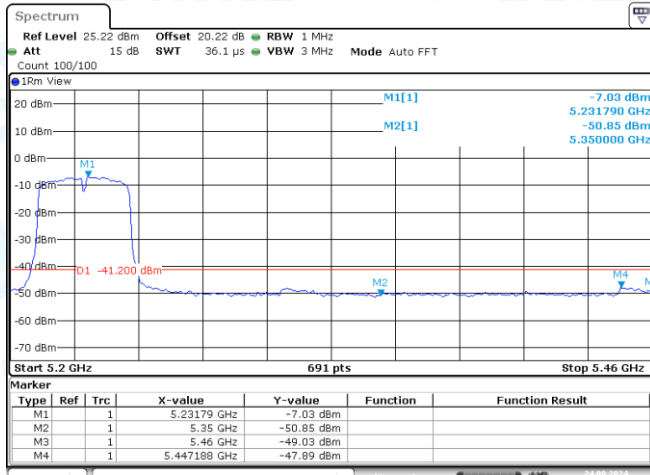
11AC40MIMO-Ant1-5230-PASS
