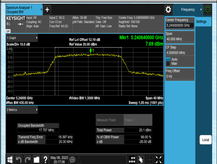
11AC20MIMO-Ant2-5240
