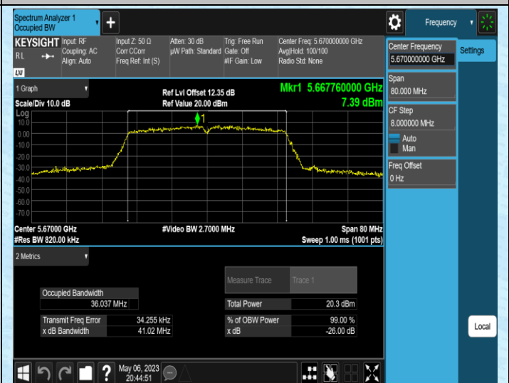
11AC40MIMO-Ant2-5670
