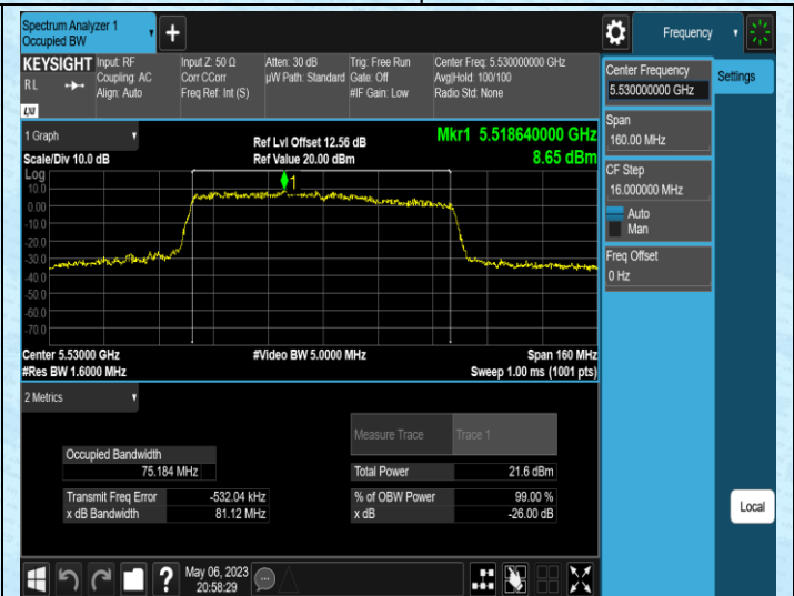
11AC80MIMO-Ant2-5530
