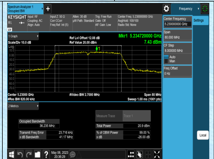
11AC40MIMO-Ant2-5230
