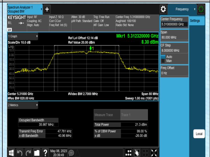
11AC40MIMO-Ant2-5310
