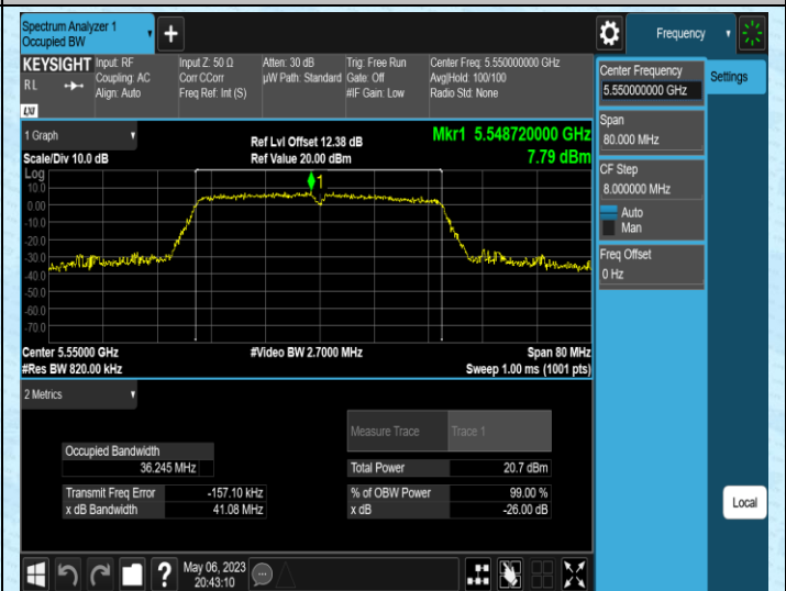
11AC40MIMO-Ant2-5550
