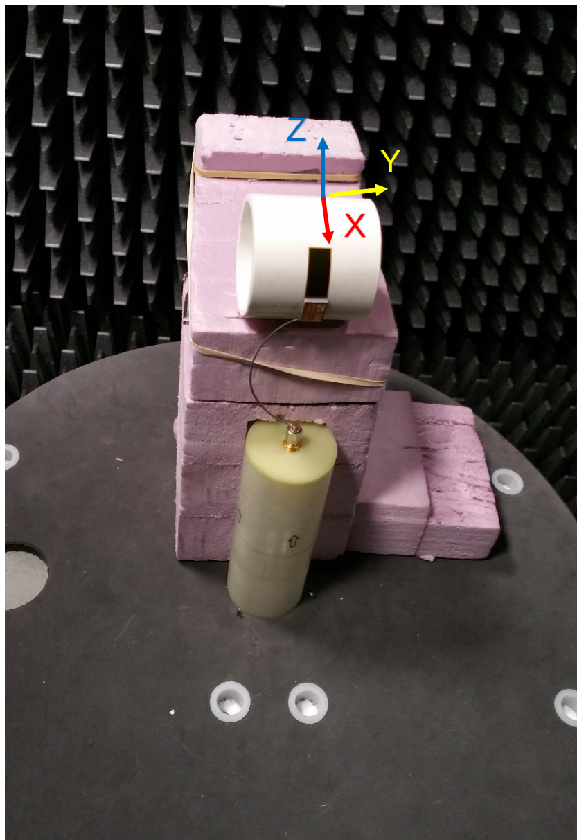
Figure 15: Inner diameter setup
