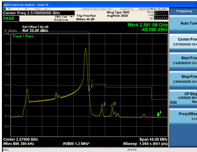
Band7-20MHz-16QAM-21350-100RB#0
