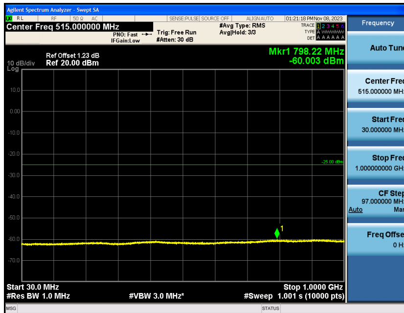
Band7-5MHz-16QAM-21425-1RB#0-Range2:1000~26500MHz
