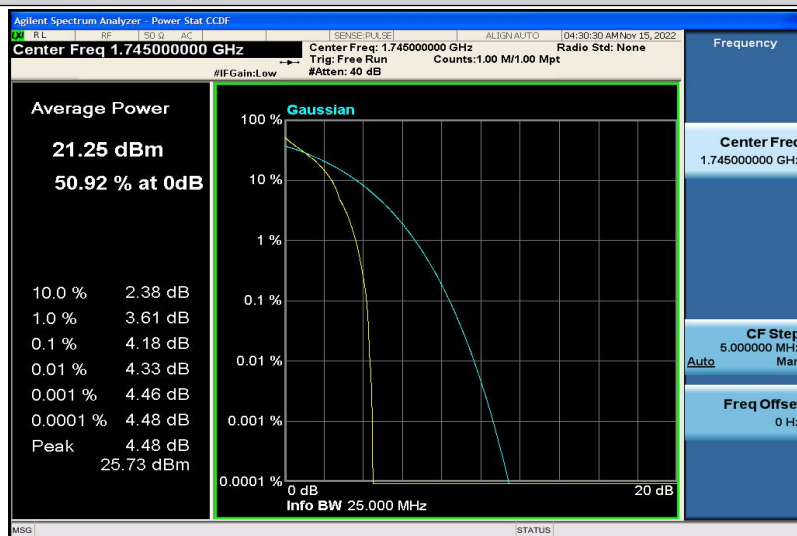
Band66-15MHz-QPSK-132322-1RB#0
