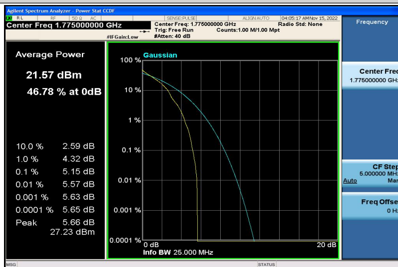
Band66-10MHz-QPSK-132622-1RB#0
