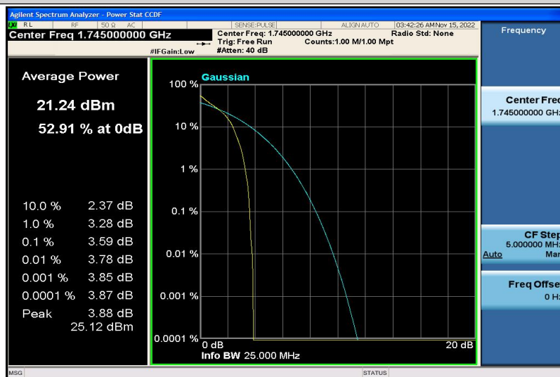
Band66-5MHz-QPSK-132322-1RB#0
