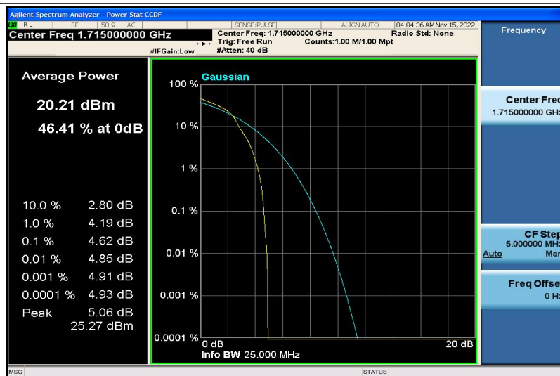
Band66-10MHz-16QAM-132022-1RB#0
