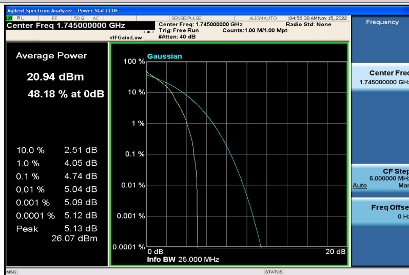
Band66-20MHz-QPSK-132322-1RB#0
