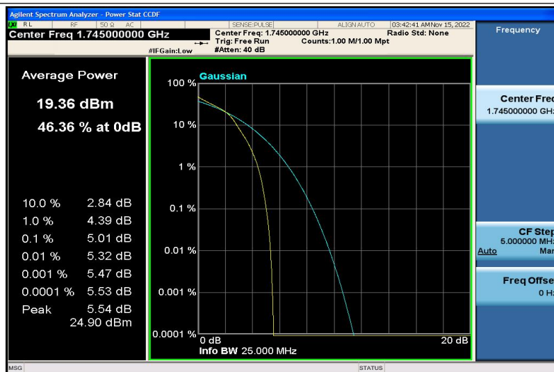
Band66-5MHz-16QAM-132322-25RB#0
