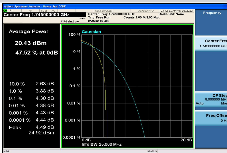
Band66-5MHz-16QAM-132322-1RB#0
