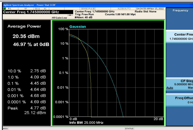
Band66-10MHz-16QAM-132322-1RB#0
