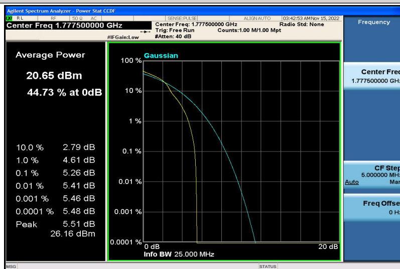
Band66-5MHz-16QAM-132647-1RB#0
