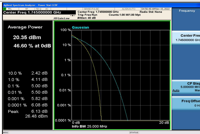
Band66-20MHz-QPSK-132322-100RB#0
