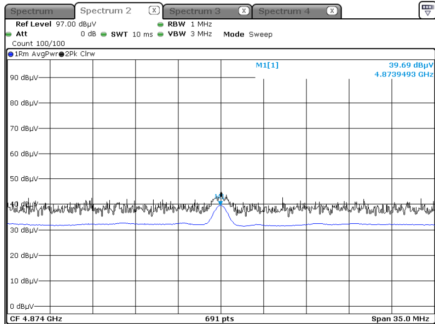
Radiated Spurious Emissions plot – Average Result (802.11b_1 Mbps, Ch.6 2nd Harmonic, X-H)
