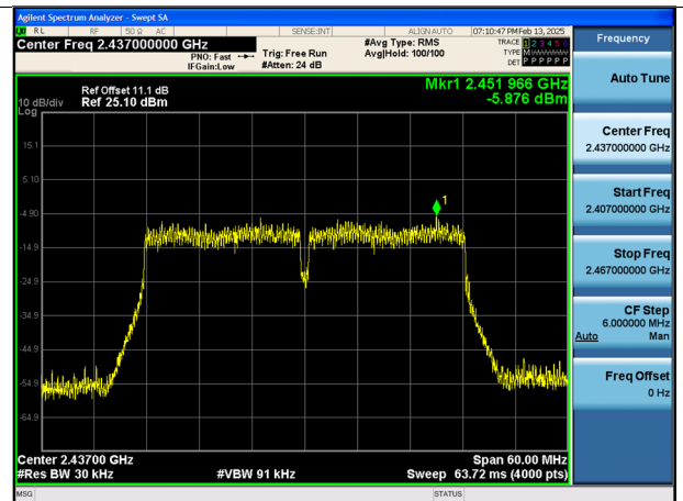
802.11n_HT40-CH 6
