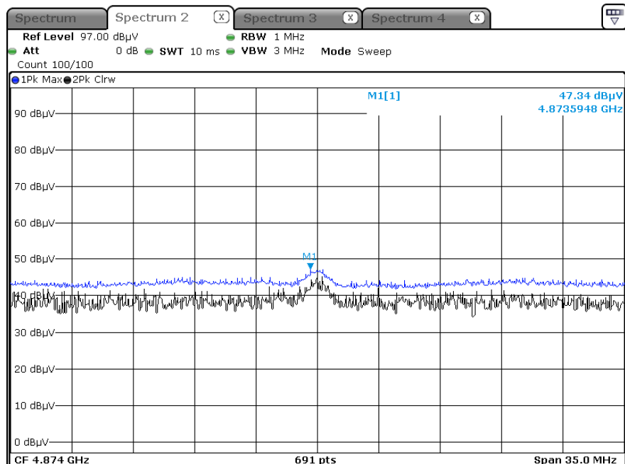
Radiated Spurious Emissions plot – Peak Result (802.11b_1 Mbps, Ch.6 2nd Harmonic, X-H)
