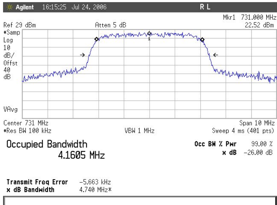
Plot 1. Occupied Bandwidth Low Channel
