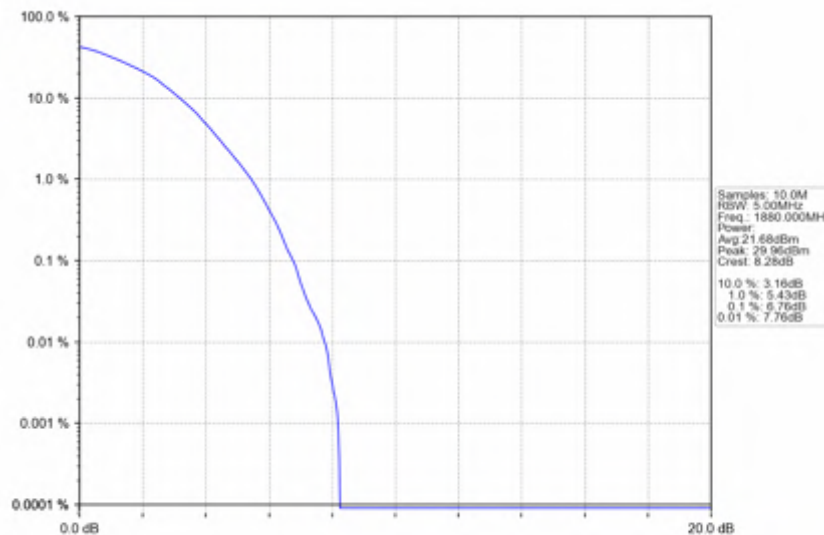
Band2_1.4MHz_16QAM_MCH_1880MHz_RB_6_0_NTNV
