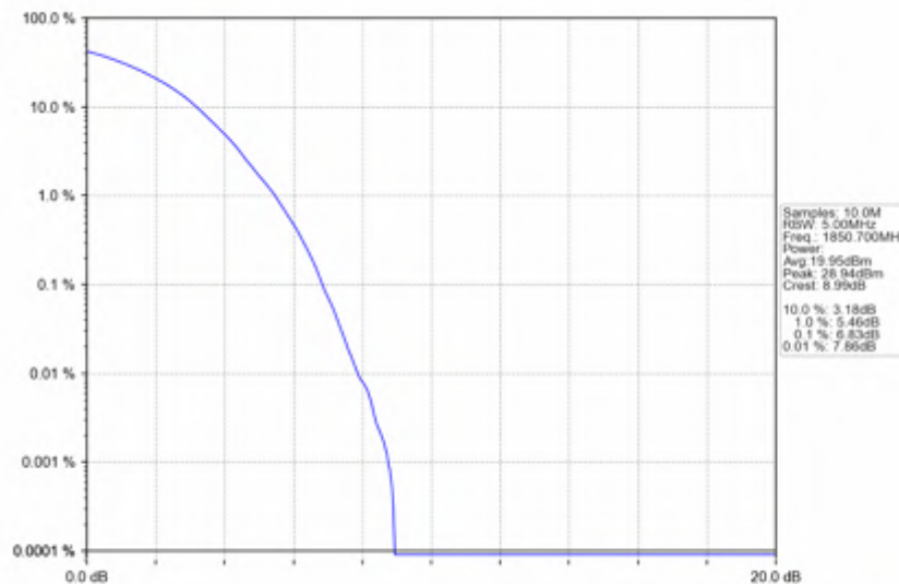
Band2_1.4MHz_256QAM_LCH_1850.7MHz_RB_6_0_NTNV
