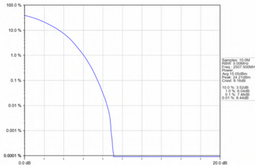
Band7_15MHz_256QAM_LCH_2507.5MHz_RB_75_0_NTNV
