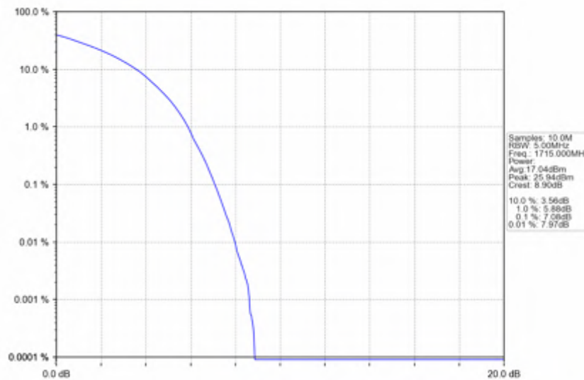
Band4_10MHz_256QAM_LCH_1715MHz_RB_50_0_NTNV
