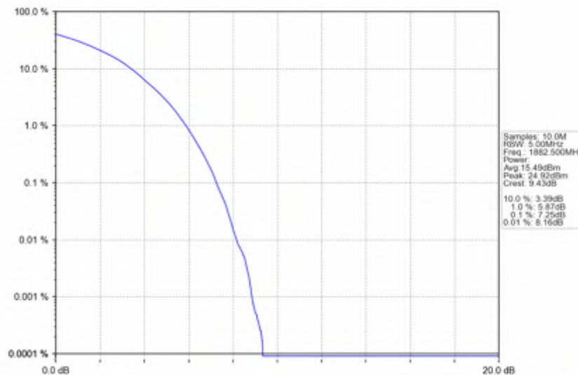
Band25_15MHz_256QAM_MCH_1882.5MHz_RB_75_0_NTNV
