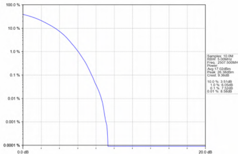
Band7_15MHz_64QAM_LCH_2507.5MHz_RB_75_0_NTNV
