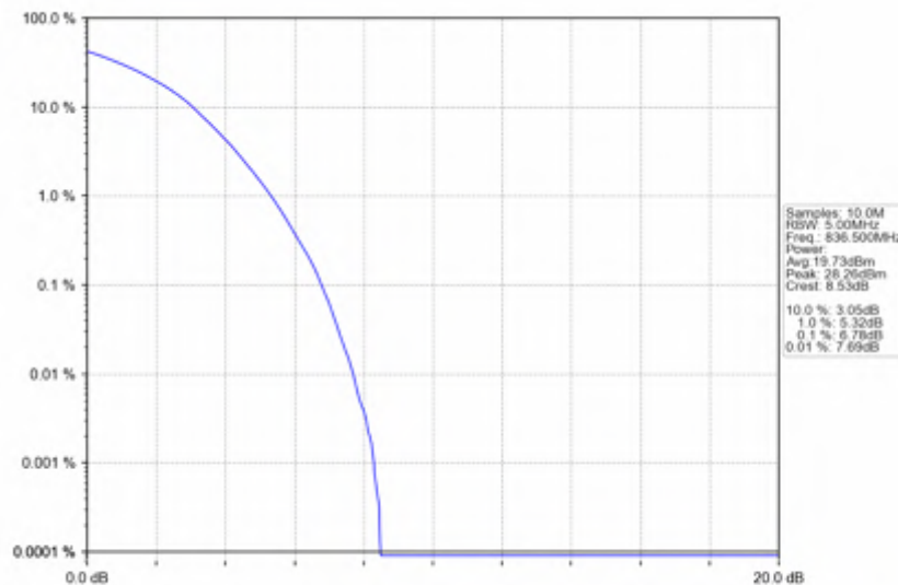
Band5_3MHz_256QAM_MCH_836.5MHz_RB_15_0_NTNV
