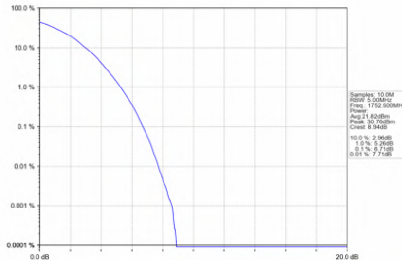
Band4_5MHz_64QAM_HCH_1752.5MHz_RB_25_0_NTNV
