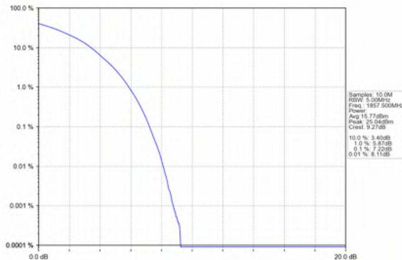
Band25_15MHz_256QAM_LCH_1857.5MHz_RB_75_0_NTNV
