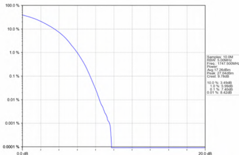
Band4_15MHz_QPSK_HCH_1747.5MHz_RB_75_0_NTNV
