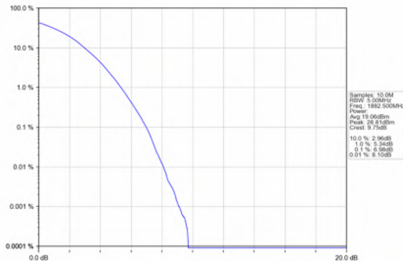
Band25_5MHz_256QAM_MCH_1882.5MHz_RB_25_0_NTNV
