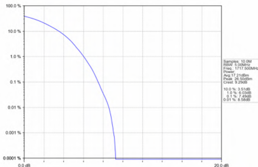
Band4_15MHz_16QAM_LCH_1717.5MHz_RB_75_0_NTNV
