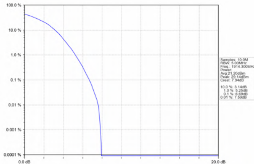
Band25_1.4MHz_64QAM_HCH_1914.3MHz_RB_6_0_NTNV
