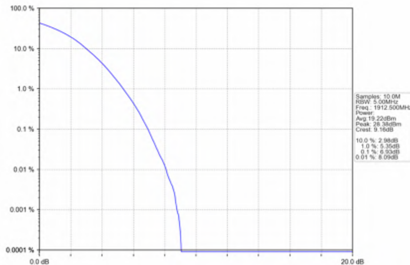
Band25_5MHz_256QAM_HCH_1912.5MHz_RB_25_0_NTNV
