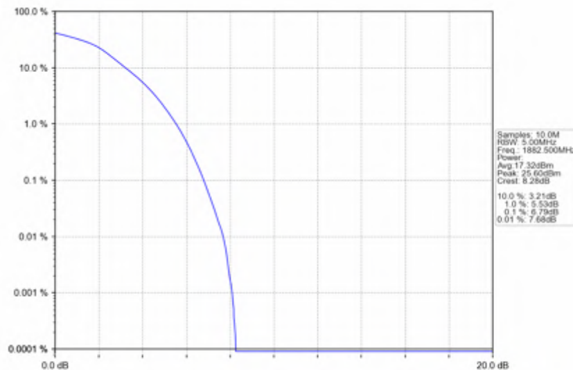
Band25_10MHz_256QAM_MCH_1882.5MHz_RB_50_0_NTNV
