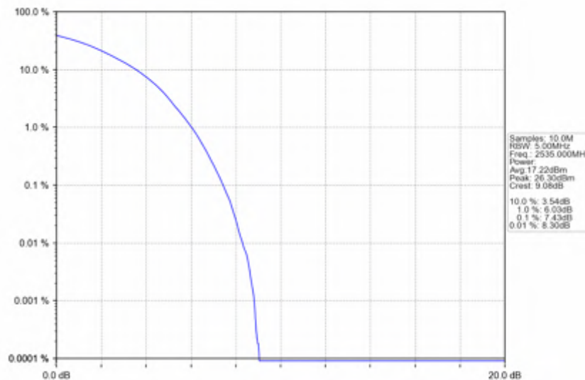
Band7_15MHz_64QAM_MCH_2535MHz_RB_75_0_NTNV
