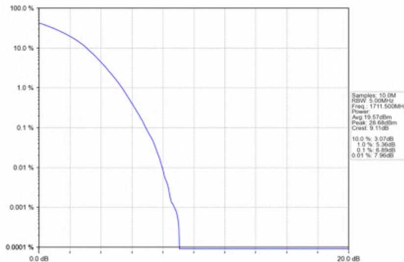
Band4_3MHz_256QAM_LCH_1711.5MHz_RB_15_0_NTNV
