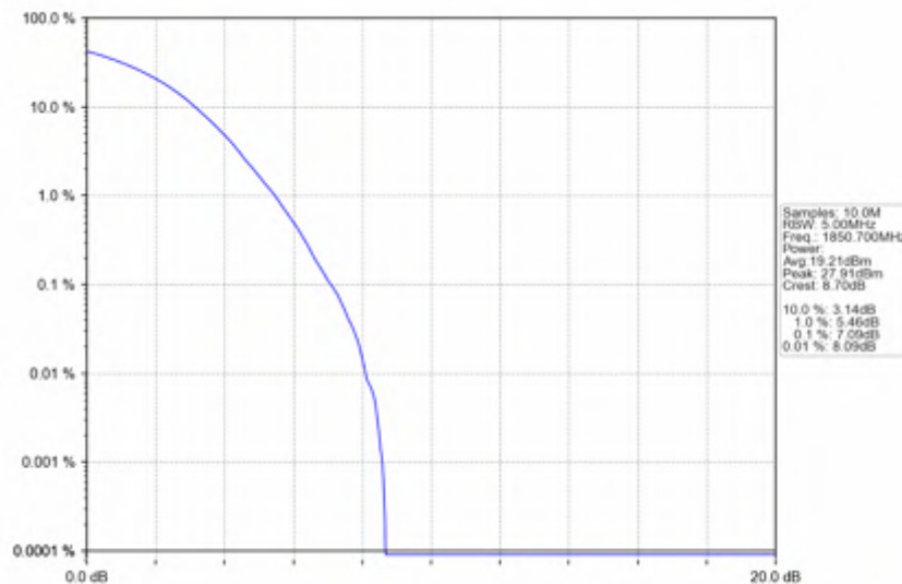
Band25_1.4MHz_256QAM_LCH_1850.7MHz_RB_6_0_NTNV
