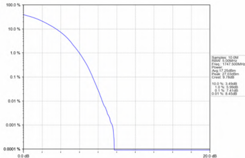
Band4_15MHz_16QAM_HCH_1747.5MHz_RB_75_0_NTNV
