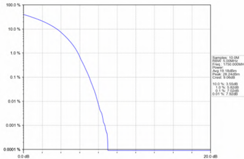
Band4_10MHz_64QAM_HCH_1750MHz_RB_50_0_NTNV
