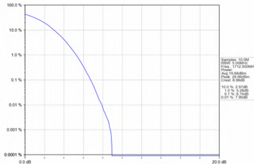
Band4_5MHz_256QAM_LCH_1712.5MHz_RB_25_0_NTNV
