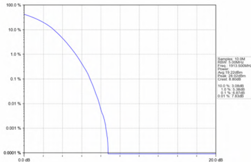
Band25_3MHz_256QAM_HCH_1913.5MHz_RB_15_0_NTNV
