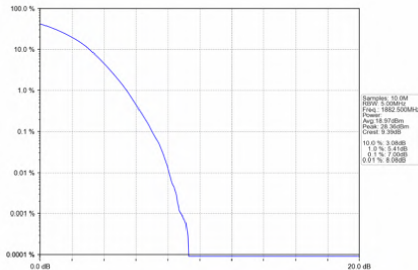
Band25_3MHz_256QAM_MCH_1882.5MHz_RB_15_0_NTNV
