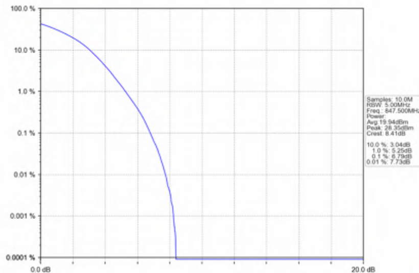
Band5_3MHz_256QAM_HCH_847.5MHz_RB_15_0_NTNV
