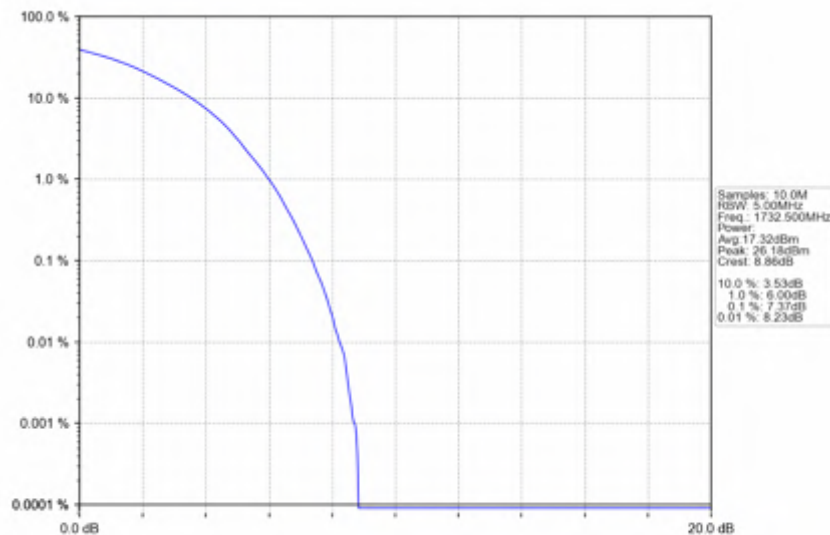
Band4_15MHz_16QAM_MCH_1732.5MHz_RB_75_0_NTNV
