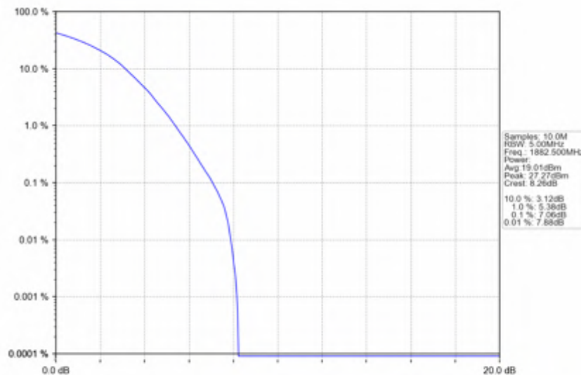
Band25_1.4MHz_256QAM_MCH_1882.5MHz_RB_6_0_NTNV
