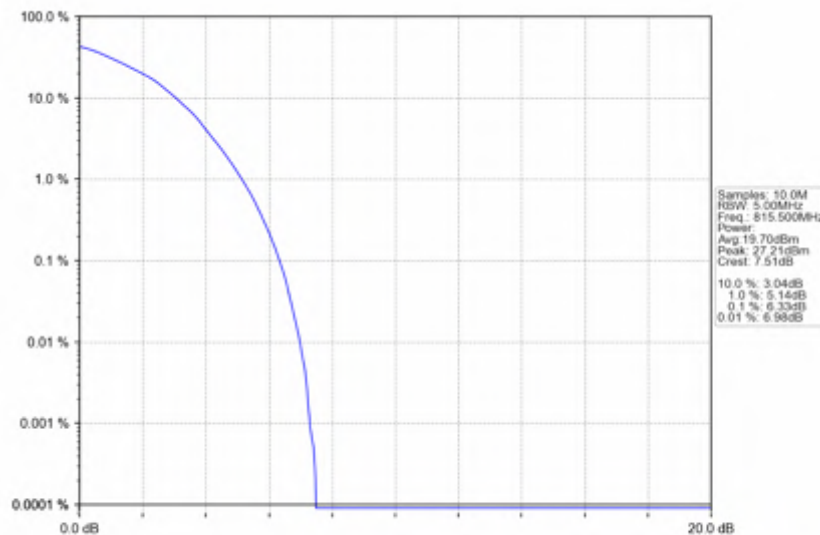
Band26a_3MHz_64QAM_LCH_815.5MHz_RB_15_0_NTNV
