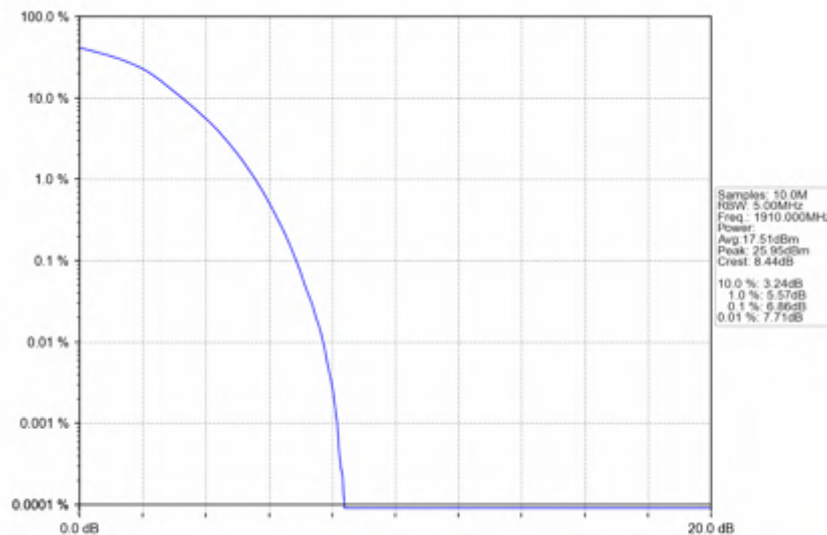
Band25_10MHz_256QAM_HCH_1910MHz_RB_50_0_NTNV
