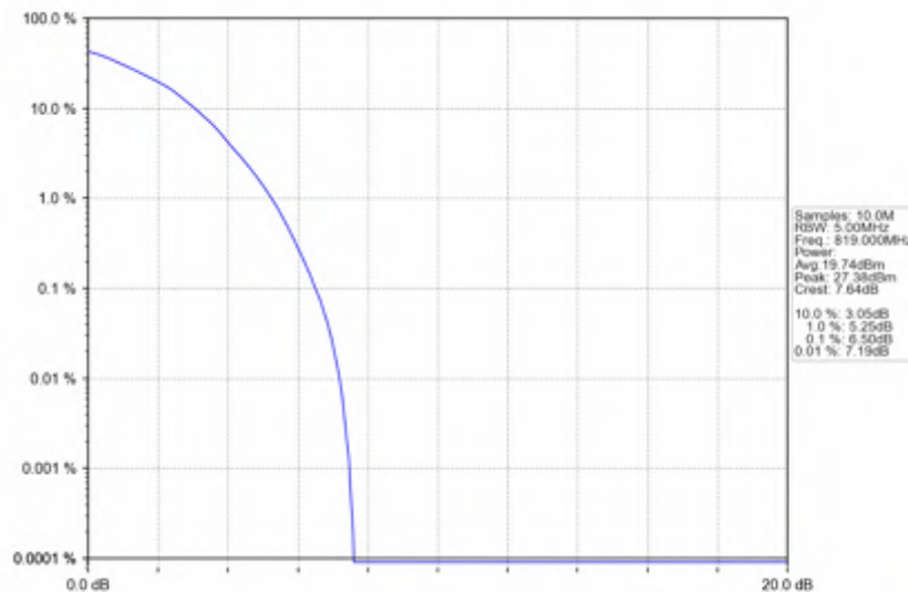
Band26a_3MHz_64QAM_MCH_819MHz_RB_15_0_NTNV
