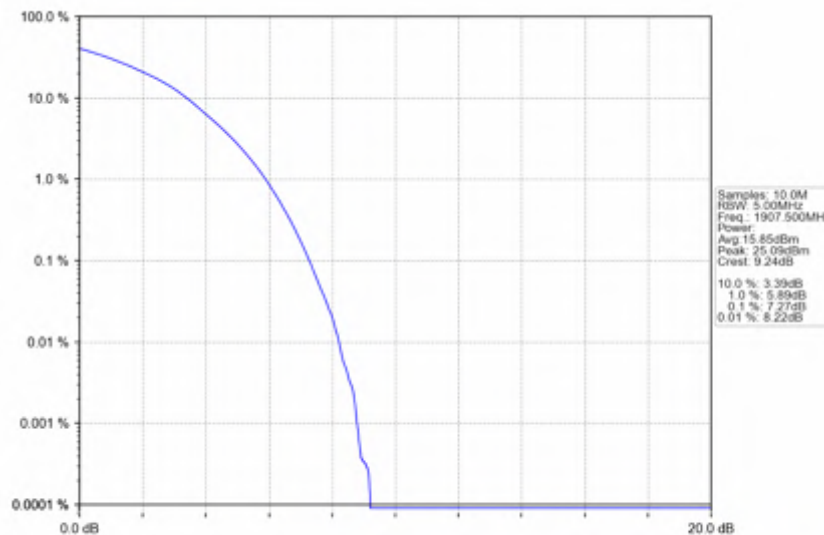
Band25_15MHz_256QAM_HCH_1907.5MHz_RB_75_0_NTNV
