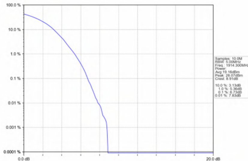
Band25_1.4MHz_256QAM_HCH_1914.3MHz_RB_6_0_NTNV
