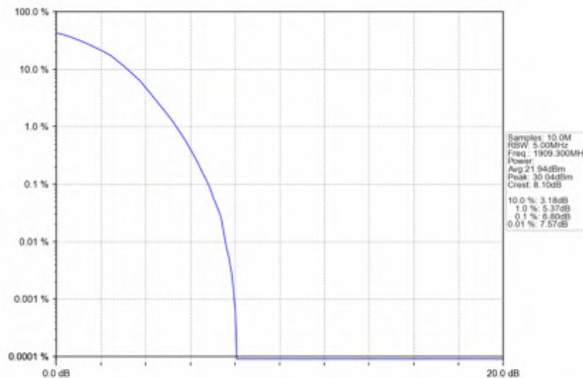
Band2_1.4MHz_16QAM_HCH_1909.3MHz_RB_6_0_NTNV
