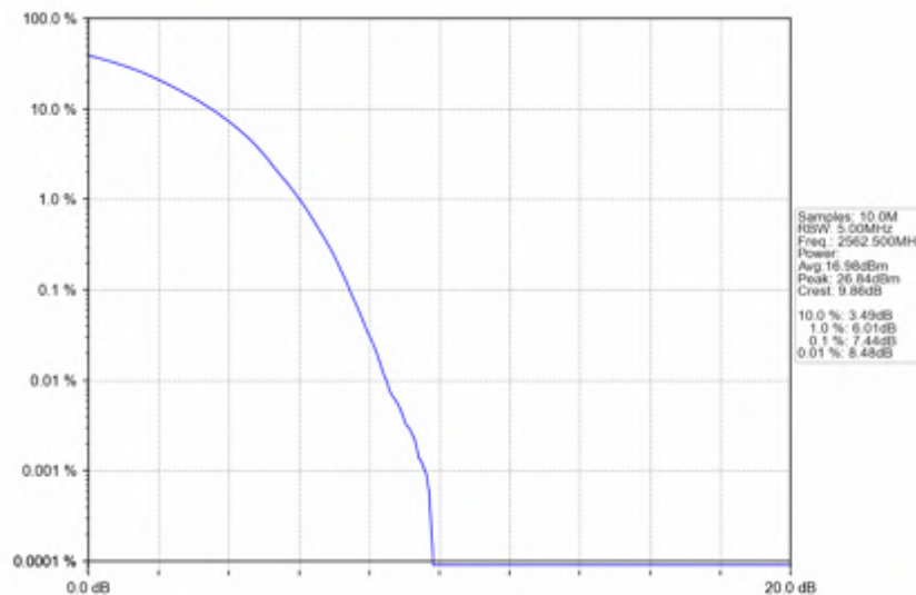
Band7_15MHz_64QAM_HCH_2562.5MHz_RB_75_0_NTNV
