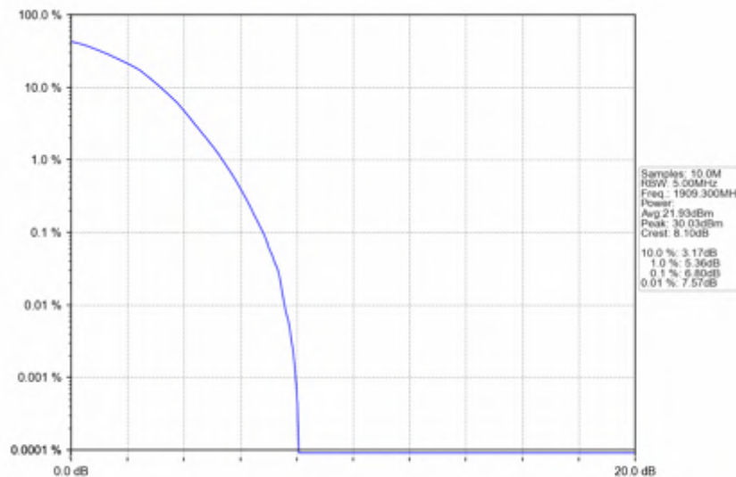
Band2_1.4MHz_64QAM_HCH_1909.3MHz_RB_6_0_NTNV
