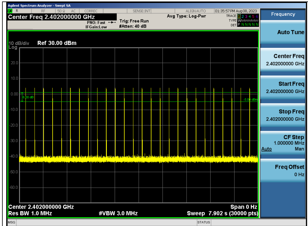
Test_Graph_EDR_HOP_ANT1_NA_2Mbps_2402_Number of Burstr
