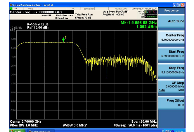
Mode:802.11ax HE20 Tone:106T Frequency:5700MHz Ant:Chain1
