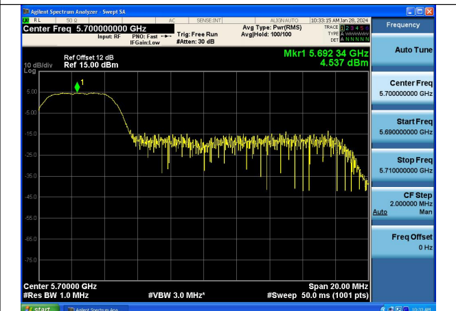
Mode:802.11ax HE20 Tone:52T Frequency:5700MHz Ant:Chain1
