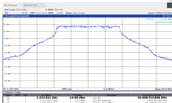
Figure 8.5-10: TSM-Bandwidth 20MHz 99 % occupied bandwidth, 2422 MHz
