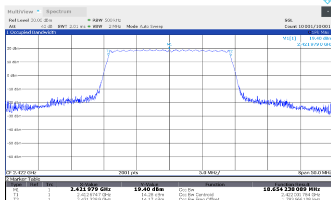
Figure 8.5-12: HDR-Bandwidth 20MHz 99 % occupied bandwidth, 2422 MHz
