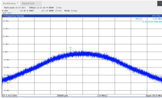
Figure 8.4-7: TSM- Bandwidth 10MHz Power spectral density, 2412 MHz
