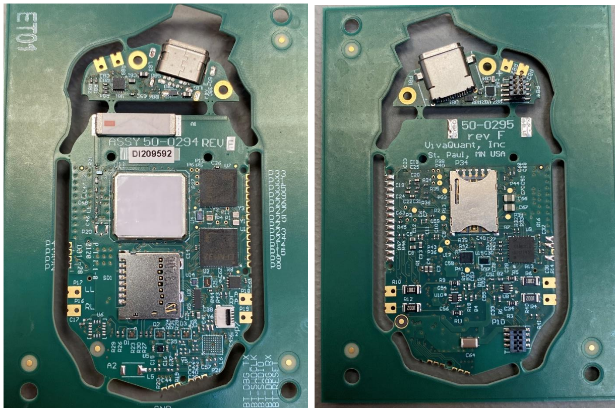
Internal Photos RX-2 Front and Back
