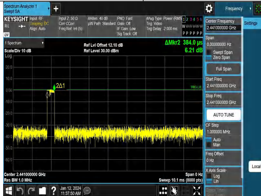
2DH1-Ant1-Hop-PASS
