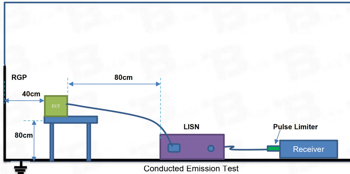
Test Setup 2
