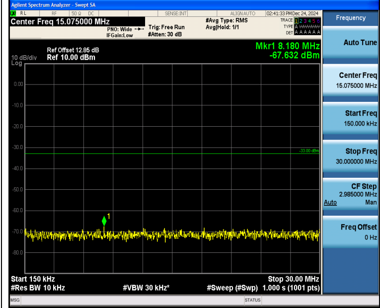
Band4_3MHz_QPSK_20385_1RB#14_0.15~30_0.15~30
