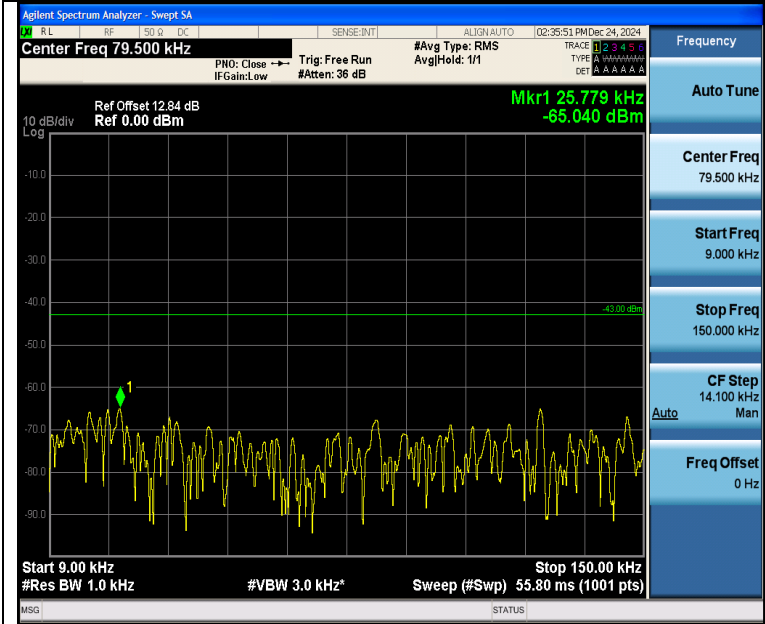
Band4_3MHz_16QAM_20175_1RB#14_0.009~0.15_0.009~0.15
