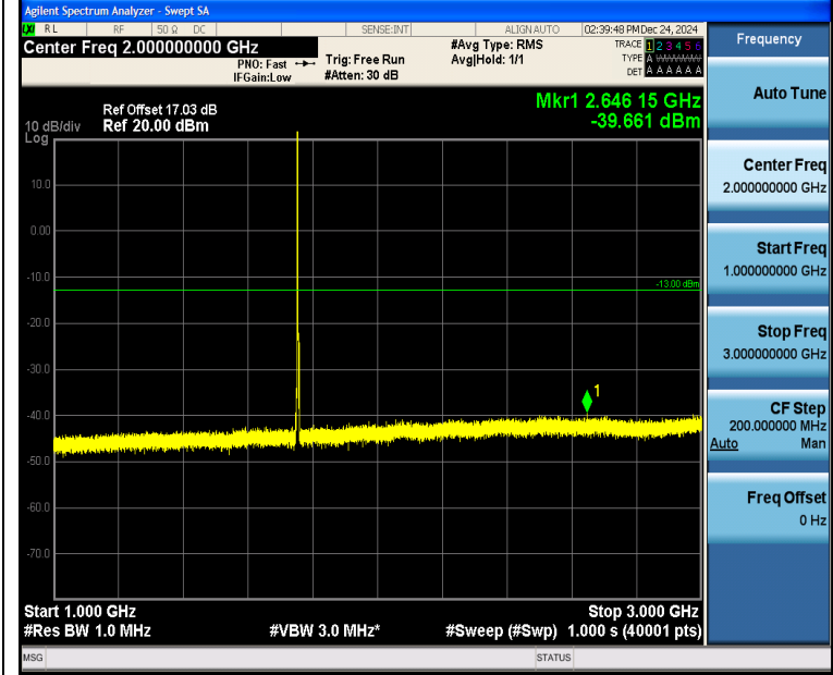
Band4_3MHz_QPSK_20385_1RB#0_1000~3000_1000~3000
