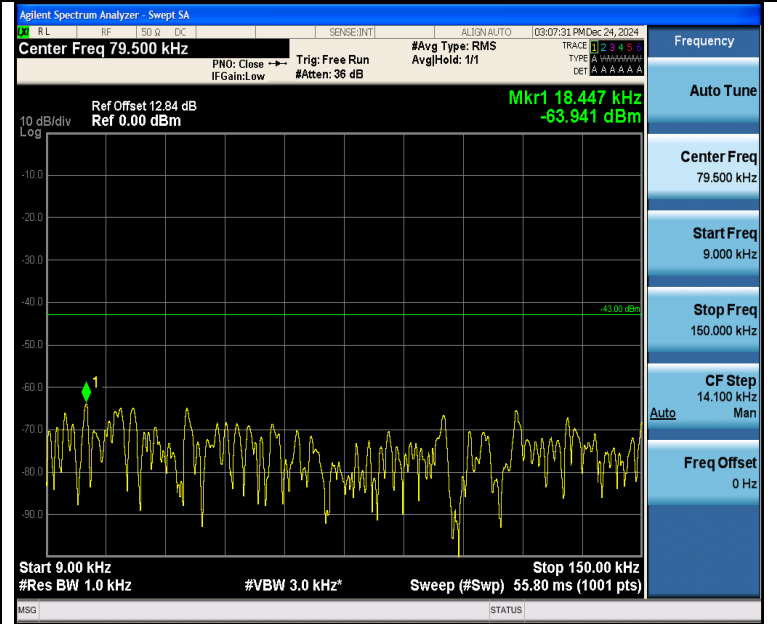
Band4_5MHz_QPSK_19975_25RB#0_0.009~0.15_0.009~0.15
