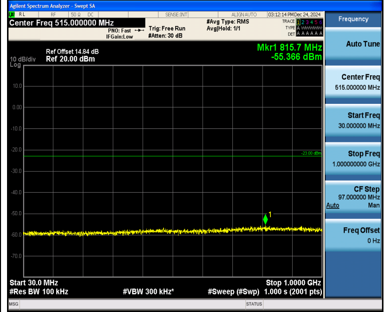
Band4_5MHz_QPSK_20175_1RB#24_30~1000_30~1000
