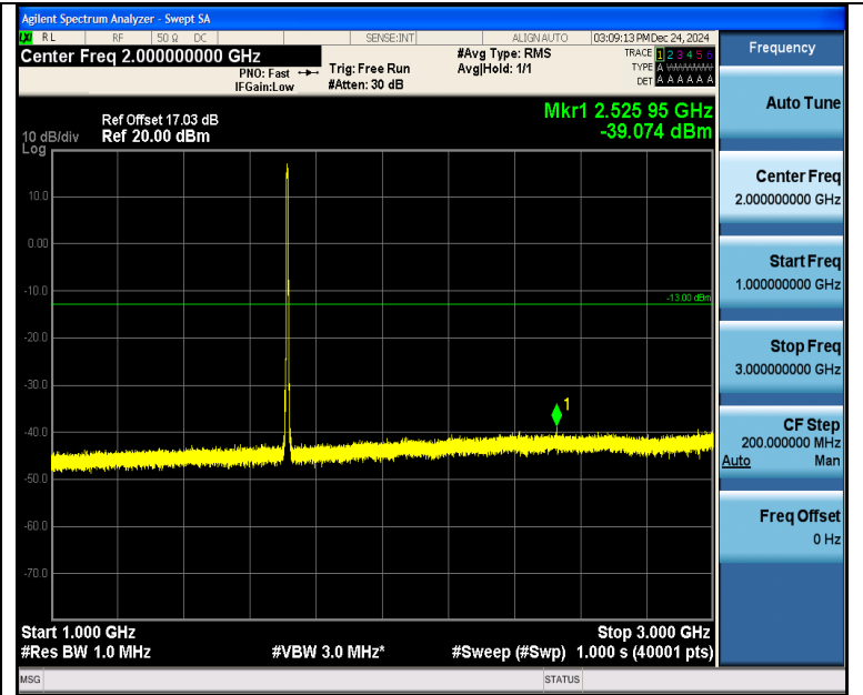
Band4_5MHz_16QAM_19975_25RB#0_1000~3000_1000~3000
