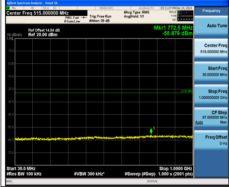
Band4_5MHz_16QAM_20175_1RB#0_30~1000_30~1000
