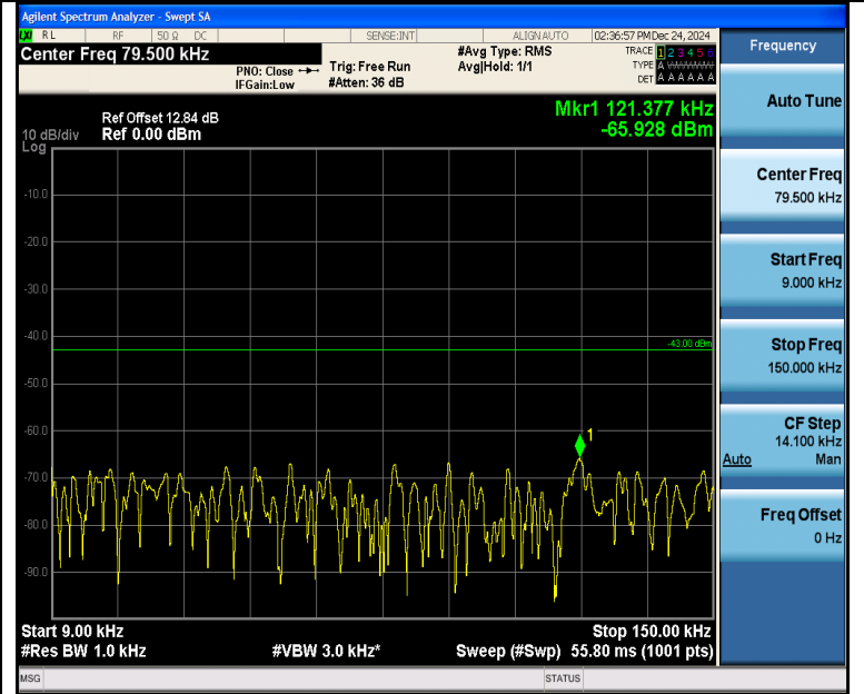
Band4_3MHz_QPSK_20175_15RB#0_0.009~0.15_0.009~0.15
