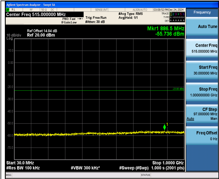
Band4_5MHz_16QAM_19975_25RB#0_30~1000_30~1000
