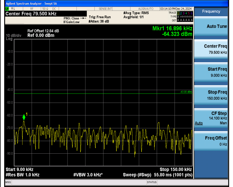
Band4_5MHz_QPSK_20175_25RB#0_0.009~0.15_0.009~0.15
