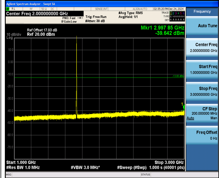
Band4_3MHz_QPSK_20175_1RB#14_1000~3000_1000~3000
