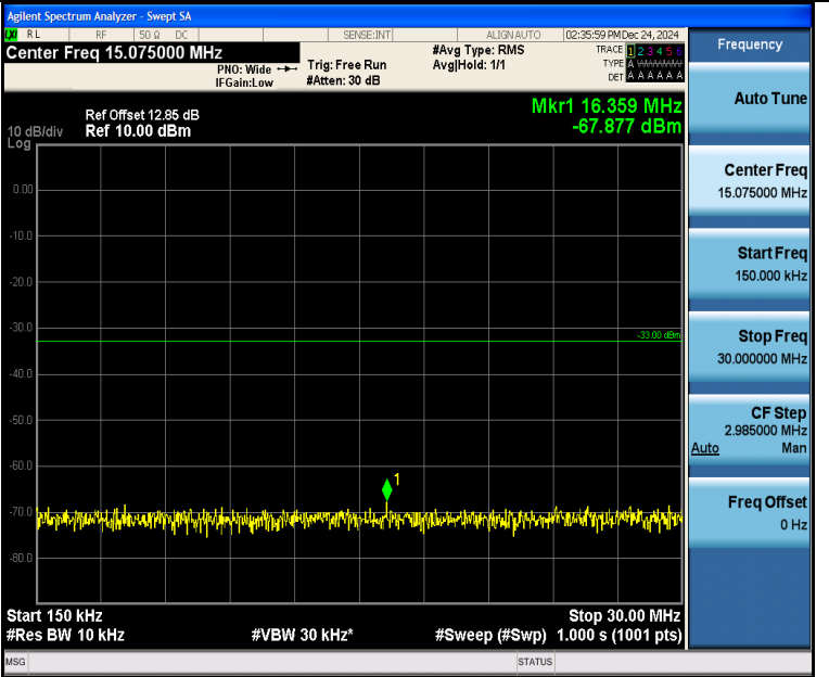
Band4_3MHz_16QAM_20175_1RB#14_0.15~30_0.15~30
