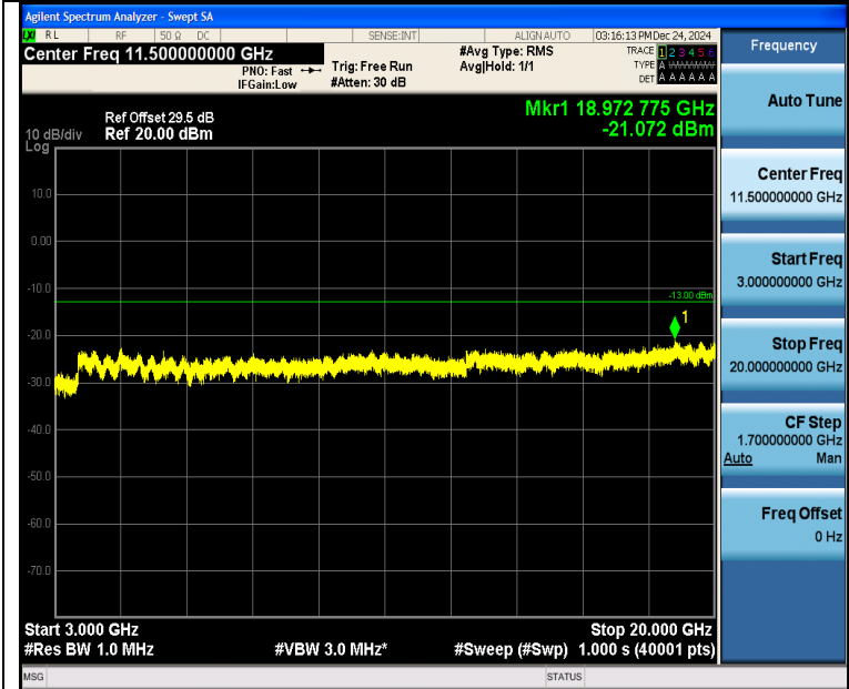
Band4_5MHz_16QAM_20175_25RB#0_3000~20000_3000~20000
