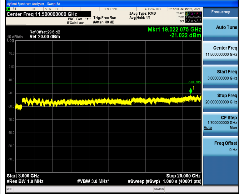
Band4_3MHz_16QAM_20175_15RB#0_3000~20000_3000~20000
