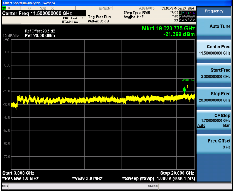
Band4_5MHz_QPSK_20175_1RB#0_3000~20000_3000~20000
