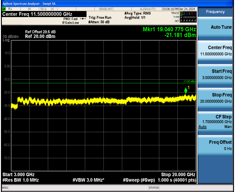
Band4_5MHz_QPSK_19975_1RB#24_3000~20000_3000~20000
