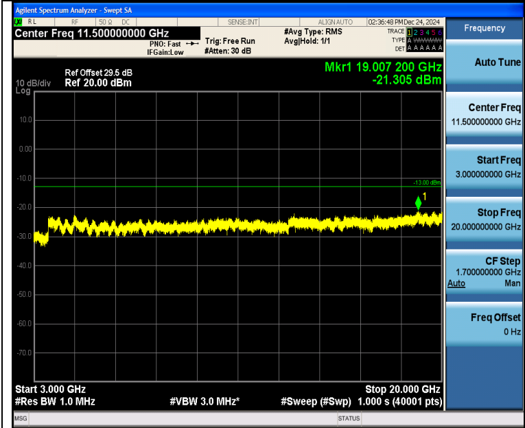
Band4_3MHz_16QAM_20175_1RB#14_3000~20000_3000~20000
