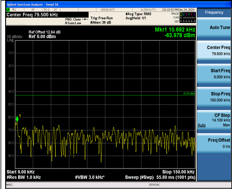
Band4_5MHz_16QAM_20175_1RB#0_0.009~0.15_0.009~0.15
