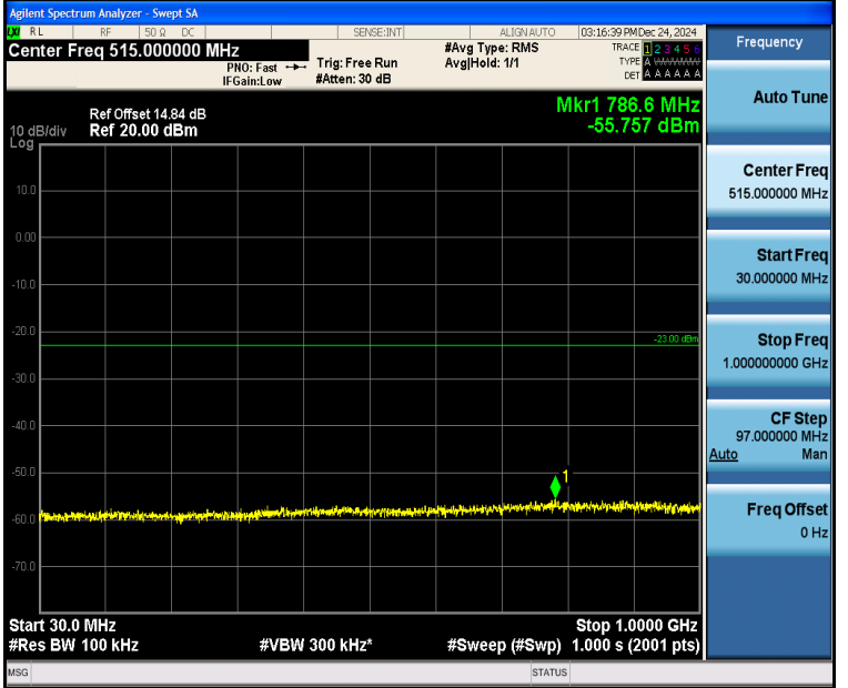
Band4_5MHz_QPSK_20375_1RB#0_30~1000_30~1000
