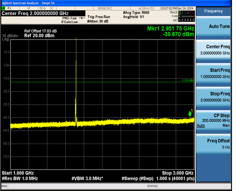
Band4_5MHz_16QAM_19975_1RB#24_1000~3000_1000~3000
