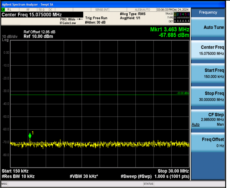
Band4_5MHz_16QAM_19975_1RB#24_0.15~30_0.15~30
