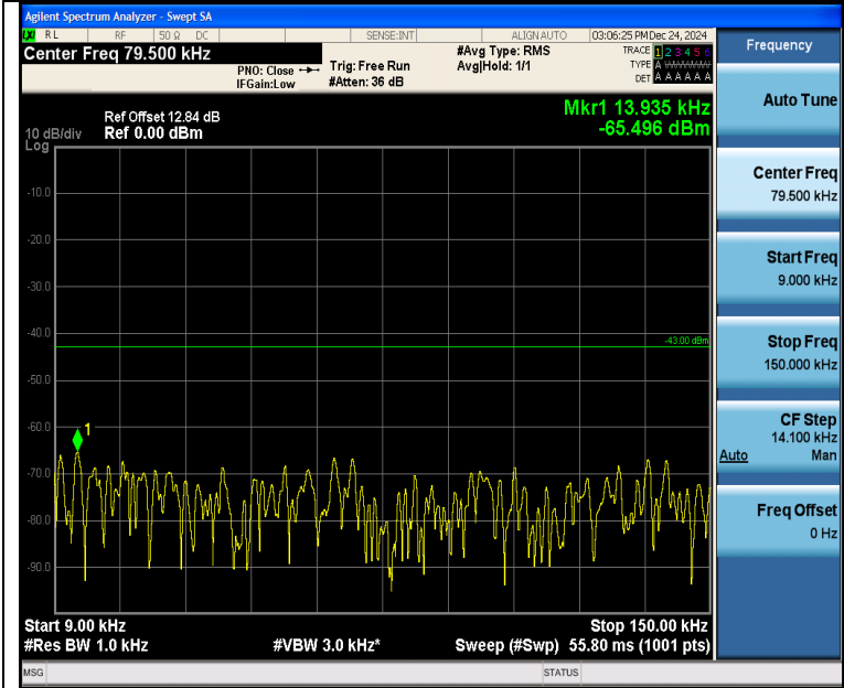
Band4_5MHz_16QAM_19975_1RB#24_0.009~0.15_0.009~0.15
