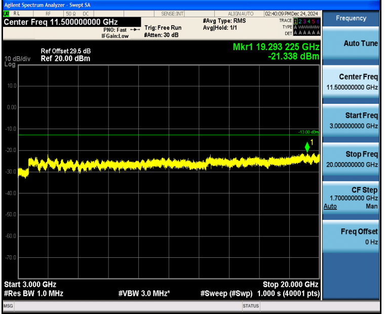
Band4_3MHz_QPSK_20385_1RB#0_3000~20000_3000~20000
