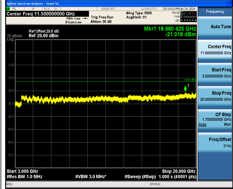
Band4_5MHz_16QAM_20175_1RB#24_3000~20000_3000~20000
