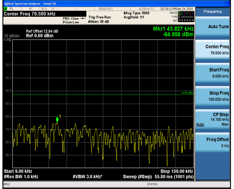
Band4_3MHz_QPSK_20385_1RB#0_0.009~0.15_0.009~0.15
