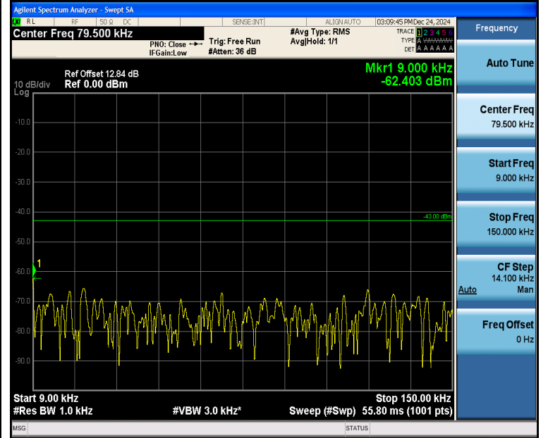
Band4_5MHz_QPSK_20175_1RB#0_0.009~0.15_0.009~0.15
