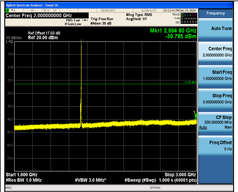
Band4_5MHz_16QAM_20175_1RB#24_1000~3000_1000~3000
