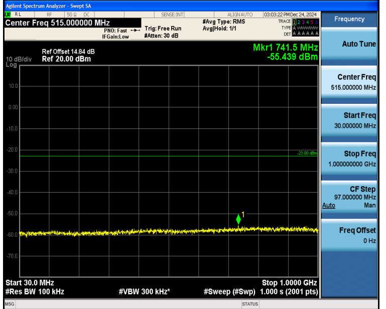
Band4_5MHz_QPSK_19975_1RB#0_30~1000_30~1000
