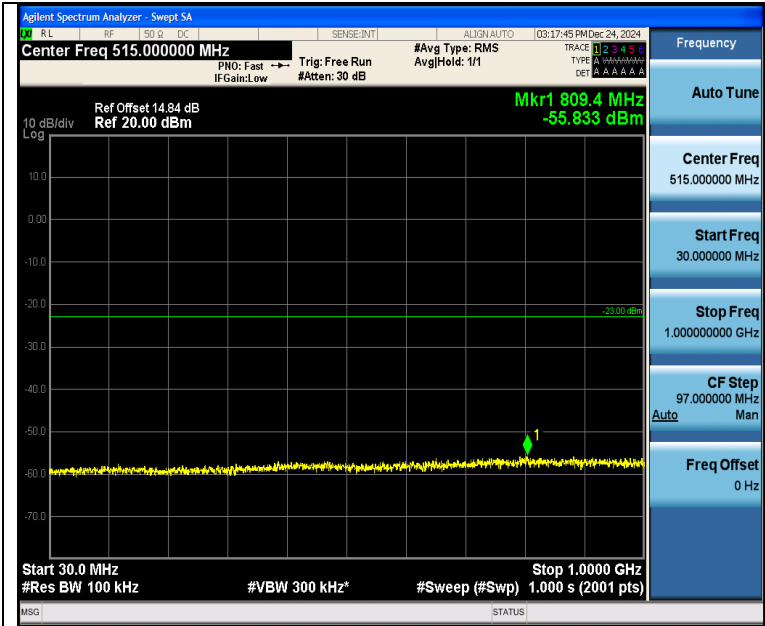
Band4_5MHz_16QAM_20375_1RB#0_30~1000_30~1000
