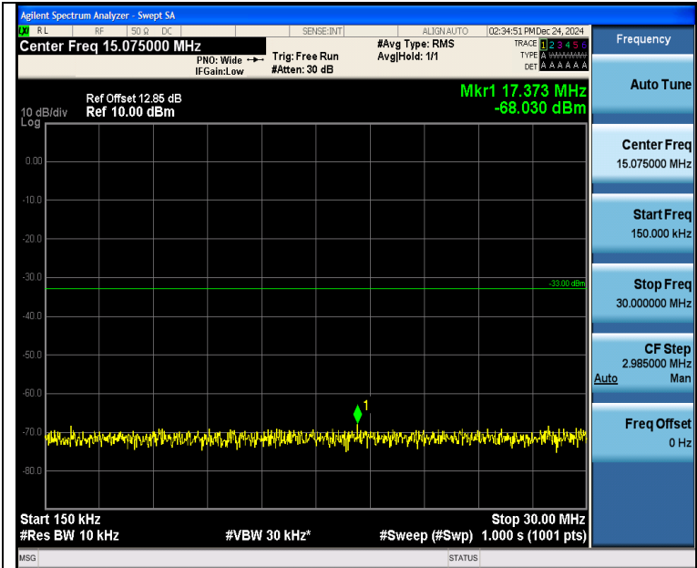
Band4_3MHz_QPSK_20175_1RB#14_0.15~30_0.15~30
