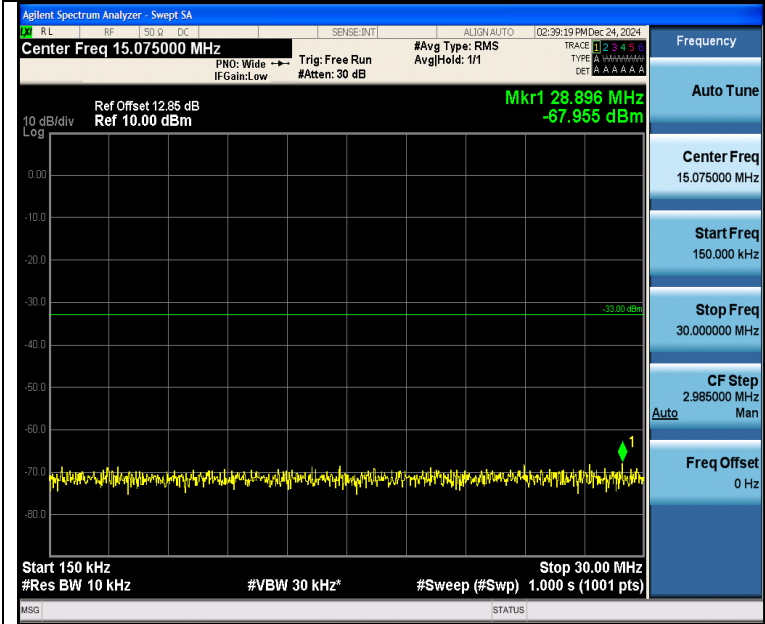
Band4_3MHz_QPSK_20385_1RB#0_0.15~30_0.15~30
