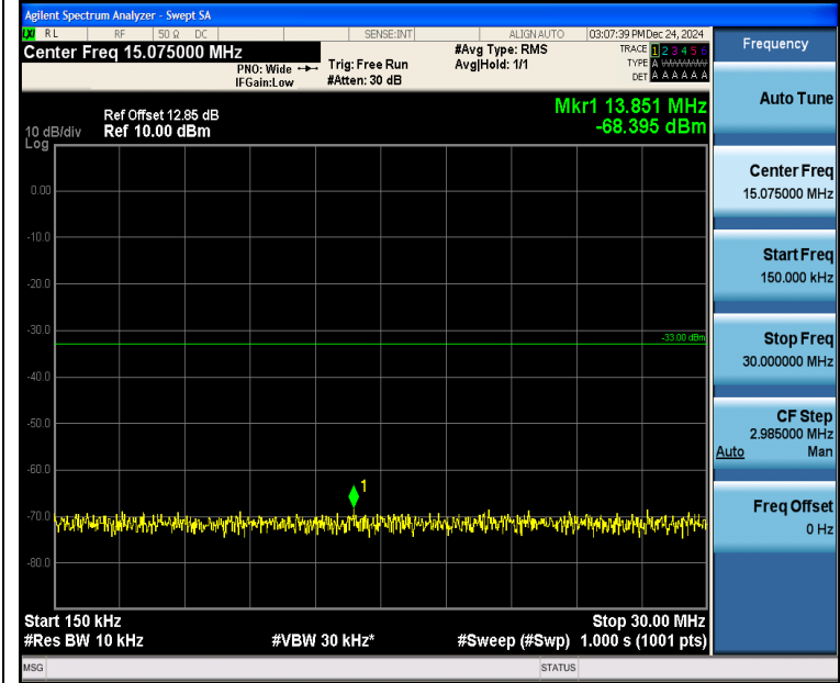
Band4_5MHz_QPSK_19975_25RB#0_0.15~30_0.15~30
