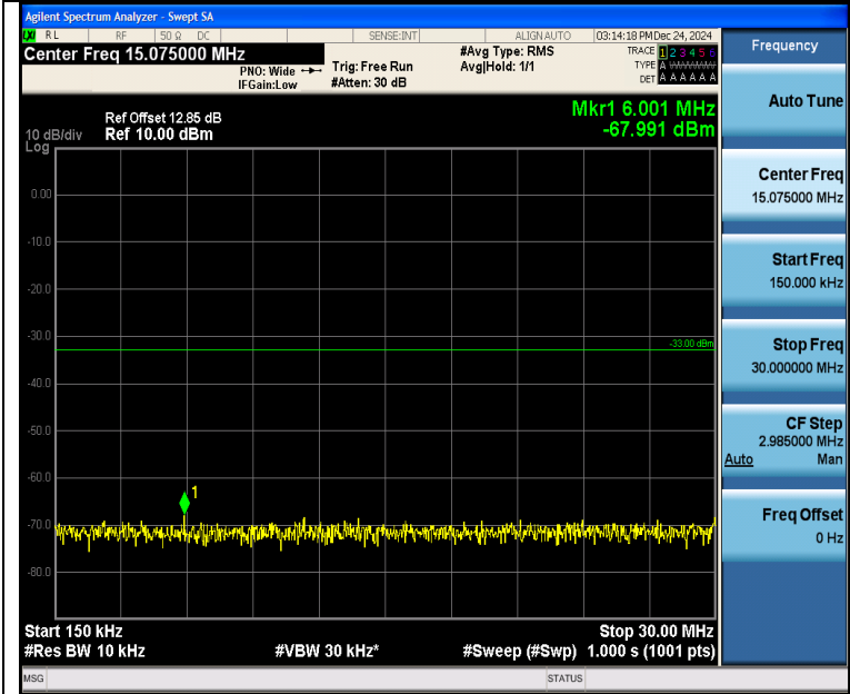
Band4_5MHz_QPSK_20175_25RB#0_0.15~30_0.15~30
