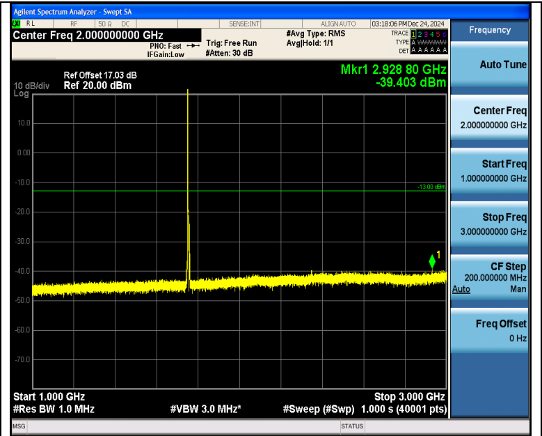
Band4_5MHz_16QAM_20375_1RB#0_1000~3000_1000~3000
