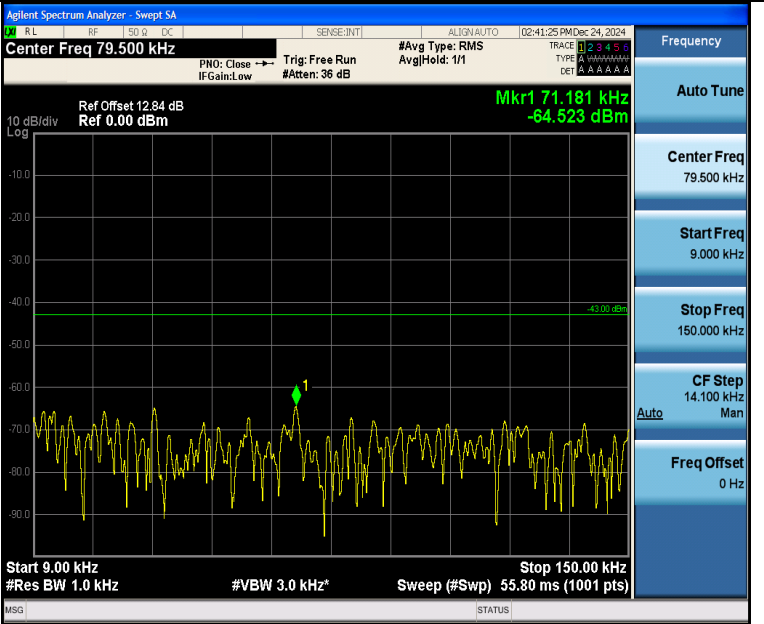
Band4_3MHz_QPSK_20385_1RB#14_0.009~0.15_0.009~0.15
