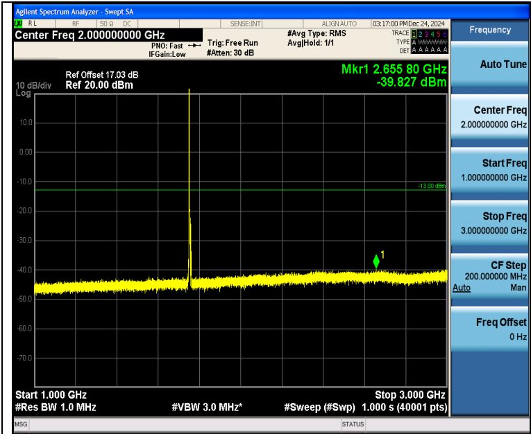
Band4_5MHz_QPSK_20375_1RB#0_1000~3000_1000~3000
