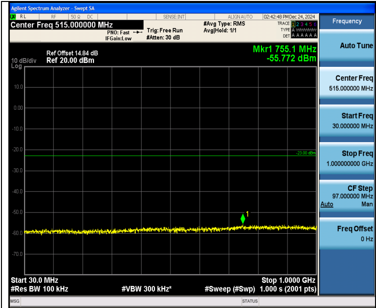
Band4_3MHz_16QAM_20385_1RB#14_30~1000_30~1000
