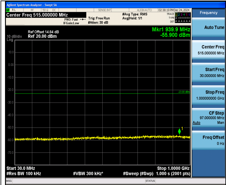
Band4_3MHz_16QAM_20175_15RB#0_30~1000_30~1000
