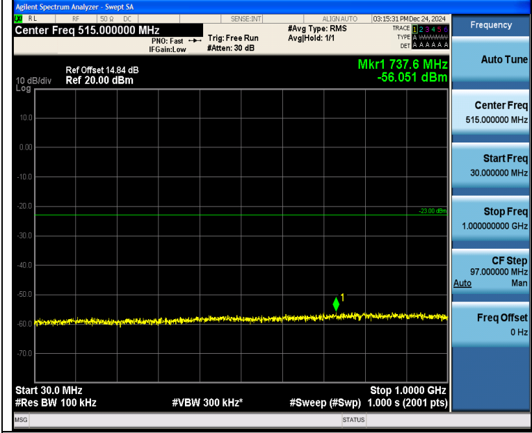
Band4_5MHz_16QAM_20175_25RB#0_30~1000_30~1000
