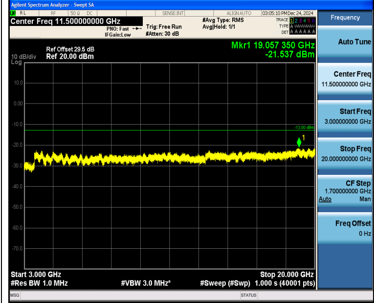
Band4_5MHz_16QAM_19975_1RB#0_3000~20000_3000~20000
