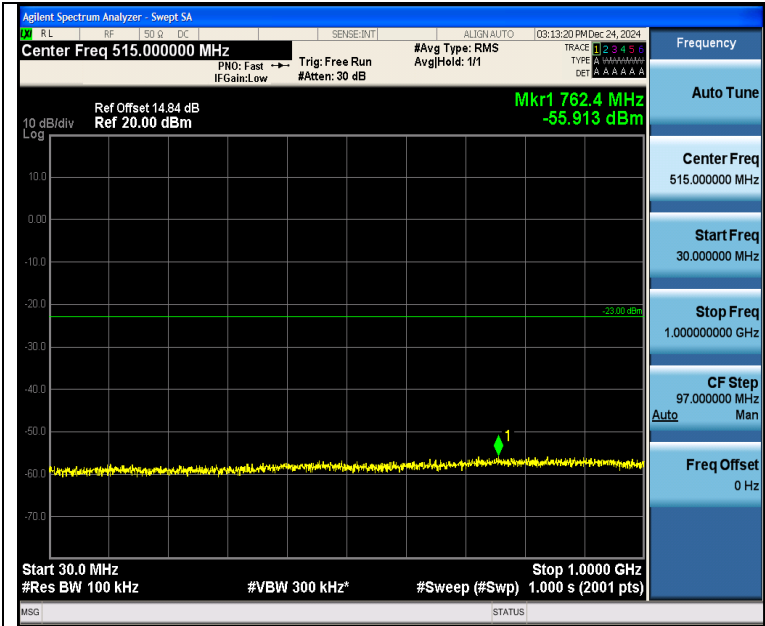
Band4_5MHz_16QAM_20175_1RB#24_30~1000_30~1000
