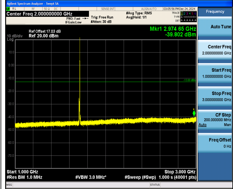
Band4_5MHz_QPSK_19975_1RB#24_1000~3000_1000~3000
