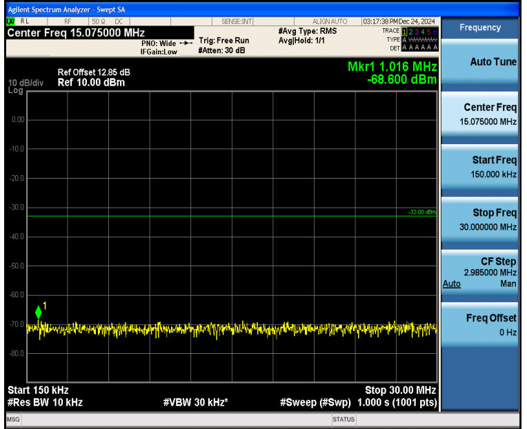
Band4_5MHz_16QAM_20375_1RB#0_0.15~30_0.15~30
