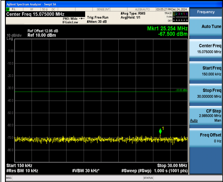
Band4_5MHz_QPSK_19975_1RB#24_0.15~30_0.15~30
