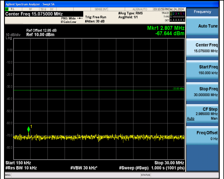
Band4_5MHz_16QAM_20175_1RB#0_0.15~30_0.15~30
