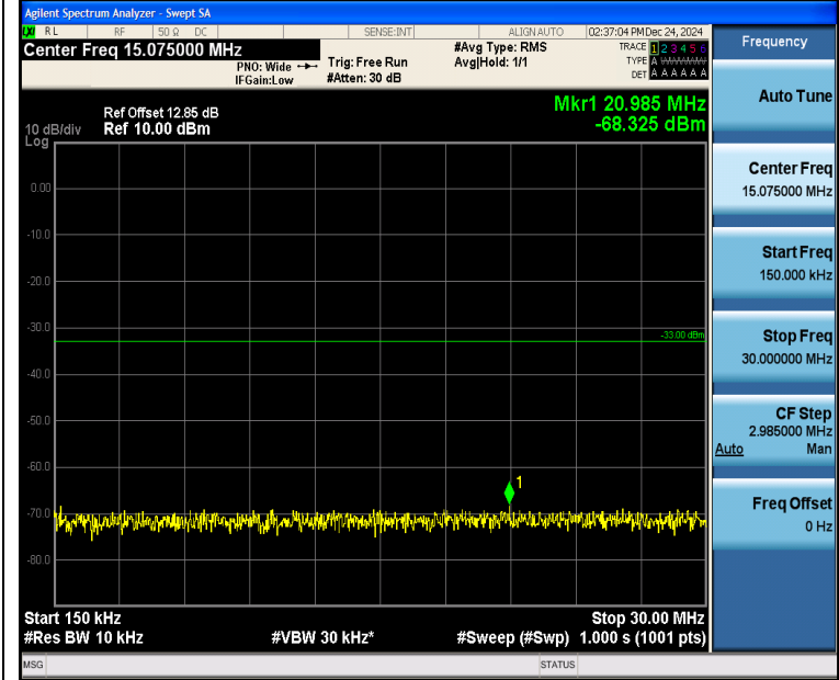
Band4_3MHz_QPSK_20175_15RB#0_0.15~30_0.15~30
