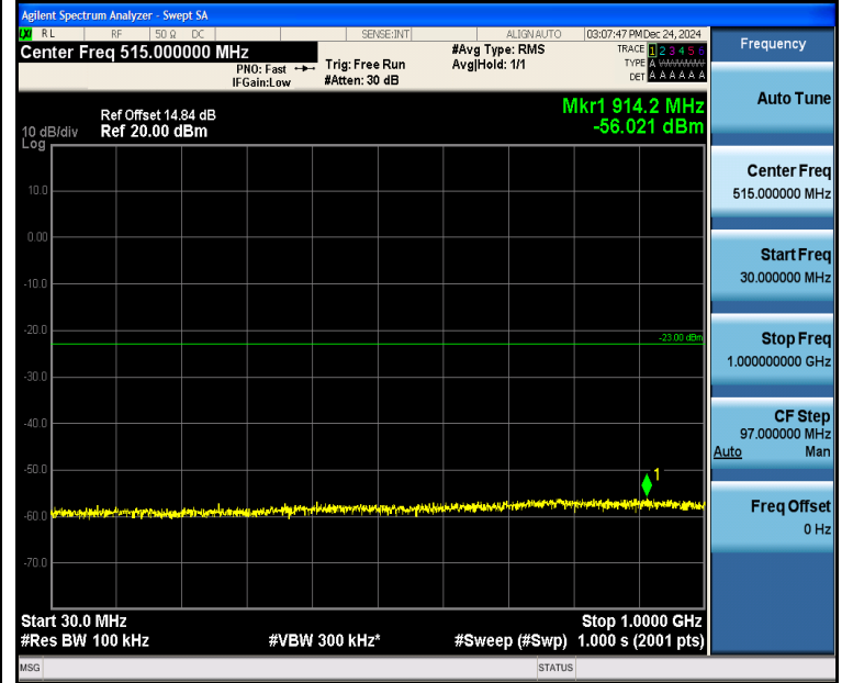
Band4_5MHz_QPSK_19975_25RB#0_30~1000_30~1000
