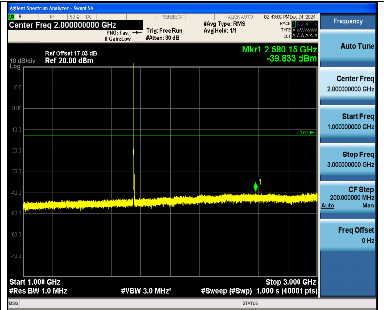
Band4_3MHz_16QAM_20385_1RB#14_1000~3000_1000~3000
