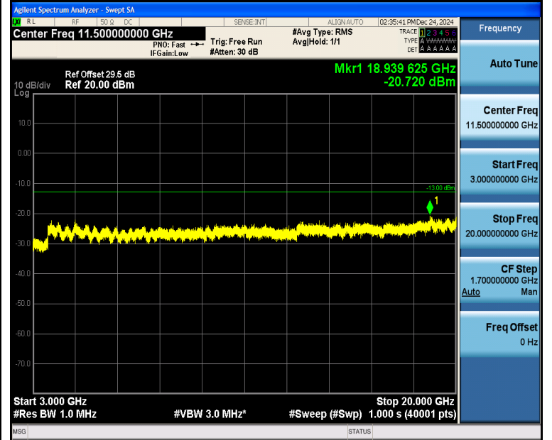
Band4_3MHz_QPSK_20175_1RB#14_3000~20000_3000~20000
