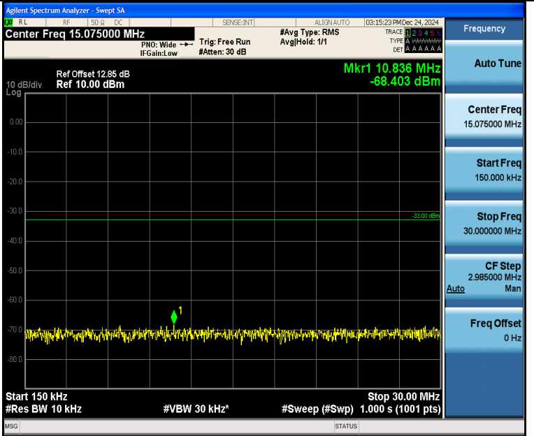
Band4_5MHz_16QAM_20175_25RB#0_0.15~30_0.15~30
