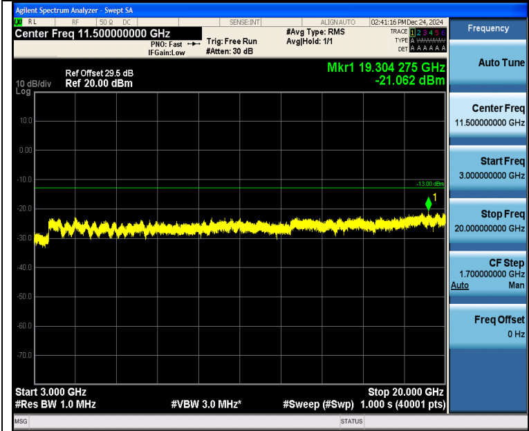
Band4_3MHz_16QAM_20385_1RB#0_3000~20000_3000~20000
