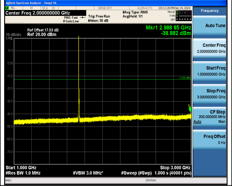
Band4_5MHz_16QAM_20175_1RB#0_1000~3000_1000~3000
