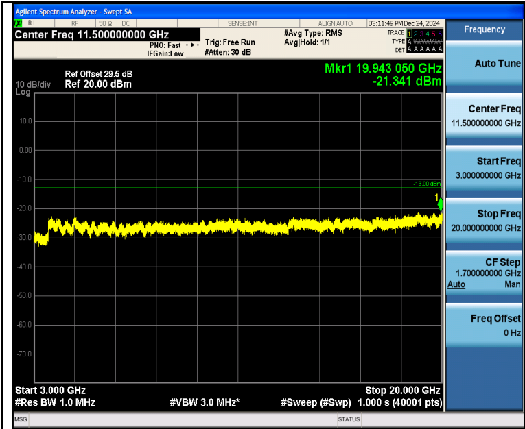
Band4_5MHz_16QAM_20175_1RB#0_3000~20000_3000~20000
