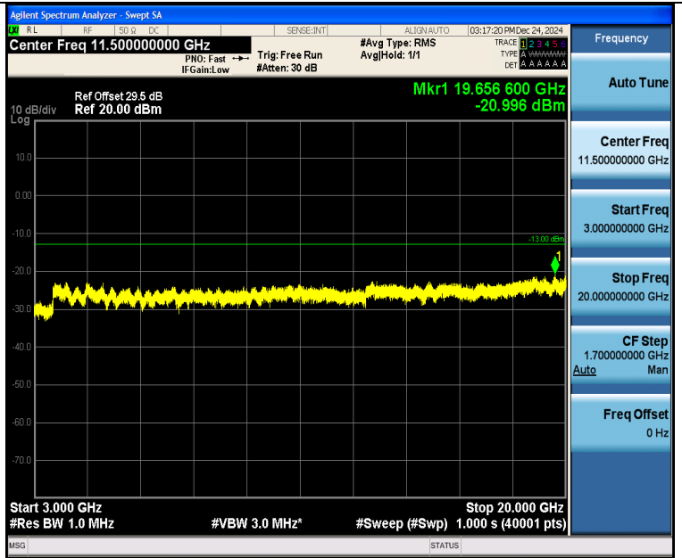
Band4_5MHz_QPSK_20375_1RB#0_3000~20000_3000~20000
