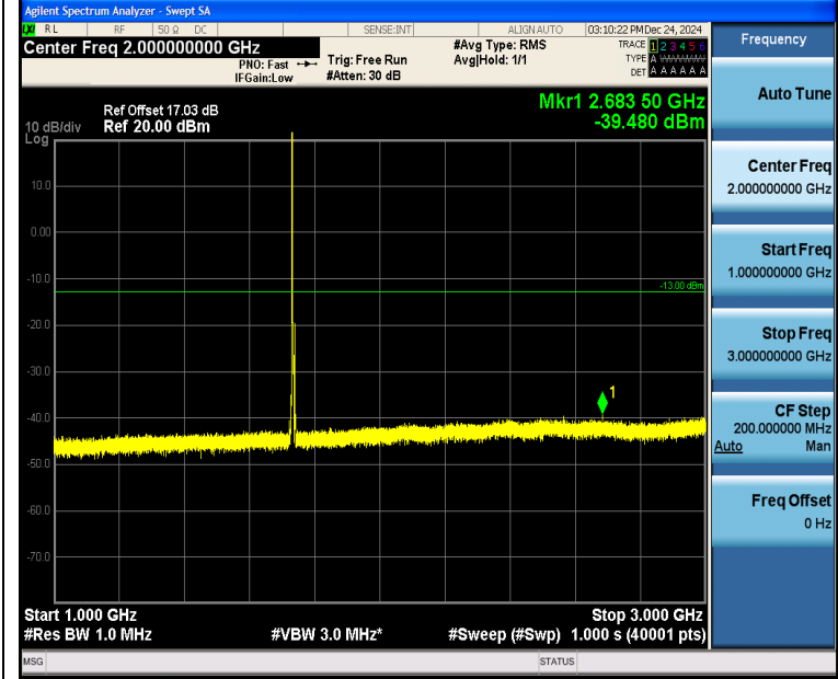
Band4_5MHz_QPSK_20175_1RB#0_1000~3000_1000~3000
