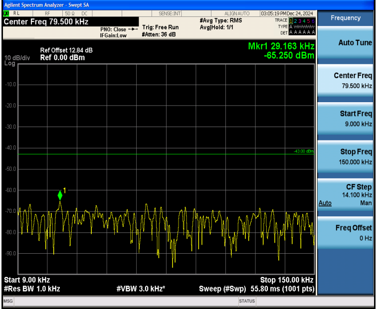
Band4_5MHz_QPSK_19975_1RB#24_0.009~0.15_0.009~0.15
