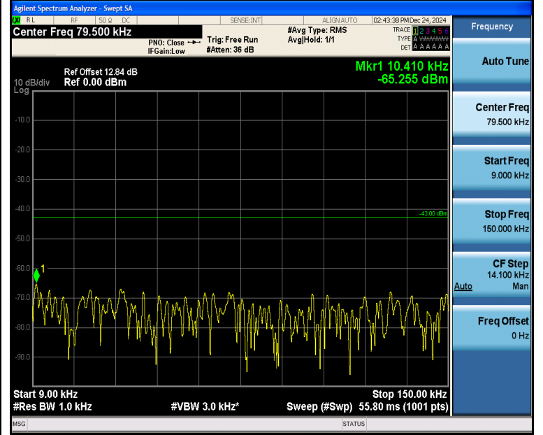
Band4_3MHz_QPSK_20385_15RB#0_0.009~0.15_0.009~0.15
