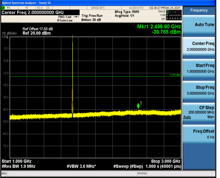
Band4_3MHz_16QAM_20175_1RB#14_1000~3000_1000~3000
