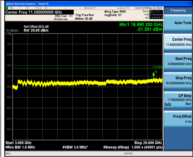
Band4_5MHz_16QAM_19975_1RB#24_3000~20000_3000~20000
