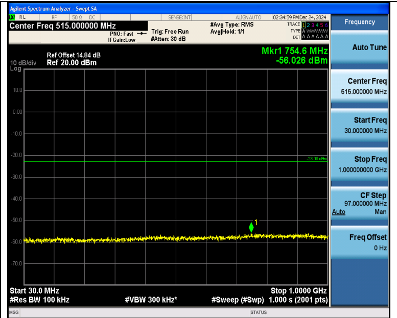
Band4_3MHz_QPSK_20175_1RB#14_30~1000_30~1000
