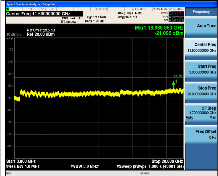
Band4_3MHz_16QAM_20385_15RB#0_3000~20000_3000~20000
