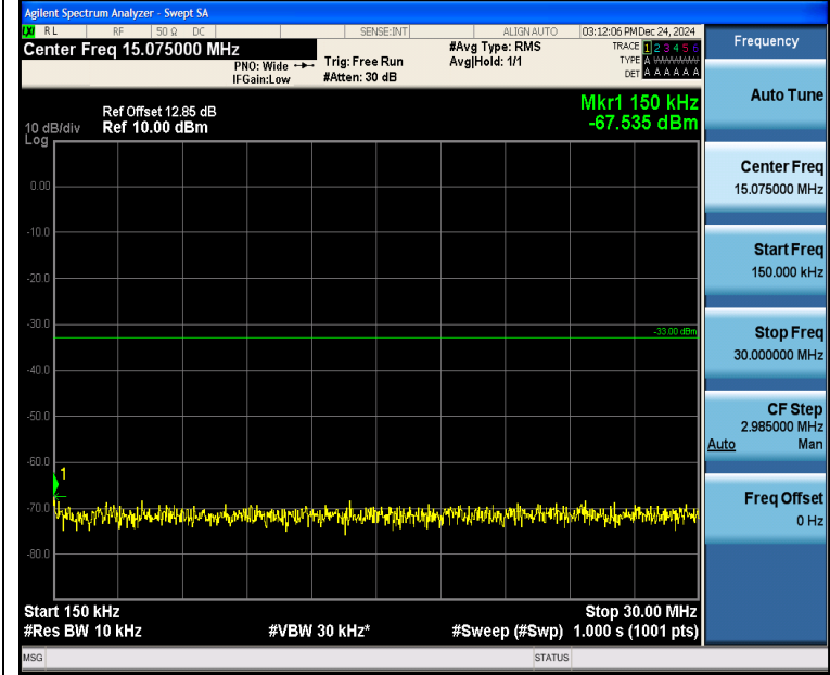
Band4_5MHz_QPSK_20175_1RB#24_0.15~30_0.15~30
