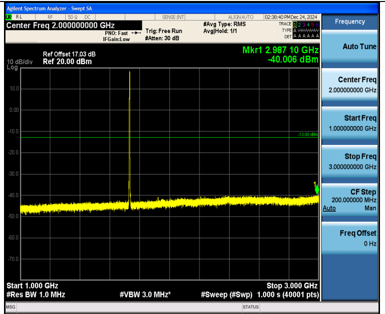
Band4_3MHz_16QAM_20175_15RB#0_1000~3000_1000~3000
