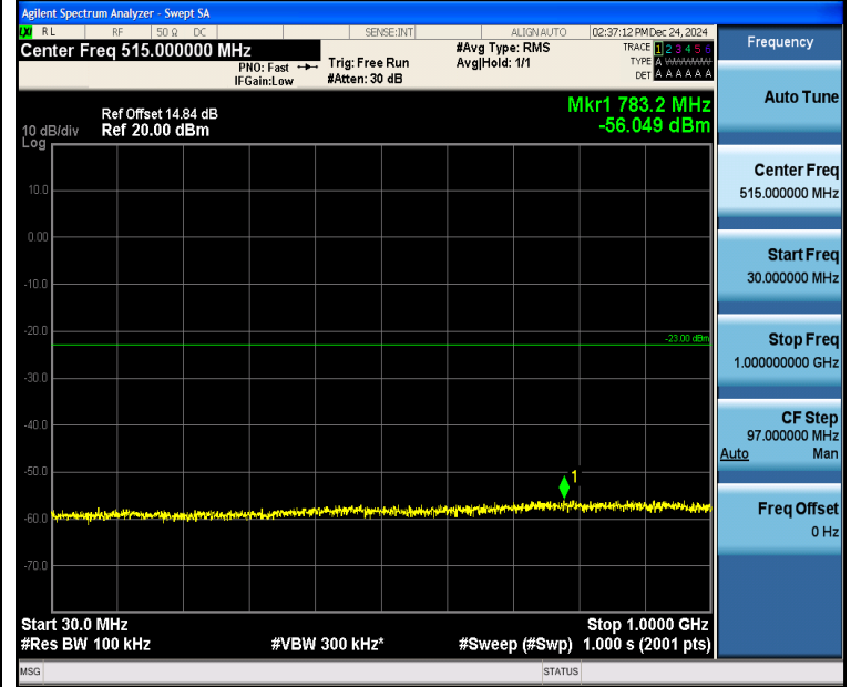
Band4_3MHz_QPSK_20175_15RB#0_30~1000_30~1000
