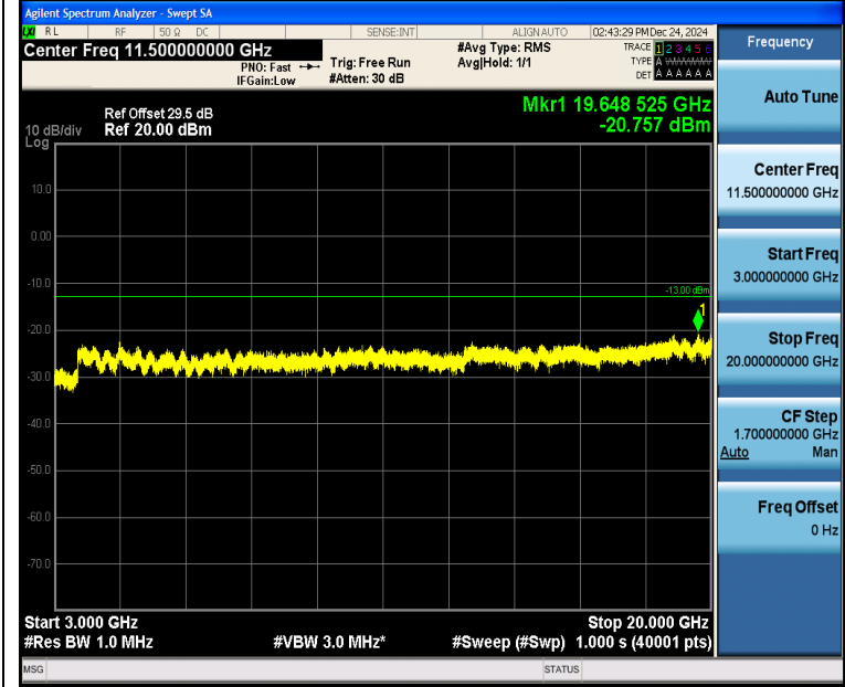
Band4_3MHz_16QAM_20385_1RB#14_3000~20000_3000~20000
