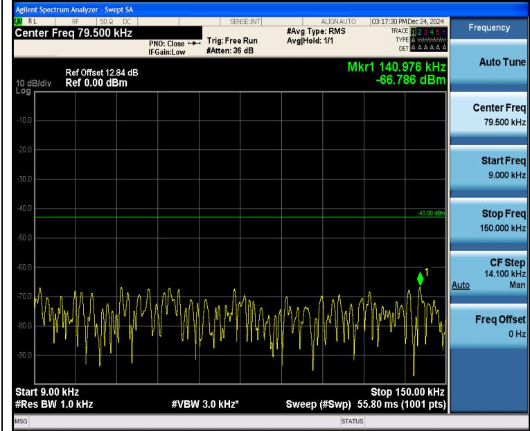
Band4_5MHz_16QAM_20375_1RB#0_0.009~0.15_0.009~0.15
