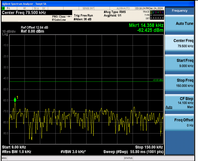
Band4_5MHz_QPSK_20375_1RB#0_0.009~0.15_0.009~0.15
