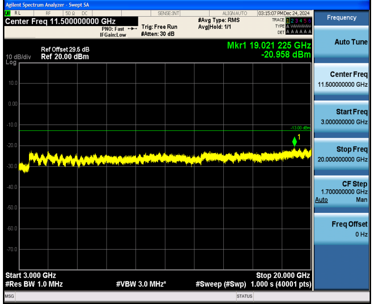
Band4_5MHz_QPSK_20175_25RB#0_3000~20000_3000~20000
