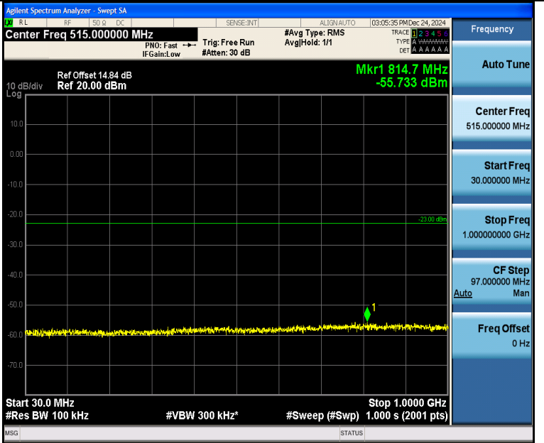
Band4_5MHz_QPSK_19975_1RB#24_30~1000_30~1000
