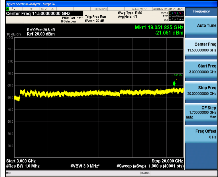
Band4_5MHz_16QAM_20375_1RB#0_3000~20000_3000~20000
