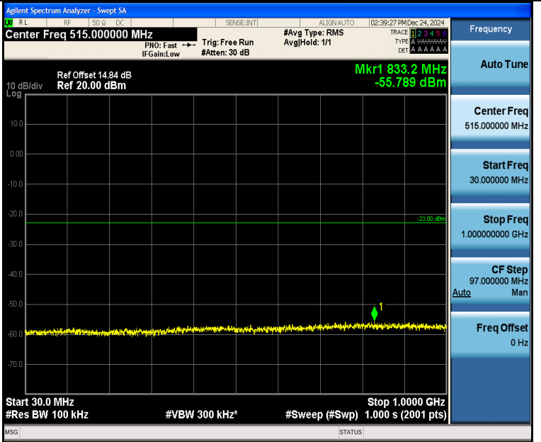
Band4_3MHz_QPSK_20385_1RB#0_30~1000_30~1000
