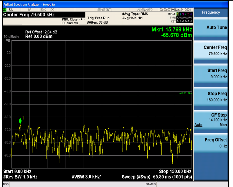
Band4_5MHz_QPSK_19975_1RB#0_0.009~0.15_0.009~0.15
