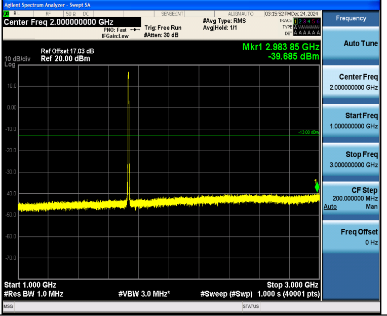
Band4_5MHz_16QAM_20175_25RB#0_1000~3000_1000~3000
