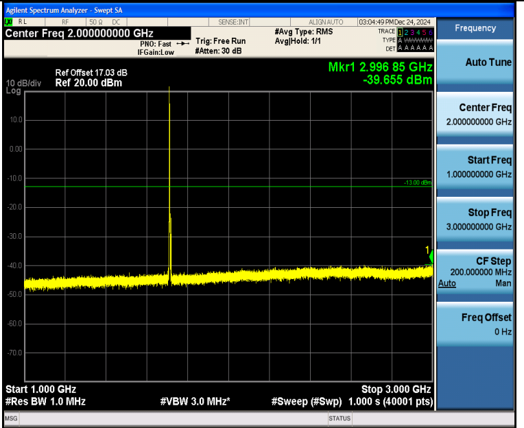
Band4_5MHz_16QAM_19975_1RB#0_1000~3000_1000~3000
