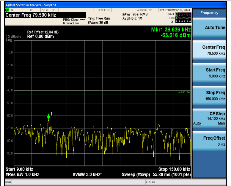
Band4_5MHz_QPSK_20175_1RB#24_0.009~0.15_0.009~0.15
