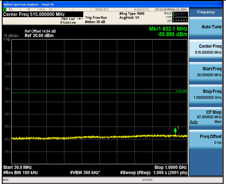
Band4_5MHz_QPSK_20175_25RB#0_30~1000_30~1000
