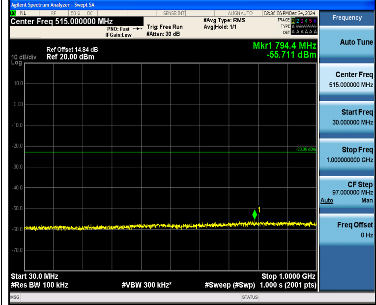
Band4_3MHz_16QAM_20175_1RB#14_30~1000_30~1000
