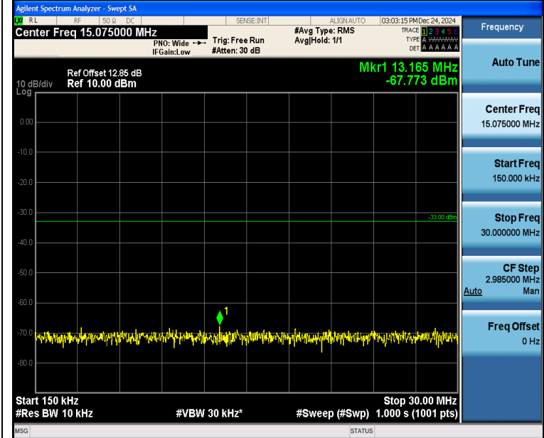
Band4_5MHz_QPSK_19975_1RB#0_0.15~30_0.15~30
