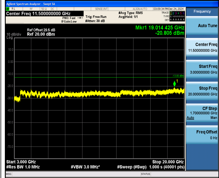
Band4_5MHz_16QAM_19975_25RB#0_3000~20000_3000~20000
