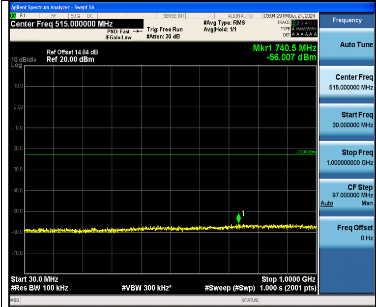
Band4_5MHz_16QAM_19975_1RB#0_30~1000_30~1000
