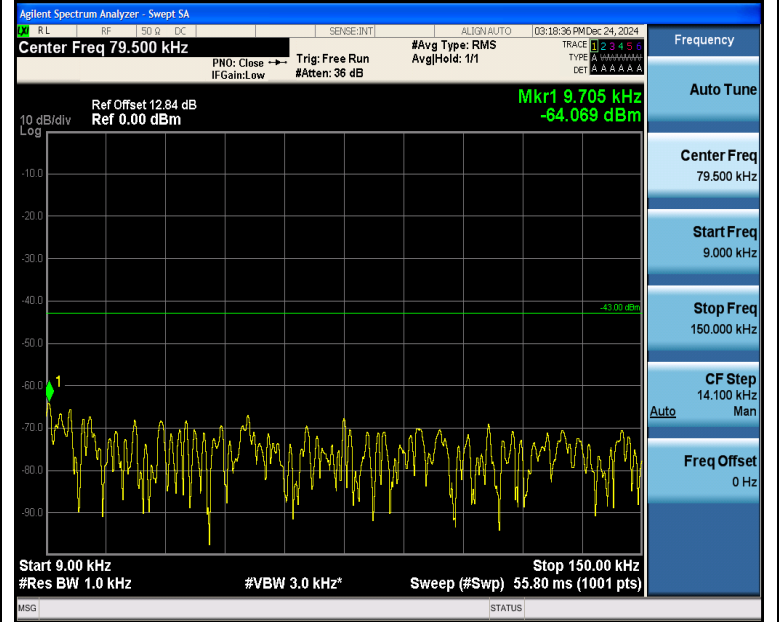
Band4_5MHz_QPSK_20375_1RB#24_0.009~0.15_0.009~0.15
