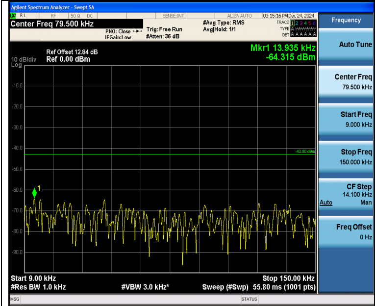
Band4_5MHz_16QAM_20175_25RB#0_0.009~0.15_0.009~0.15
