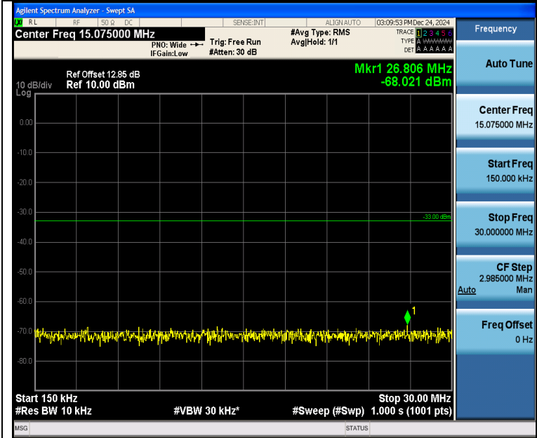
Band4_5MHz_QPSK_20175_1RB#0_0.15~30_0.15~30
