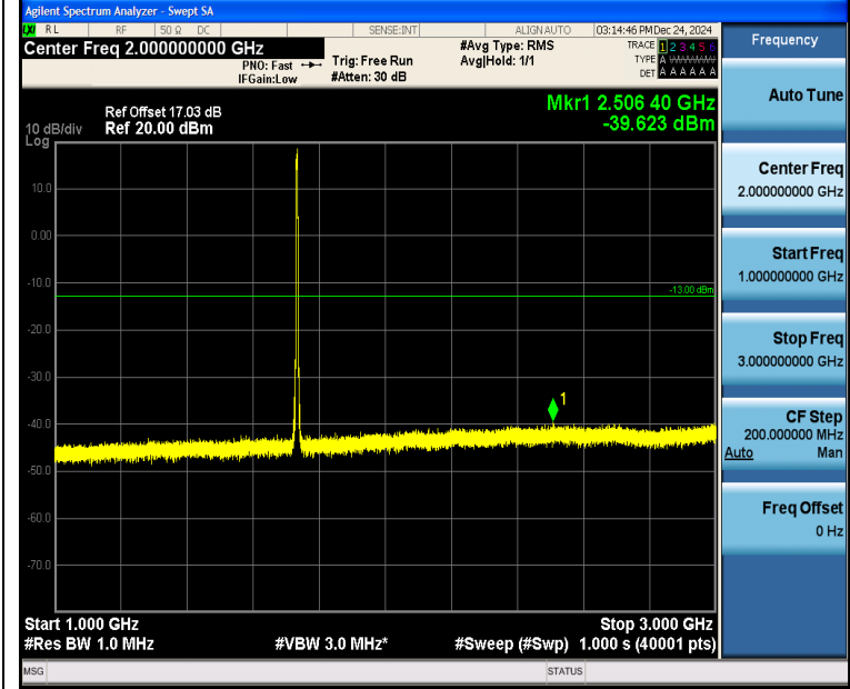
Band4_5MHz_QPSK_20175_25RB#0_1000~3000_1000~3000
