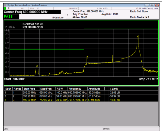
Band12-10MHz-QPSK-23130-1RB#0
