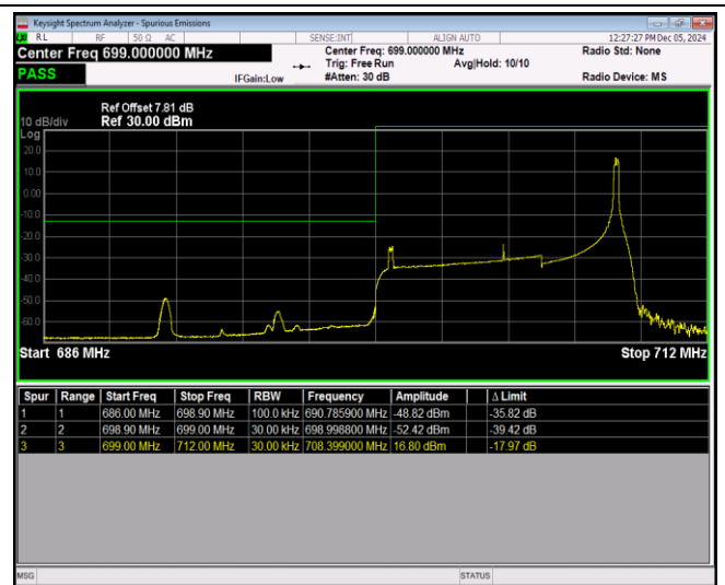
Band12-10MHz-16QAM-23130-1RB#0
