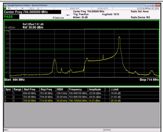
Band17-5MHz-QPSK-23825-1RB#0
