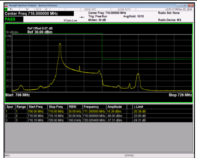
Band17-5MHz-QPSK-23825-25RB#0
