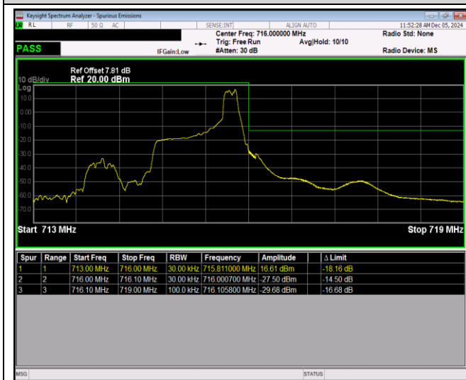
Band12-10MHz-QPSK-23060-1RB#0
