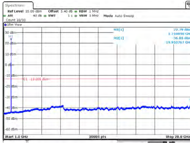
Band4_20MHz_16QAM_20050_1RB#0
