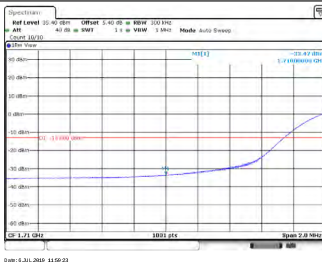
Band4_20MHz_16QAM_20300_1RB#99
