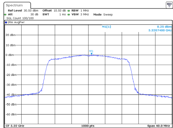
802.11ax20_5320MHz_RU_Full_Chain 2
