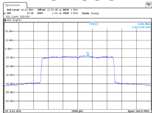
802.11ax80_5610MHz_RU_Full_Chain 1
