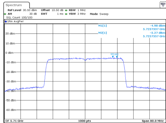
802.11ax40_5710MHz_RU_Full_Chain 1
