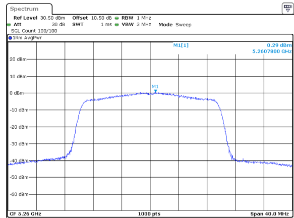
802.11ax20_5260MHz_RU_Full_Chain 2
