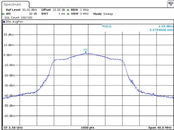
802.11a_5580MHz_Chain 1
