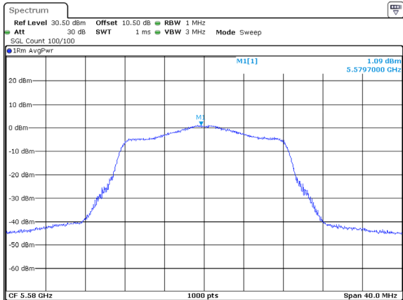
802.11a_5580MHz_Chain 2
