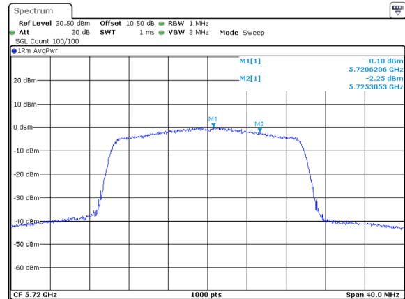
802.11ax20_5720MHz_RU_Full_Chain 2
