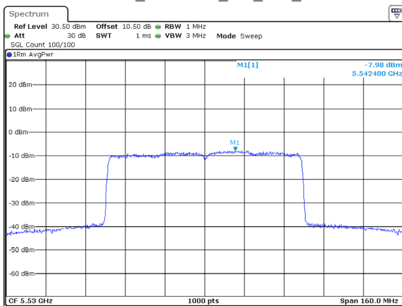
802.11ax80_5530MHz_RU_Full_Chain 1
