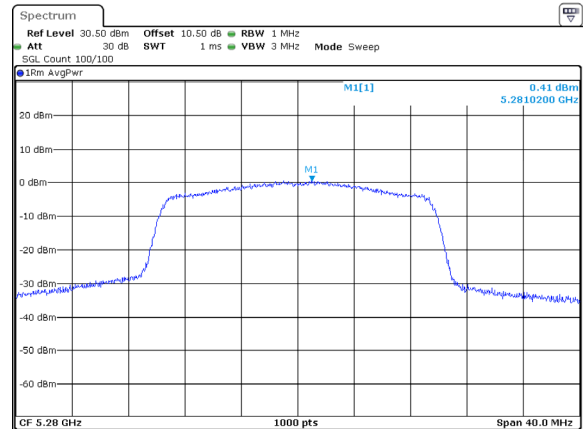
802.11ax20_5280MHz_RU_Full_Chain 1
