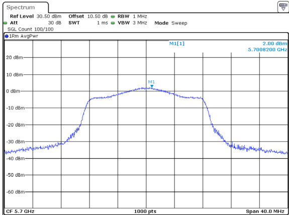
802.11a_5700MHz_Chain 1
