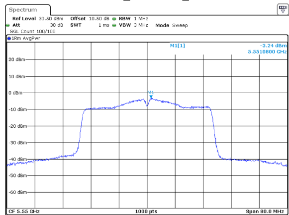
802.11ac40_5550MHz_Chain 1
