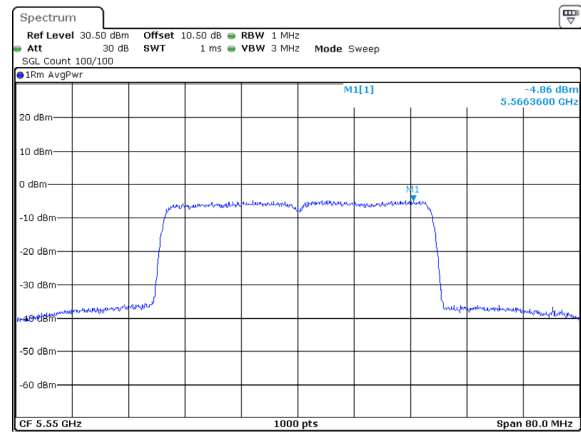
802.11ax40_5550MHz_RU_Full_Chain 1
