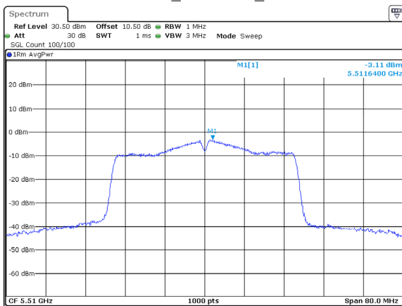
802.11ac40_5510MHz_Chain 1
