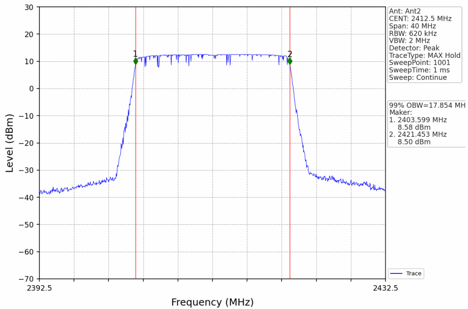
20M_LCH_2412.5MHz_Ant2_NTNV
