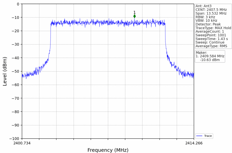
10M_LCH_2407.5MHz_Ant3_NTNV
