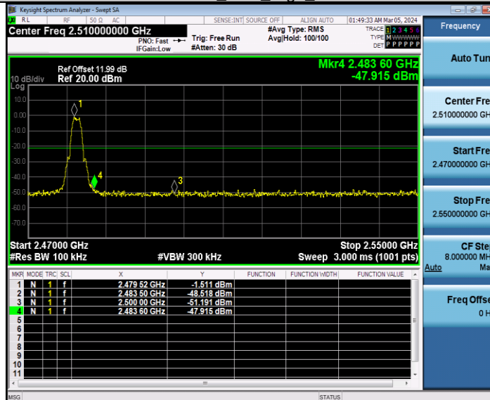
ZIGBEE_Ant1_High_2480
